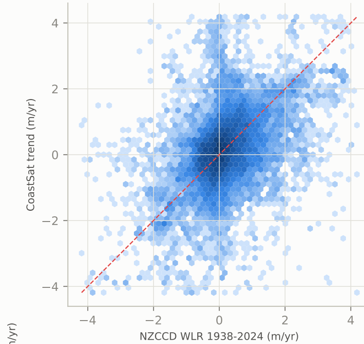
Same transect, different periods \rho=0.41 , sign agreement 64%, n=22,509
