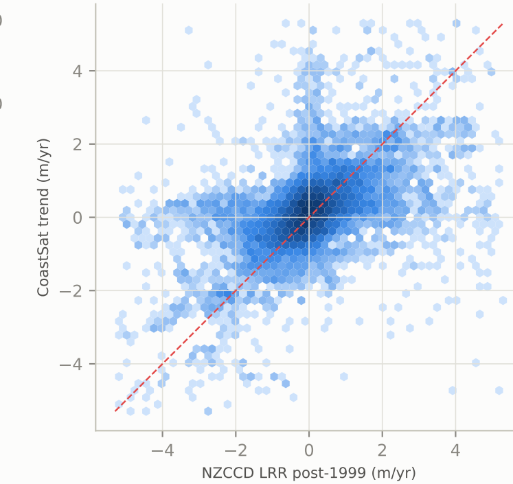
Same transect, same period \rho=0.52 , sign agreement 68%, n=12,312
