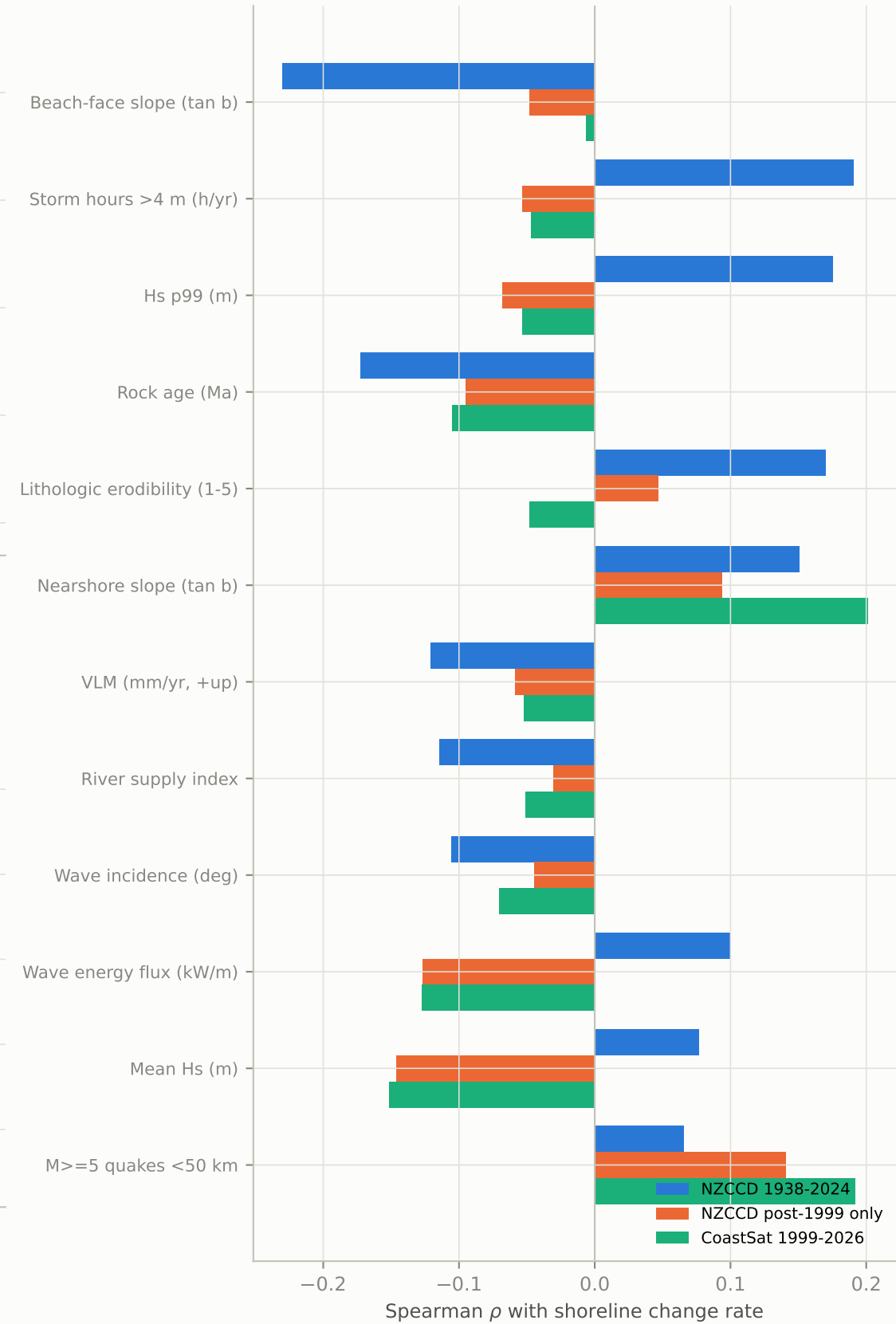
Driver correlations depend on record length, not method (same transects, site-block bootstrap)
