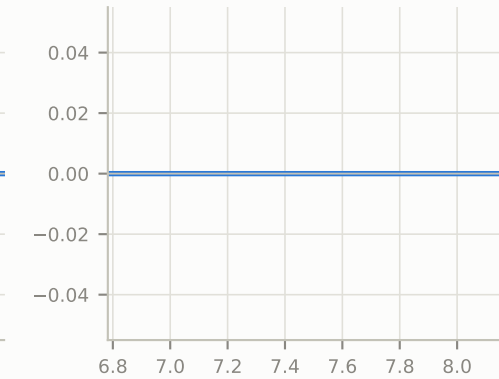
Seismic shaking index
