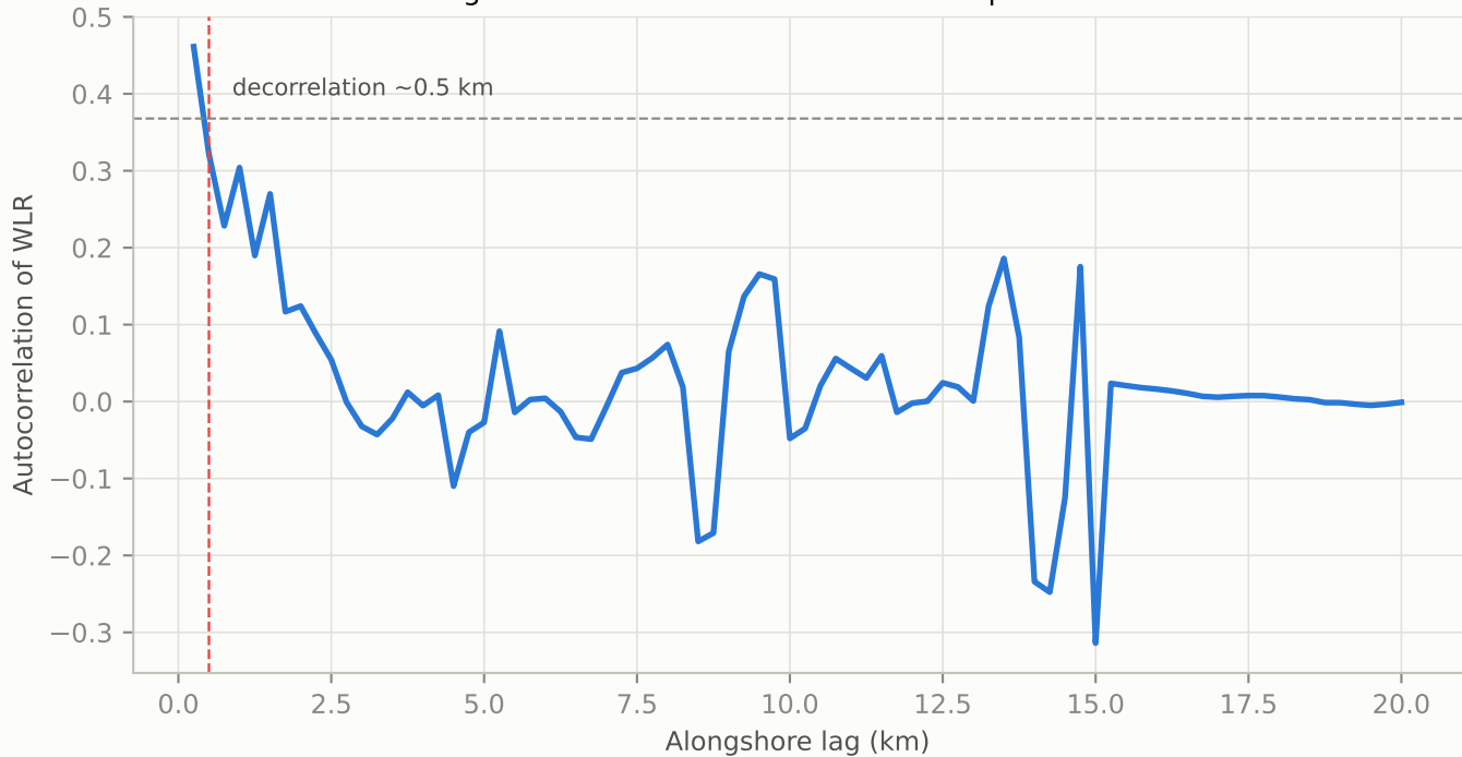
Alongshore autocorrelation and bootstrap block choice
