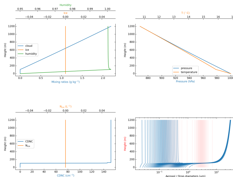
Figure 3: With initial RH = 0.95, saturation is reached after only a small amount of lifting and the cloud is much deeper.
