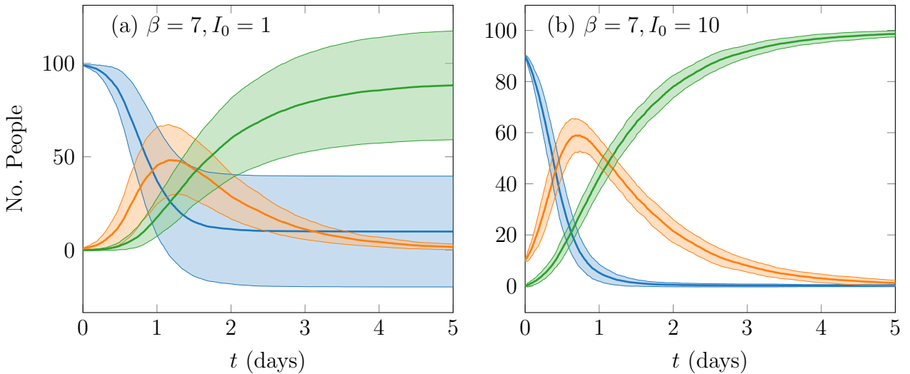
Figure 3: Ensemble averaged SIR model with \beta/N people infected per day per infected person per susceptible person and \gamma = 1 people recovered per day per infected person, where N = 100 is the total population. I_0 people are infected at t = 0 and the rest of the population is susceptible. (a): \beta = 7 , I_0 = 1 ; (b): \beta = 7 , I_0 = 10 . Figures produced by M. G. Hauge Evans.
