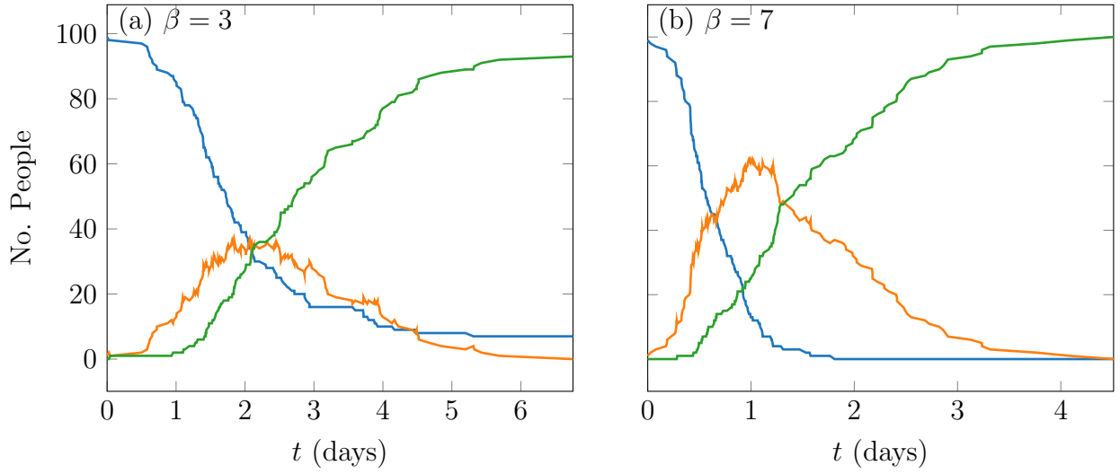
Figure 2: SIR model with \beta/N people infected per day per infected person per susceptible person and \gamma people recovered per day per infected person, where N is the total population. (a): \beta = 3 , \gamma = 1 ; (b): \beta = 7 , \gamma = 1 . Figures produced by M. G. Hauge Evans.
