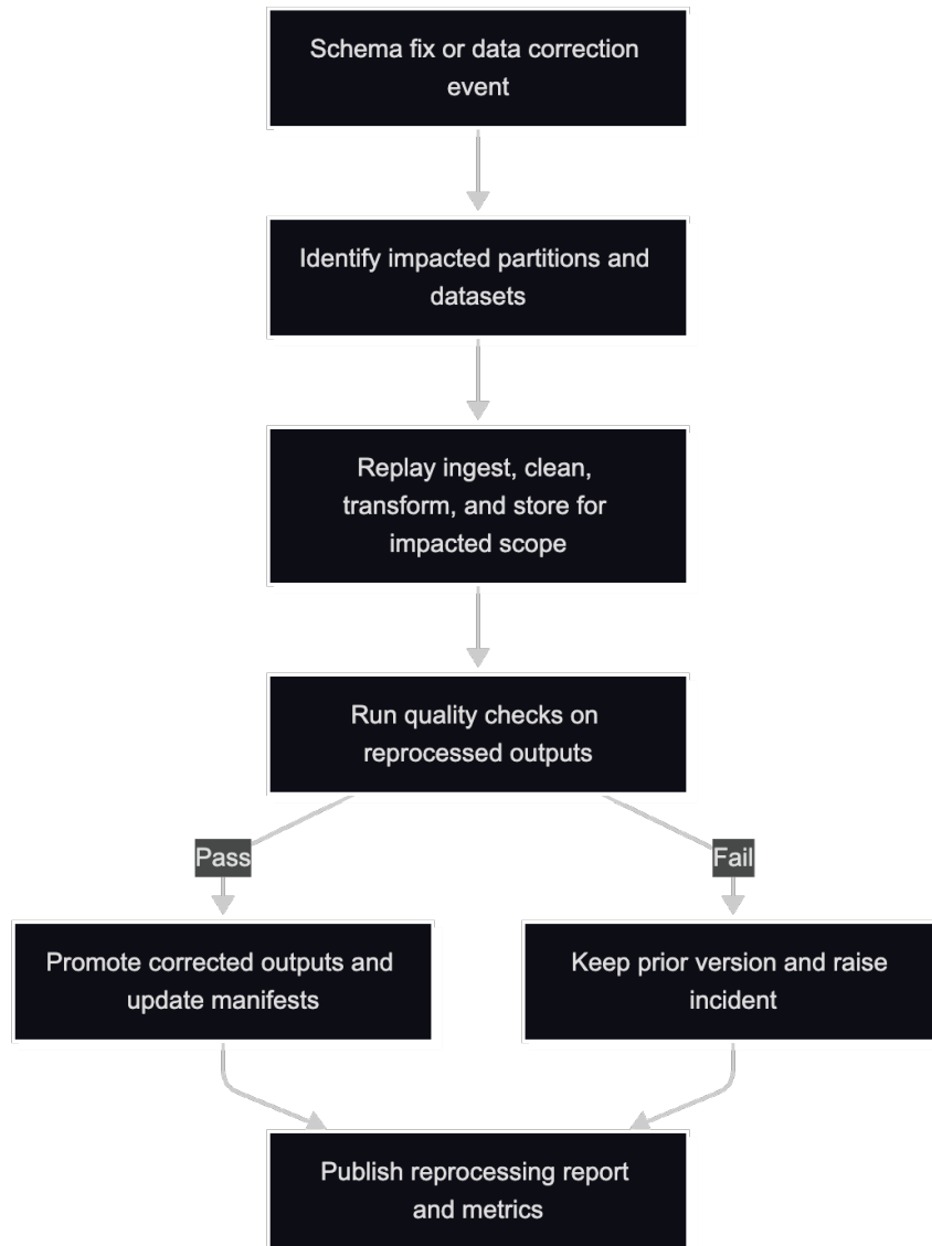
Figure 5: Offline targeted reprocessing workflow (OfflineDatasetWorkflow).
