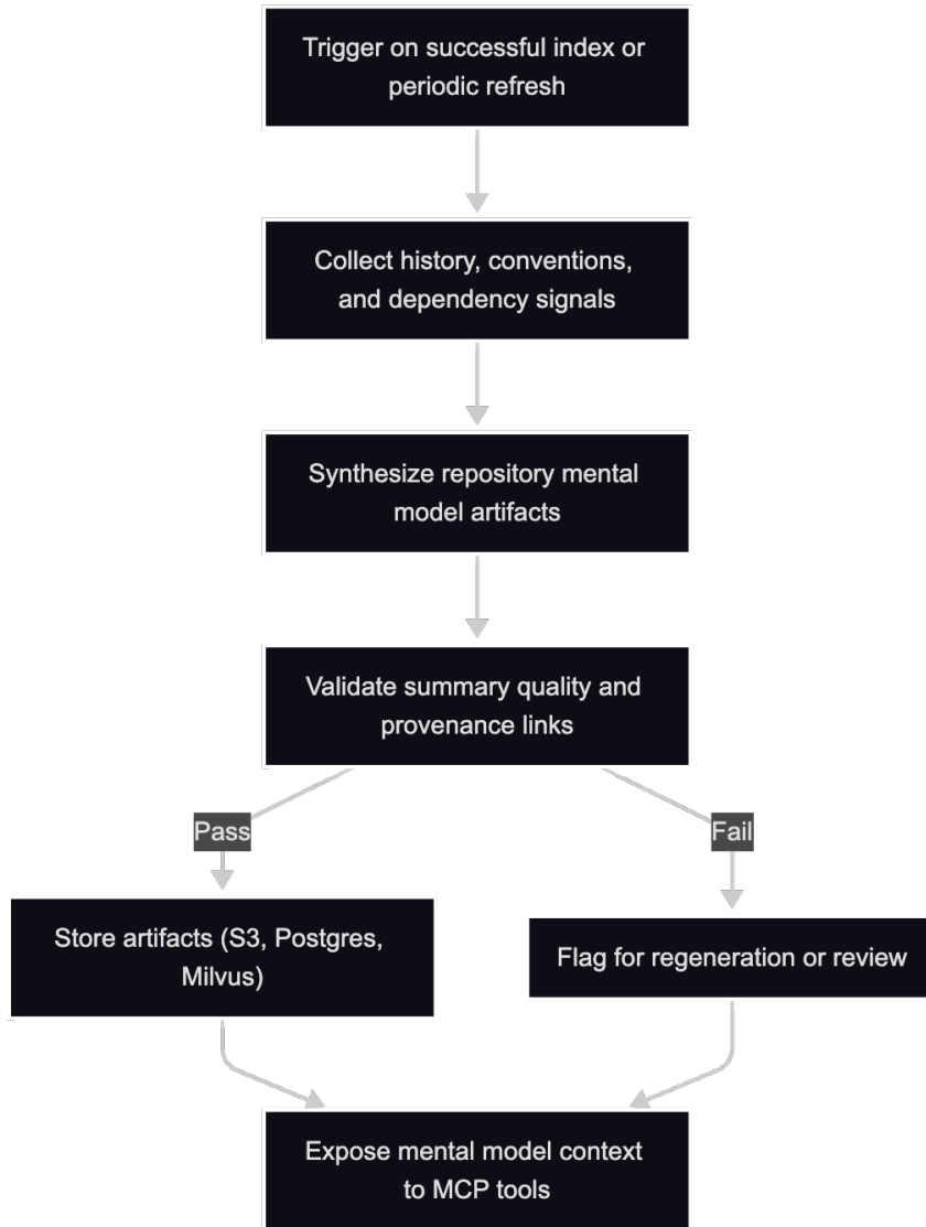
Figure 6: Mental model workflow (MentalModelWorkflow).
