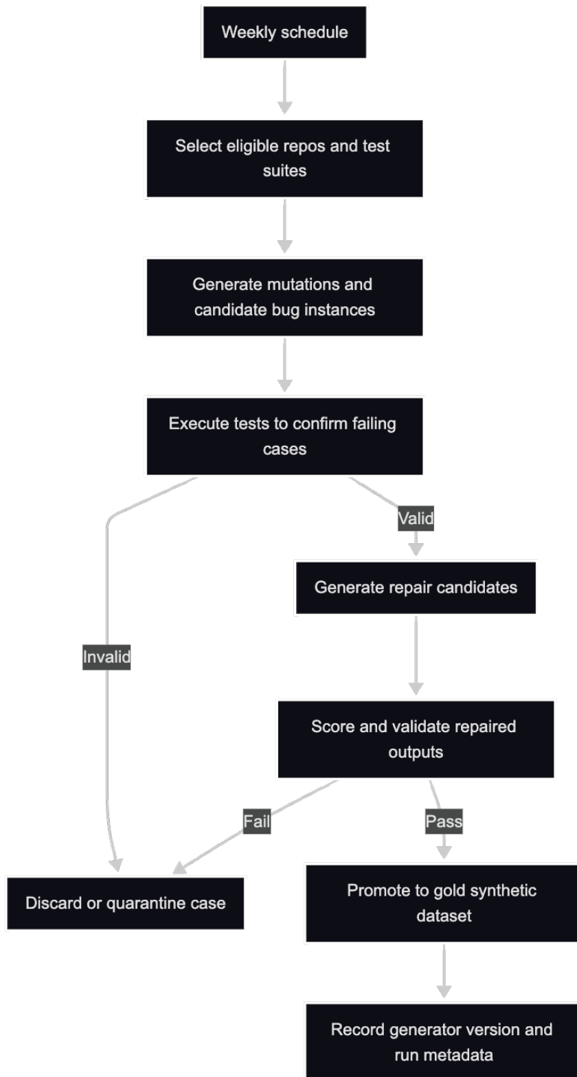
Figure 4: Offline synthetic refresh workflow (OfflineDatasetWorkflow).
