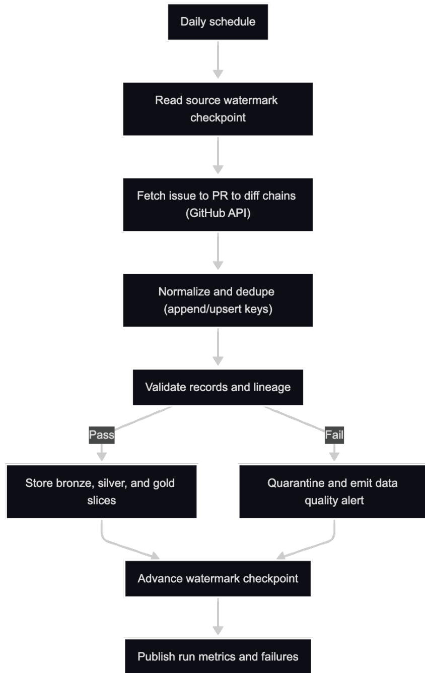
Figure 3: Offline rolling scraped workflow (OfflineDatasetWorkflow).
