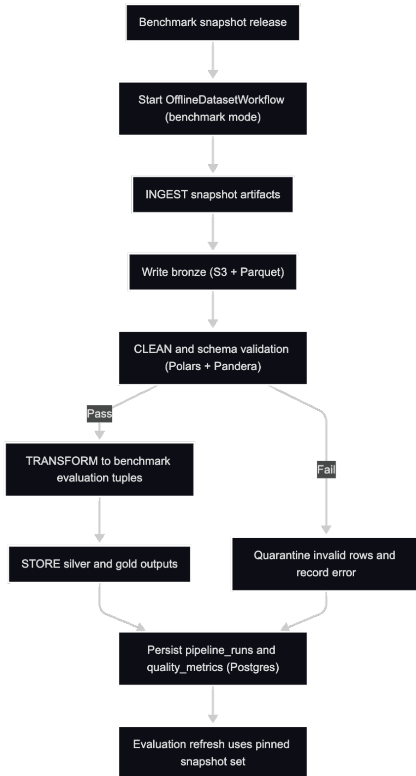
Figure 2: Offline benchmark snapshot workflow (OfflineDatasetWorkflow).
