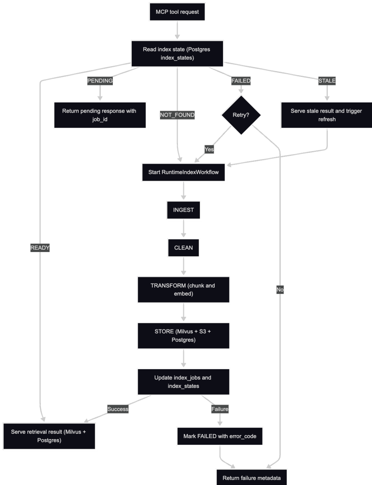
Figure 1: Runtime indexing workflow (RuntimeIndexWorkflow).
