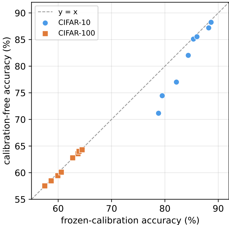
Calibration-free vs frozen (16 cells)
