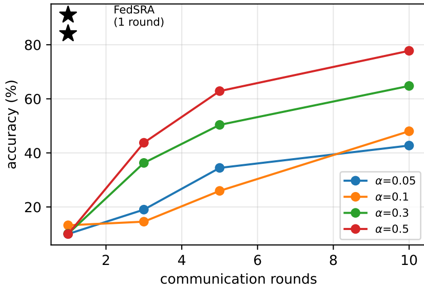
cifar10: multi-round ETF vs FedSRA one-shot
