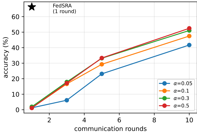
cifar100: multi-round ETF vs FedSRA one-shot
