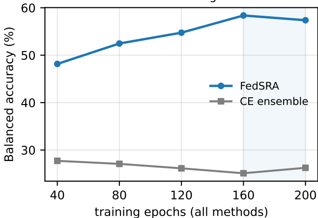
Fed-ISIC convergence
