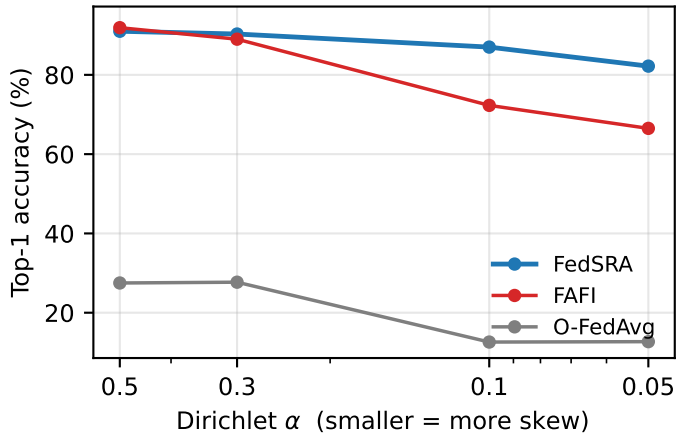
PathMNIST
