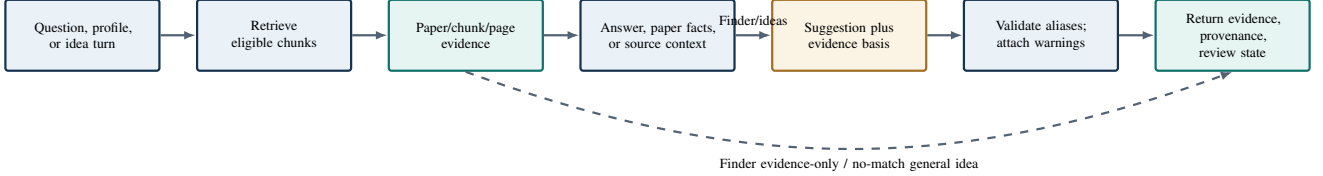
Fig. 2. Ask, structured Finder, and conversational Idea Generator evidence flow.
