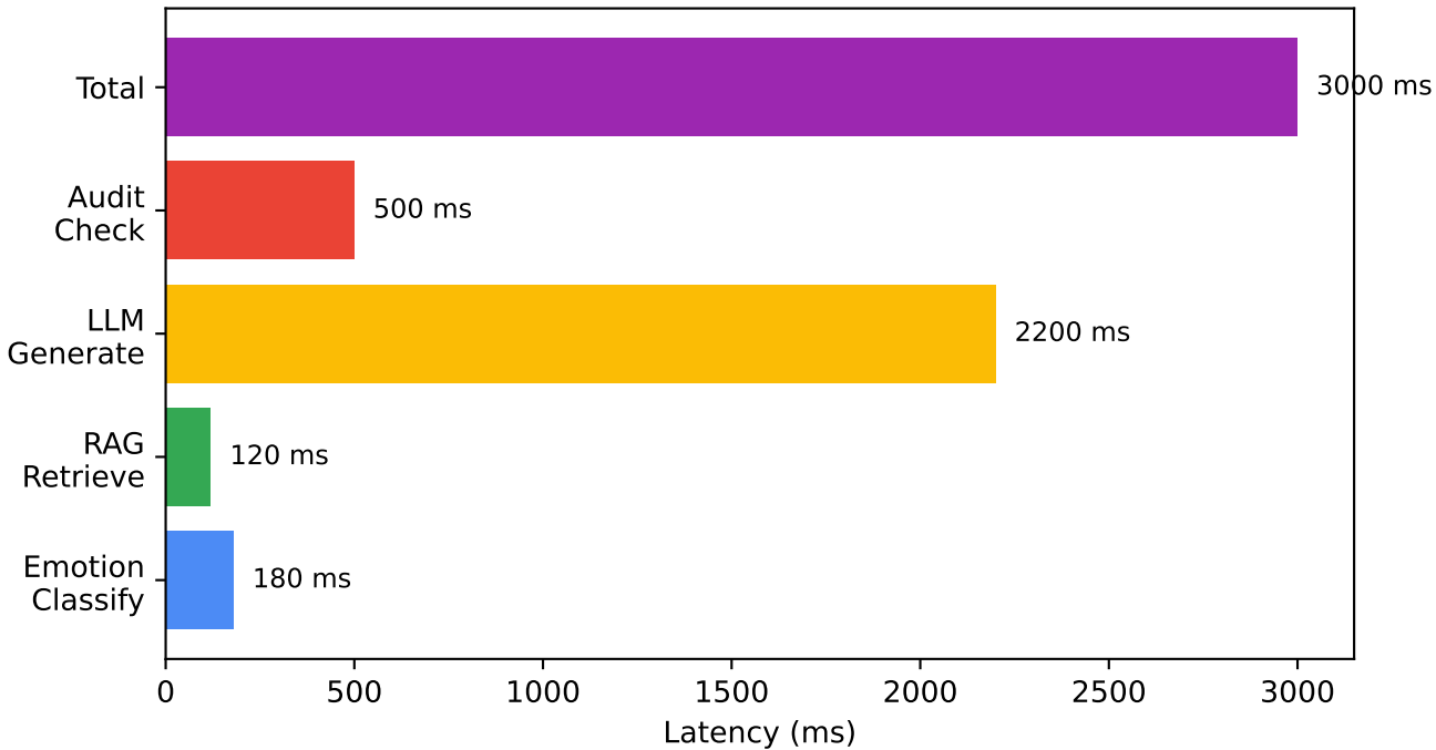
Response Latency Breakdown
