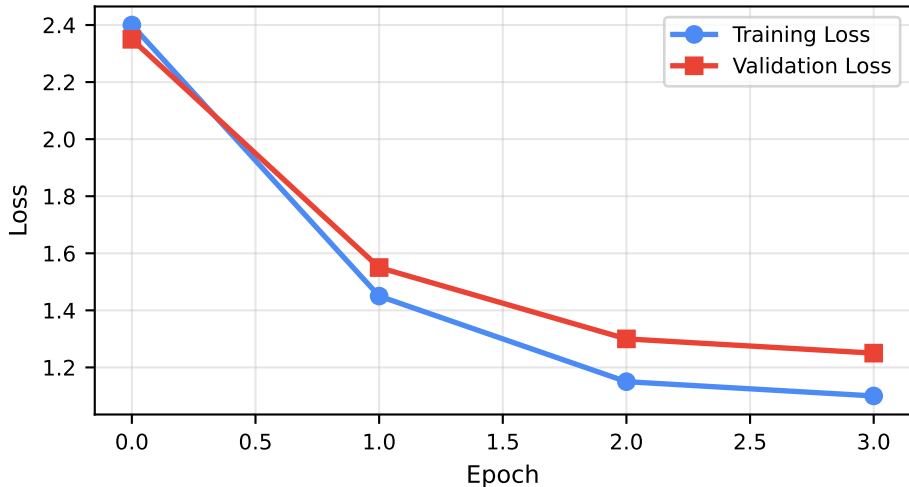
QLoRA Fine-Tuning Loss (Gemma 3 27B IT)
