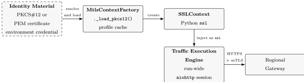
Figure 3.1: Secure Transport and mutual Transport Layer Security (mTLS) Management Layer. The secure-transport layer keeps certificate material and password resolution outside generated workload steps, making channel-establishment failures distinguishable from application responses. Source: Author’s elaboration based on the framework’s source code.
