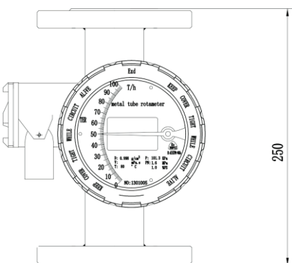
Round Converter
