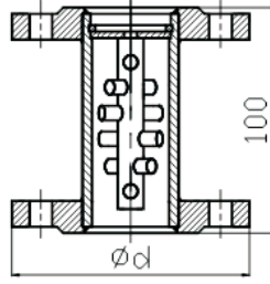
With Magnetic Filter
