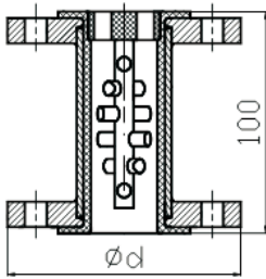
Liner FEP with Magnetic Filter
