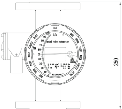
Round Converter
