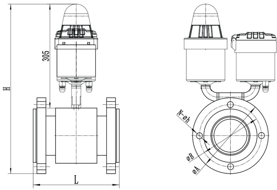
Battery with RS485 MODBUS/Wireless and DIN PN16 flange Drawing (Unit: mm)
