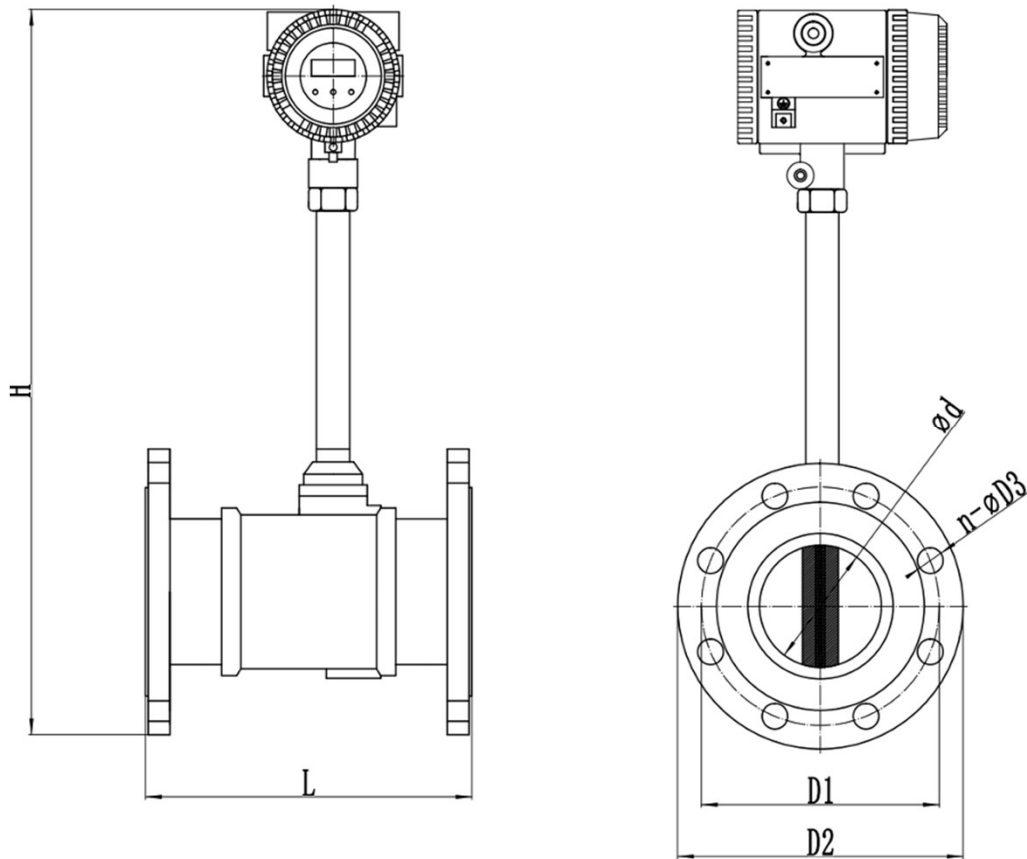
< Standard Type > 플랜지형 KVTX-3000
