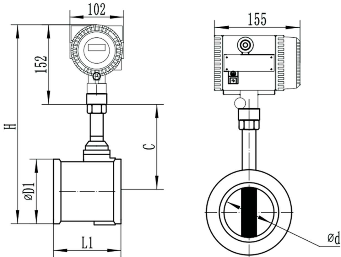
< Wafer Type > 웨이퍼형 KVTX-3000W
