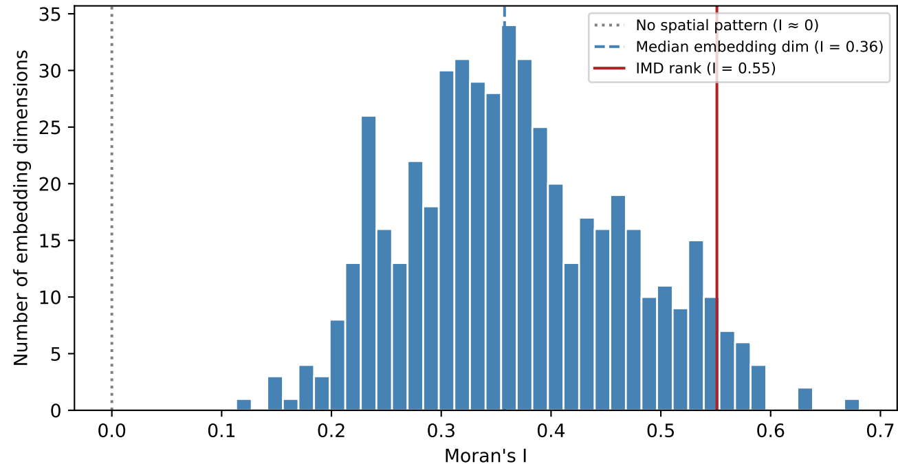
Spatial autocorrelation of the CLIP embedding dimensions
