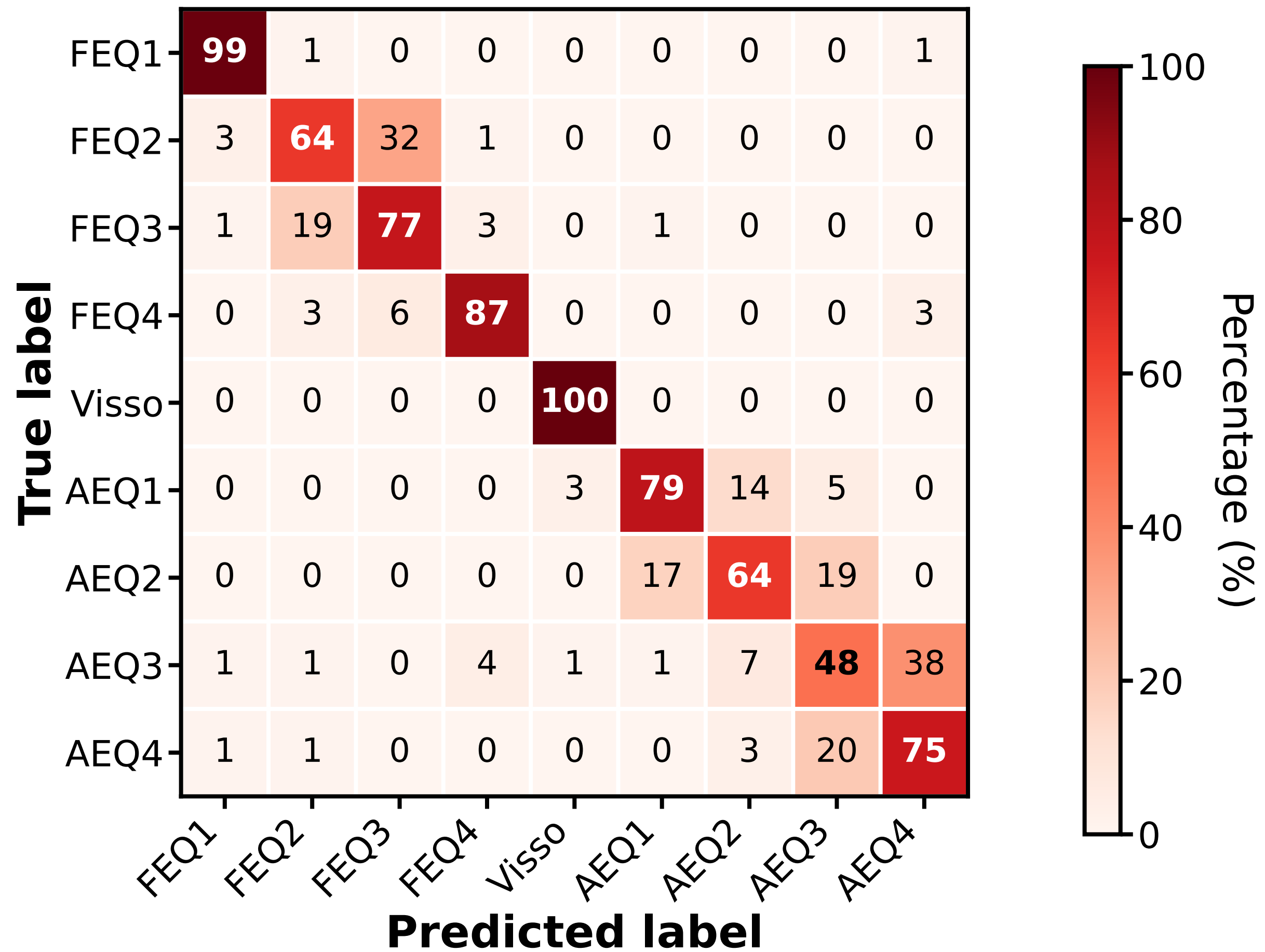
mLSTM CR; Acc: 76.96%
