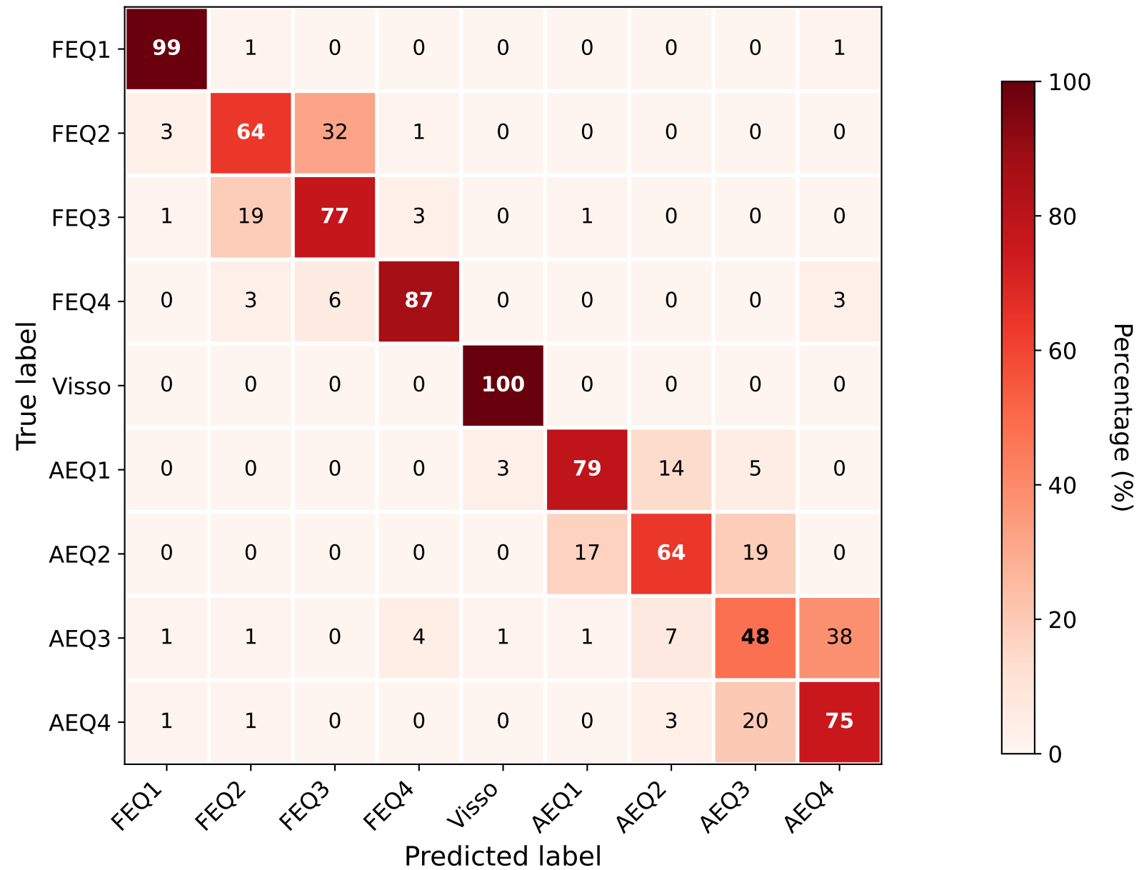
mLSTM CR; Acc: 76.96%
