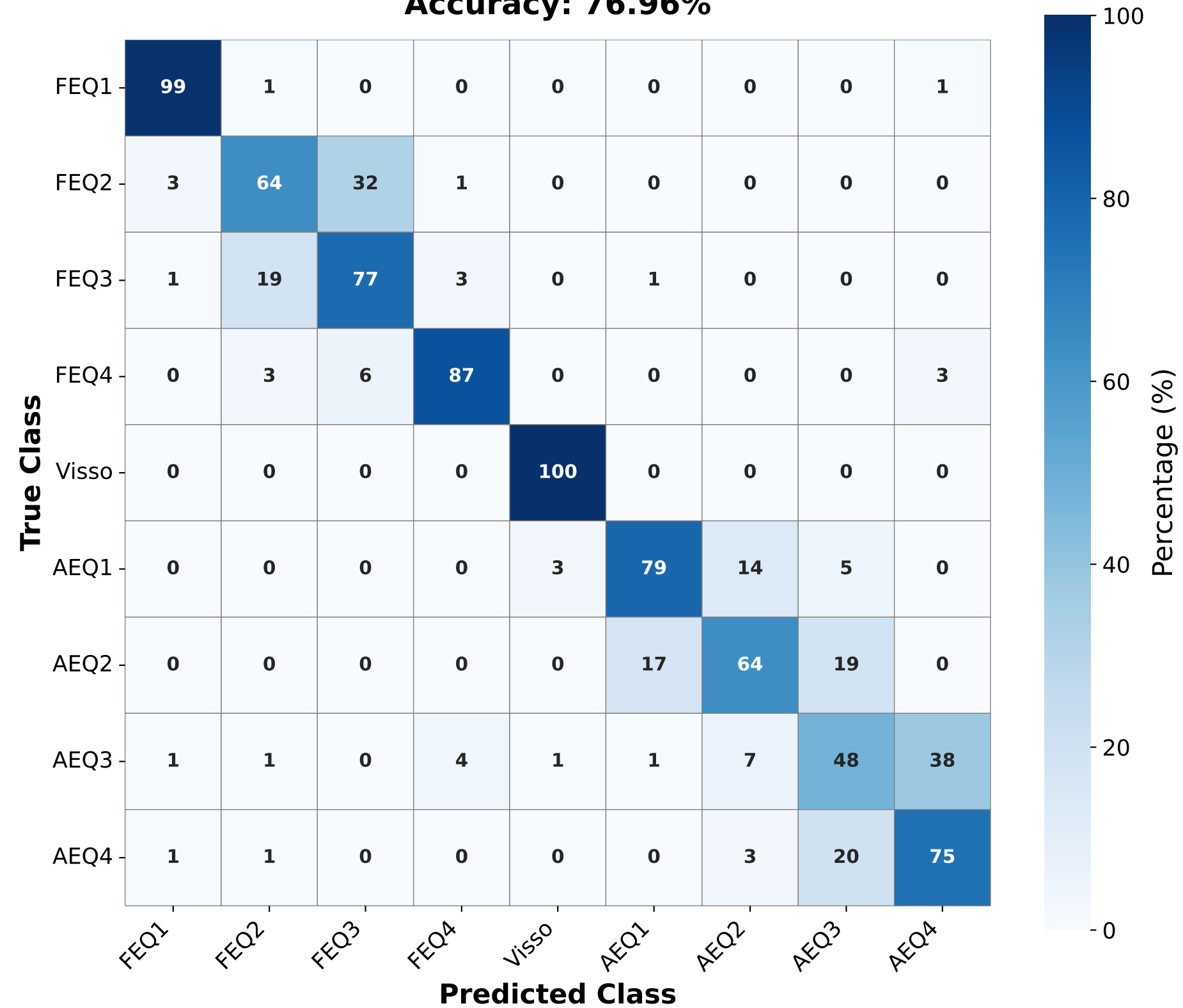
mLSTM CR Accuracy: 76.96%
