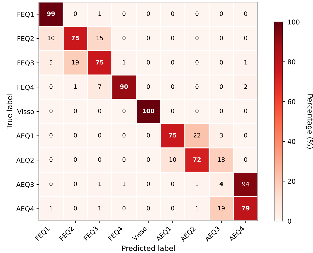
SeisLM-large; Acc: 74.22%
