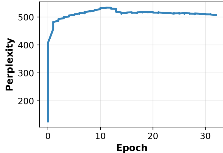
Codebook Perplexity
