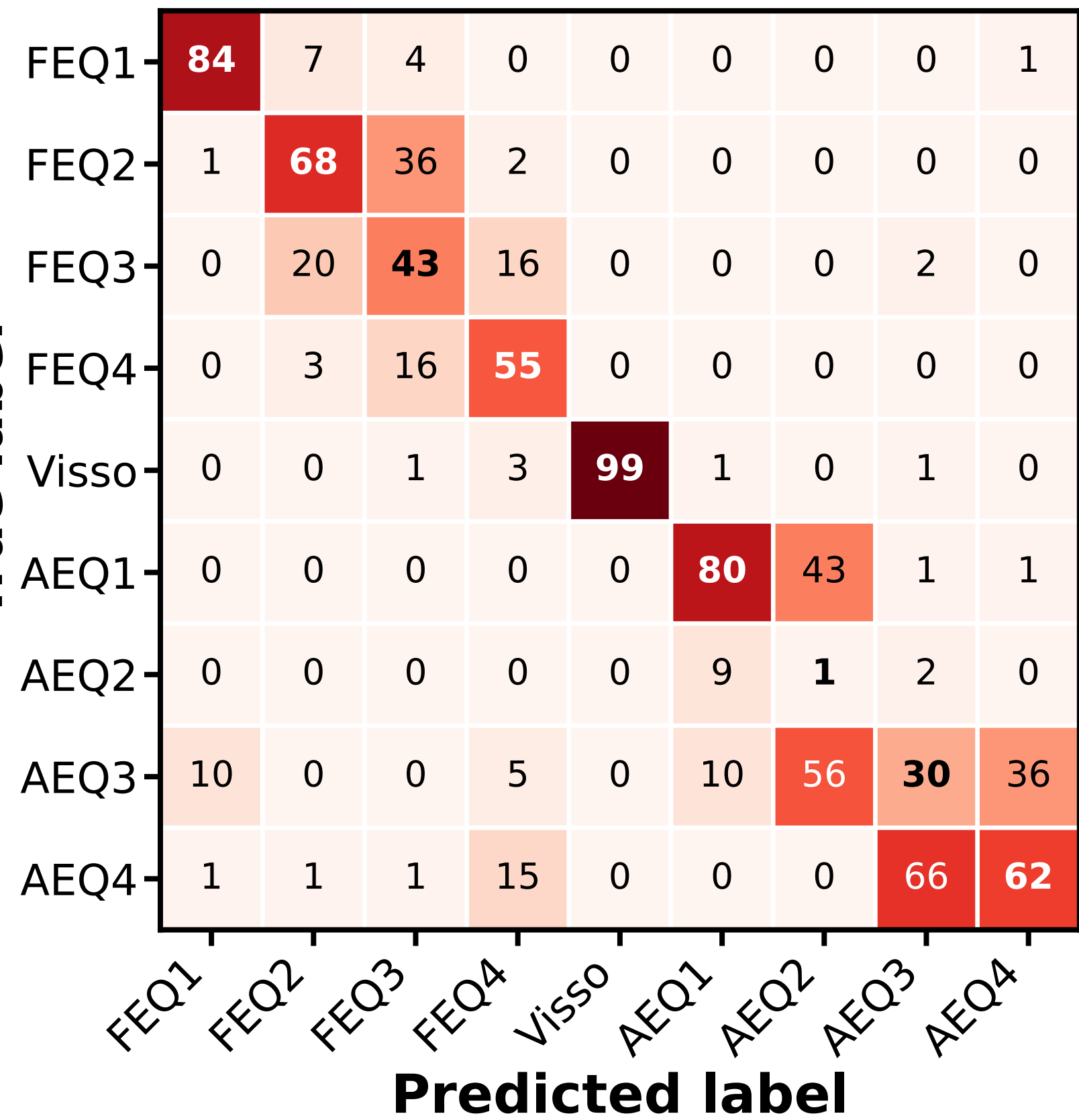
ConvNet; Acc: 58.33%
