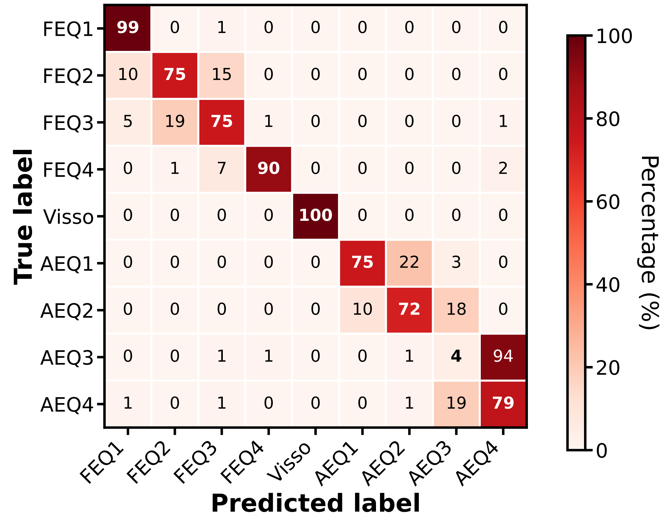
SeisLM-large; Acc: 74.22%
