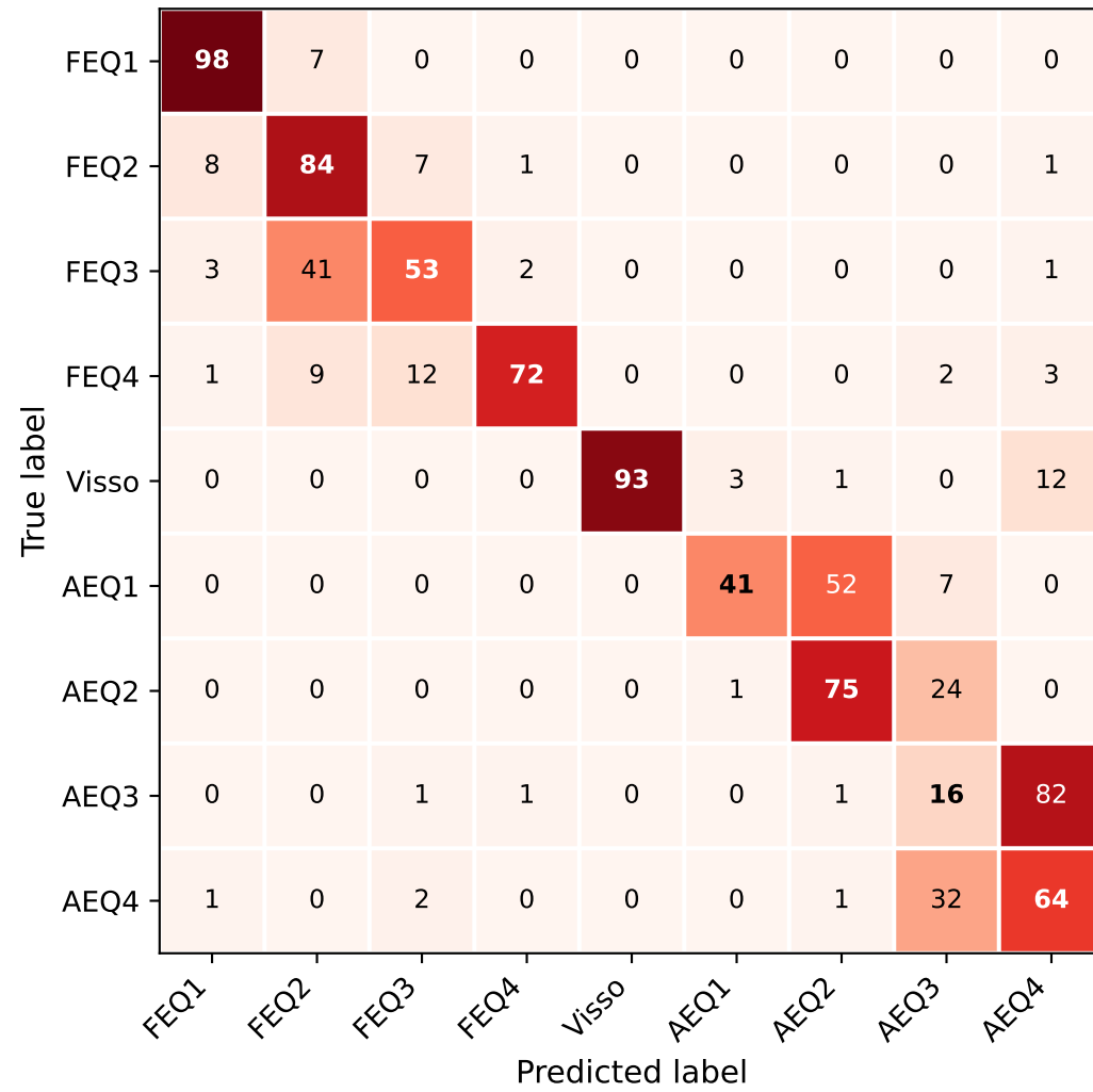
SeisLM-base; Acc: 65.11%
