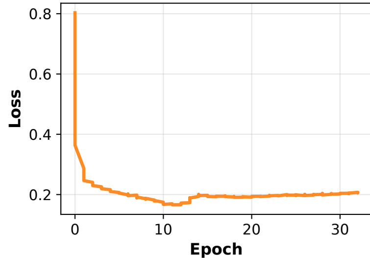
Diversity Loss
