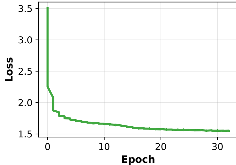
Contrastive Loss
