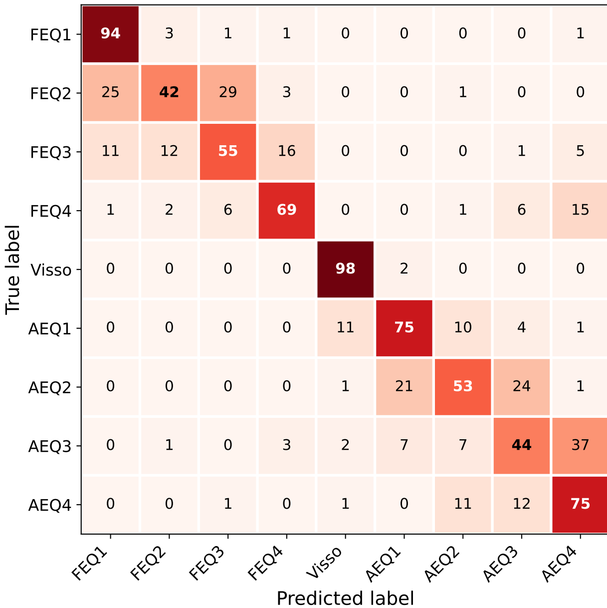
mLSTM Sequential; Acc: 67.17%
