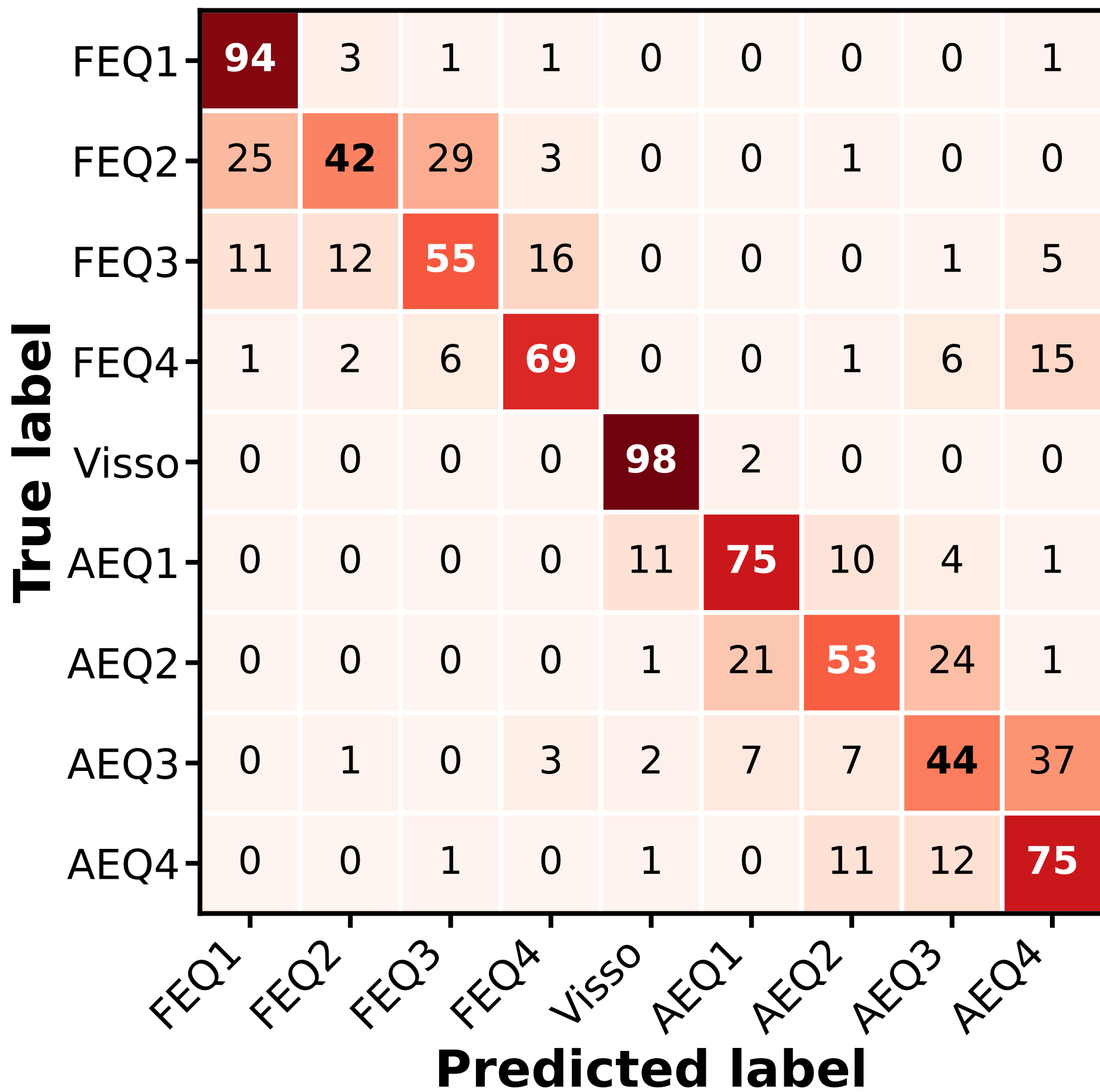
mLSTM Sequential; Acc: 67.17%
