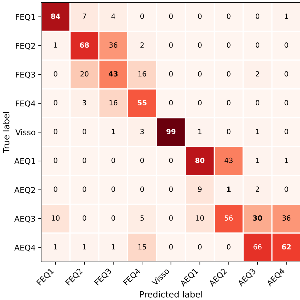
ConvNet; Acc: 58.33%
