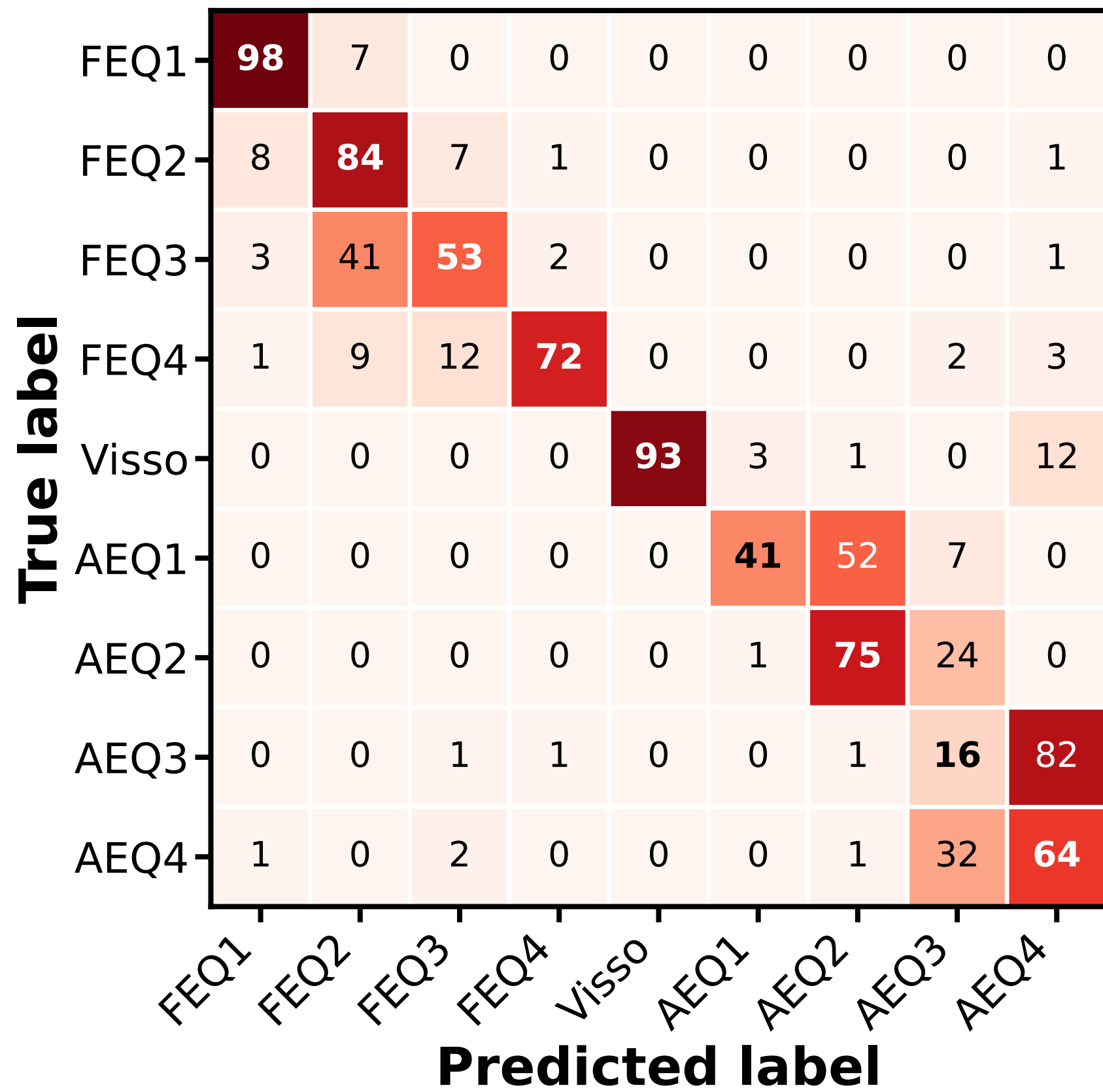
SeisLM-base; Acc: 65.11%
