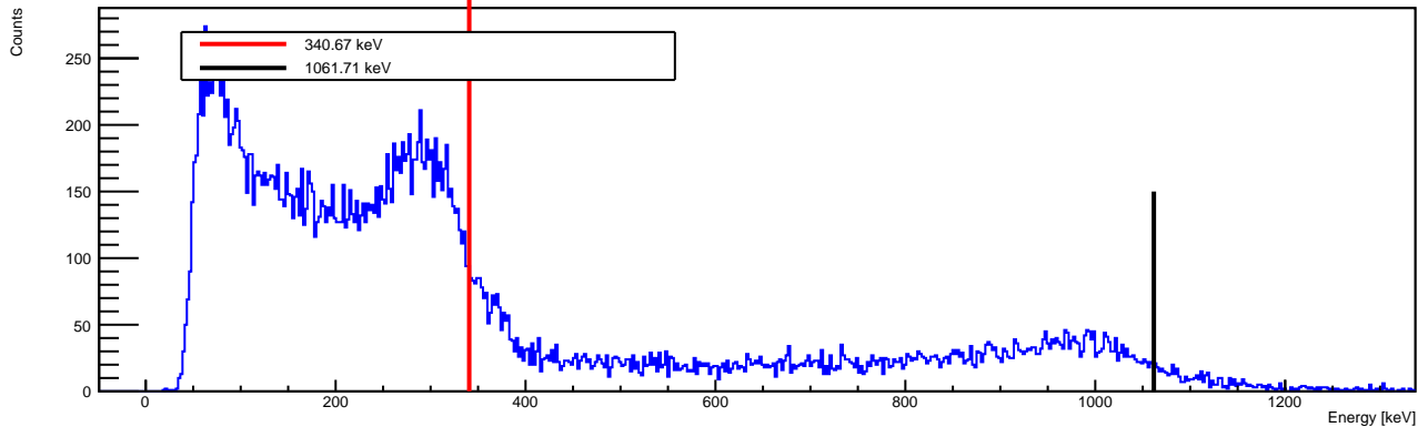
BC404 detector with 22Na (MBS)
