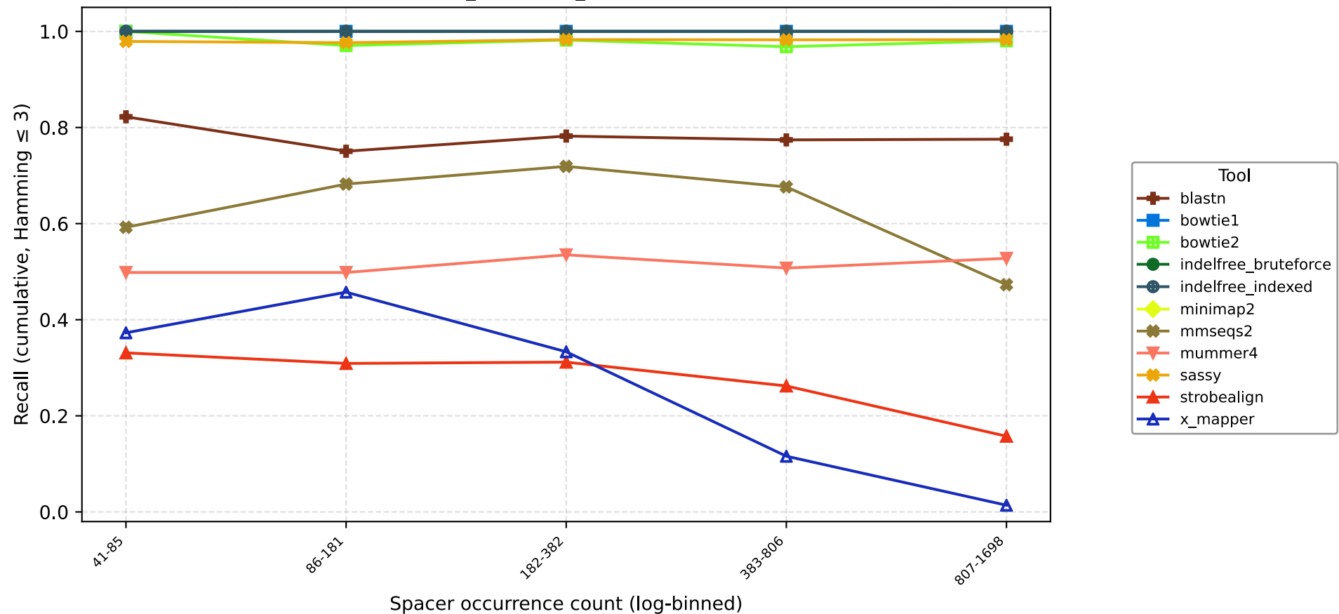
Recall vs spacer occurrence - HIGH_INSERTION_RATE simulation (cumulative Hamming \leq 3 )
