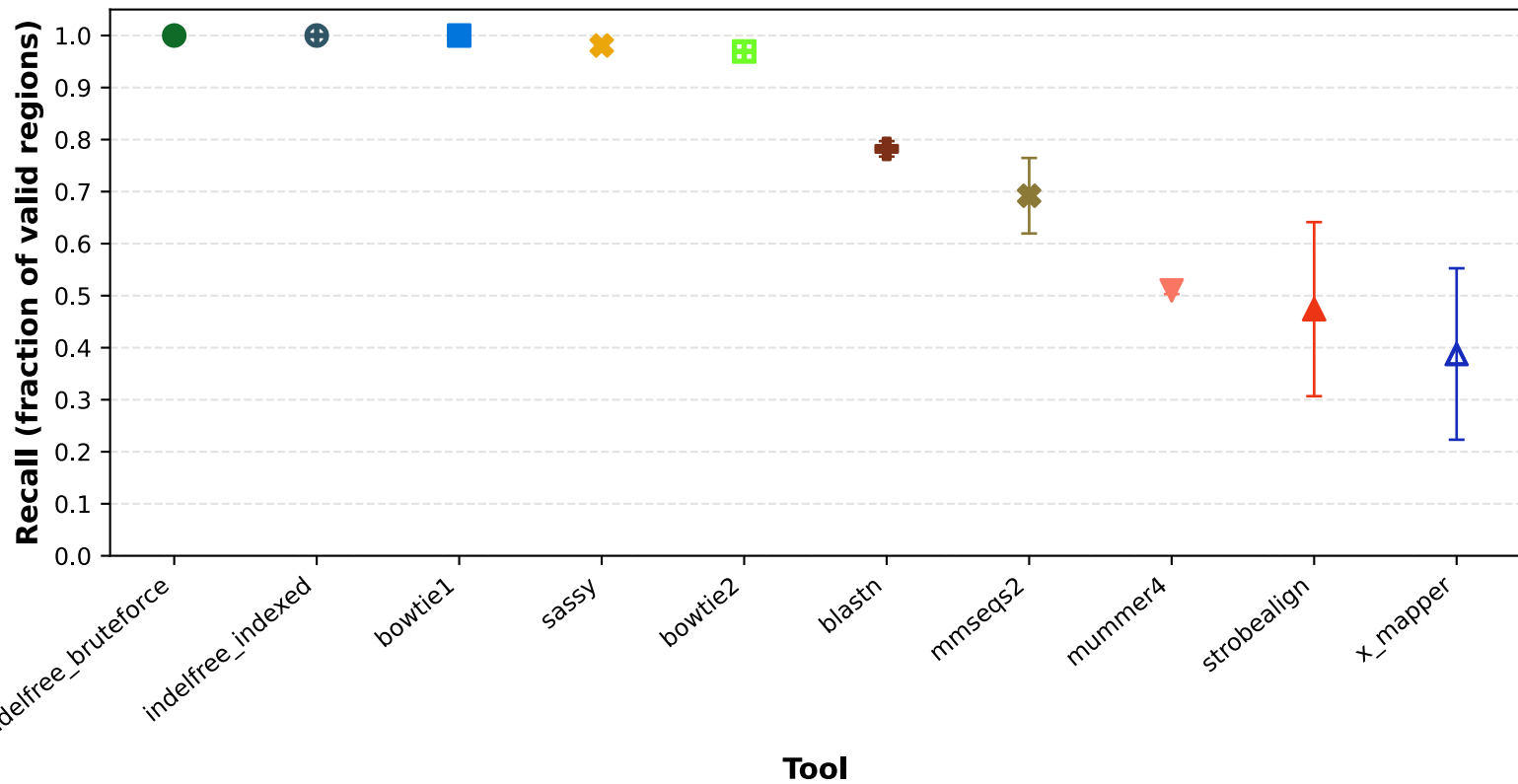
Simulated cross-dataset recall consistency at Hamming distance \leq 3 (mean \pm SD)
