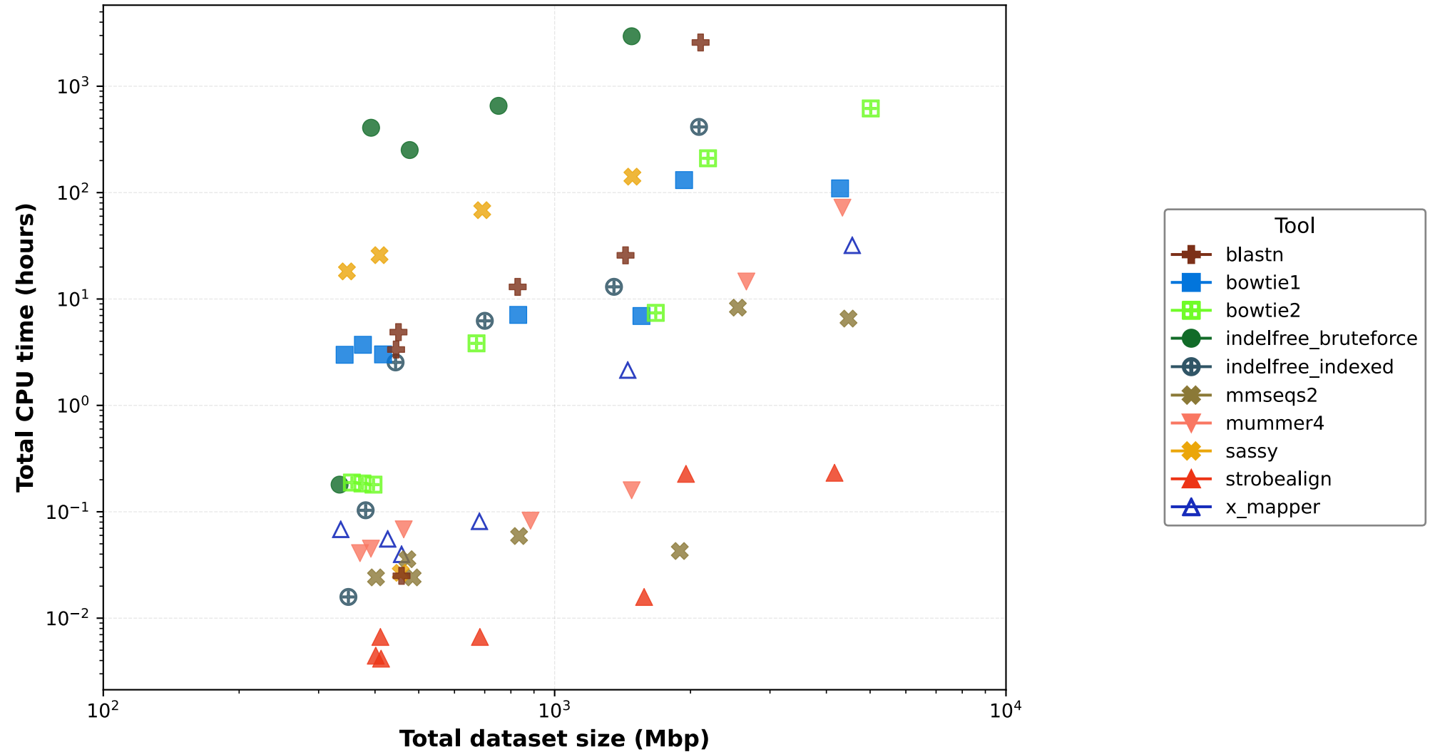
B. CPU time - Simulated datasets
