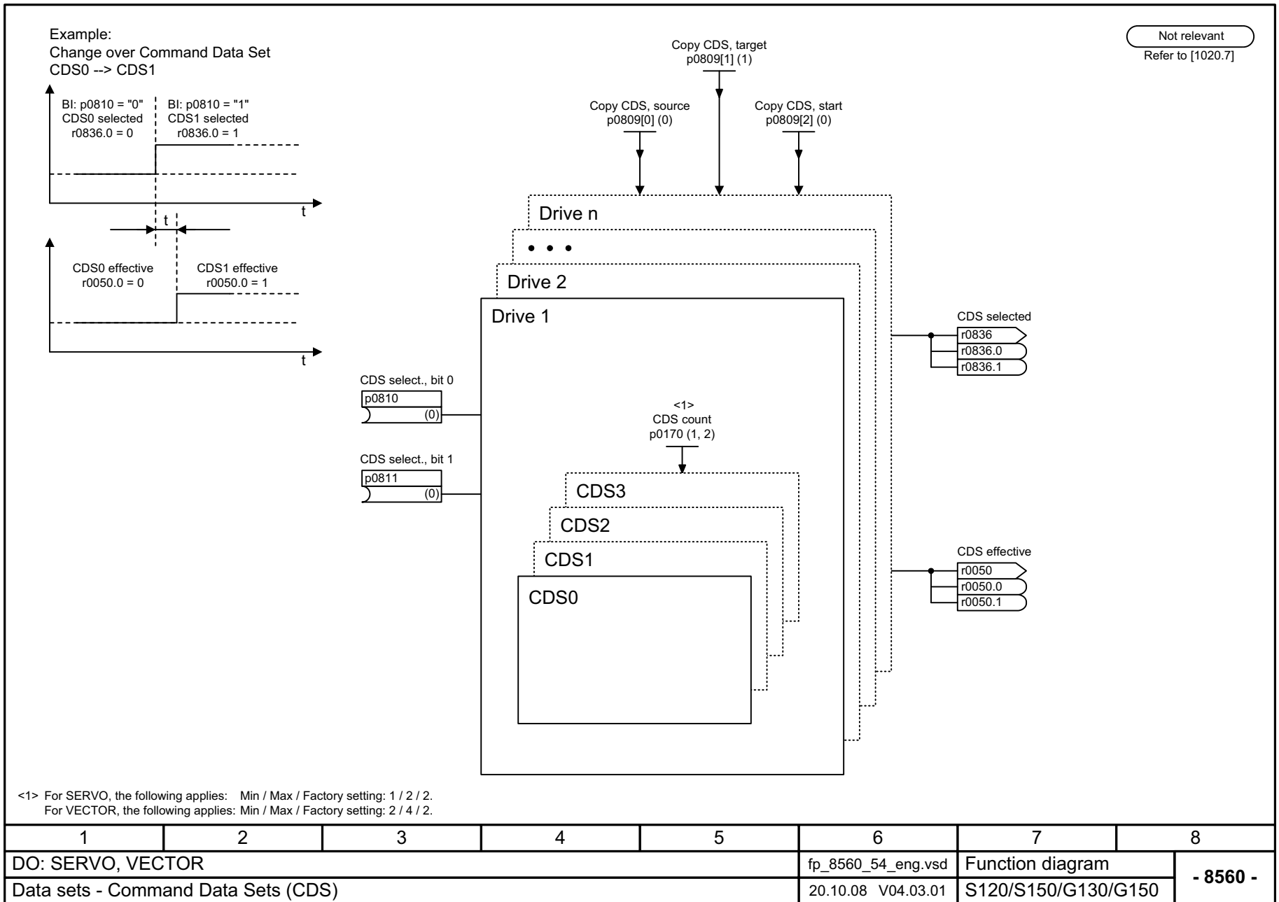
Fig. 2-129 8560 – Command data sets (CDS)
