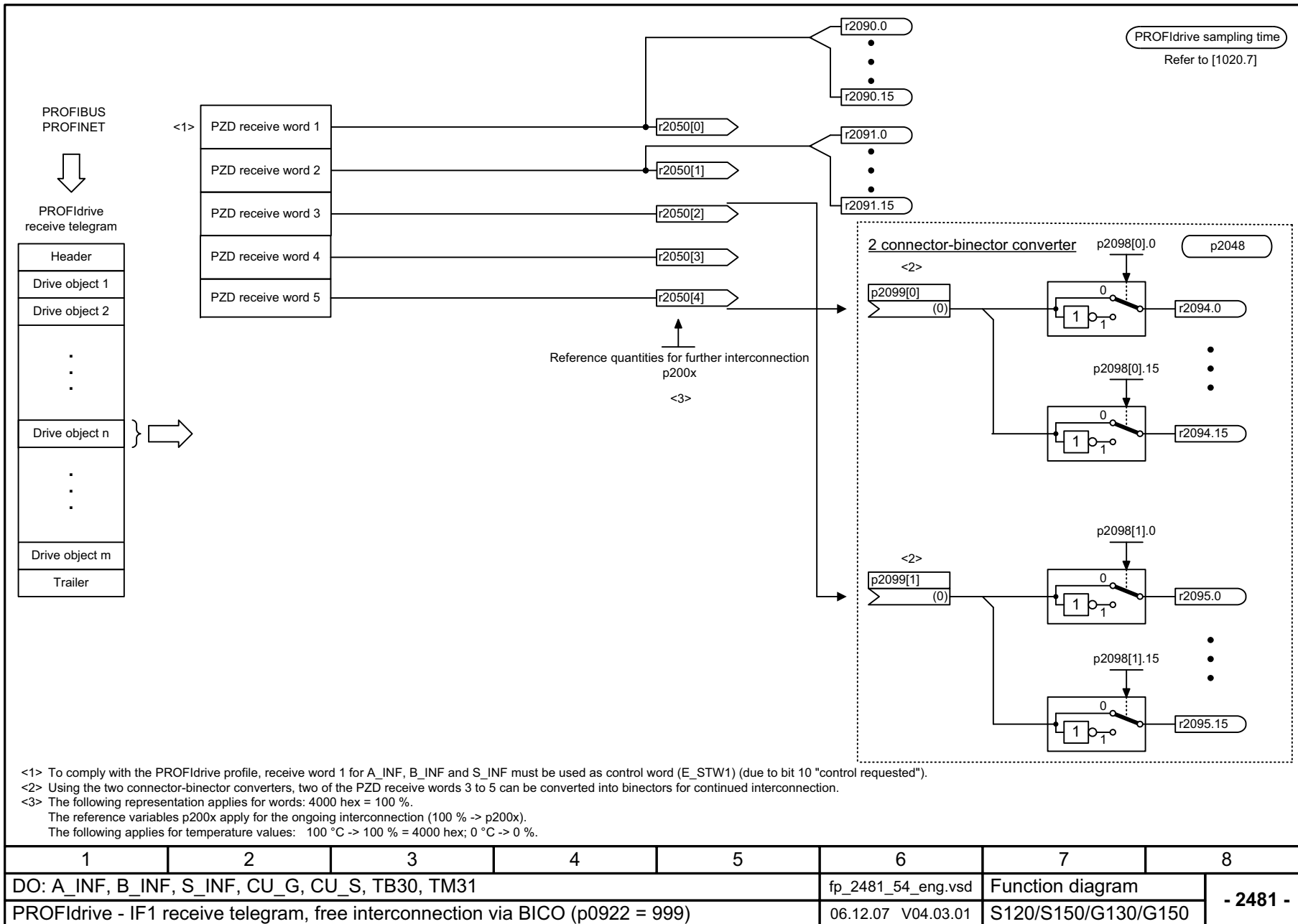
Fig. 2-43 2481 – IF1 receive telegram, free interconnection via BICO (p0922 = 999)
