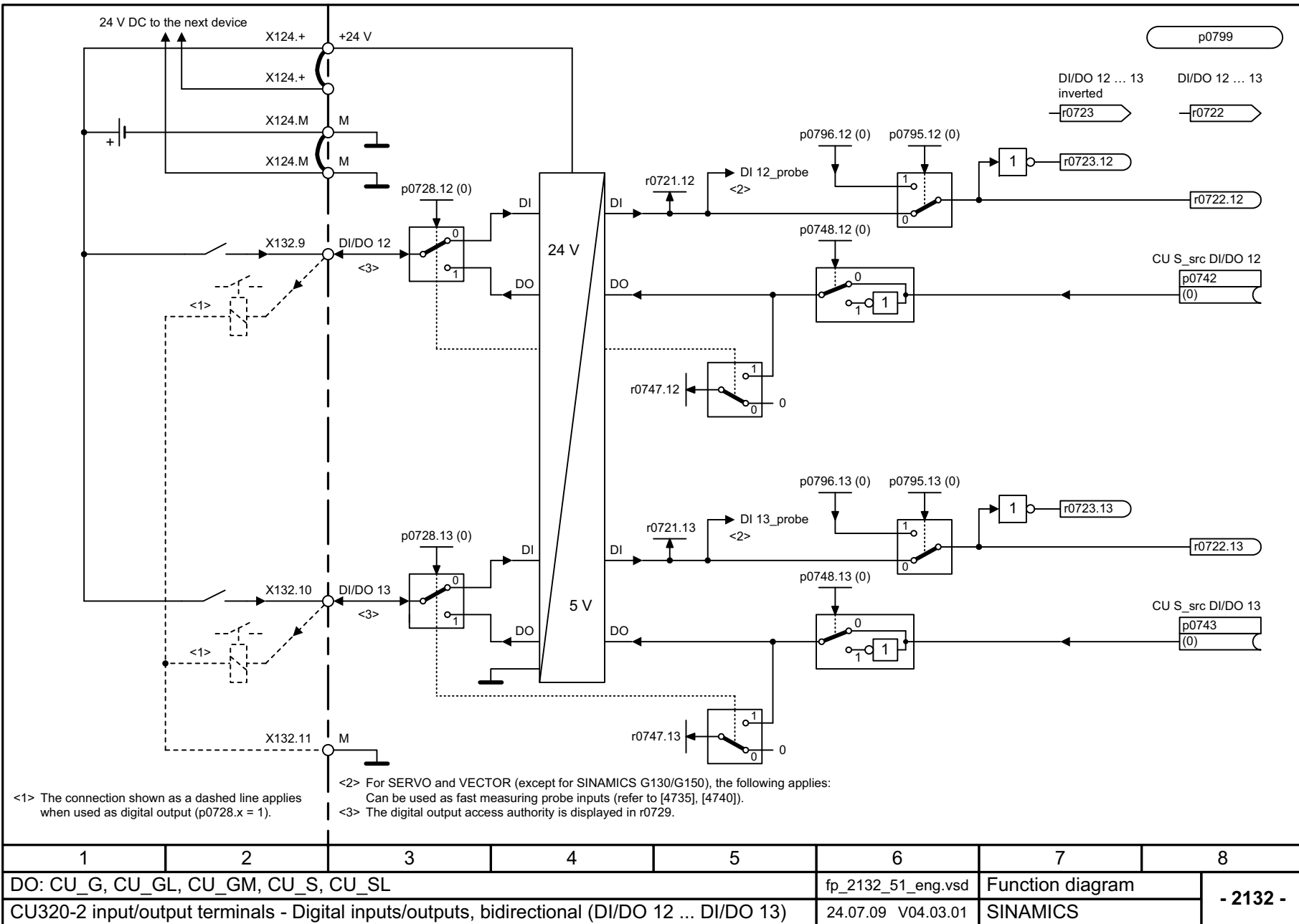
Fig. 2-20 2132 – Digital inputs/outputs, bidirectional (DI/DO 12 to DI/DO 13)
