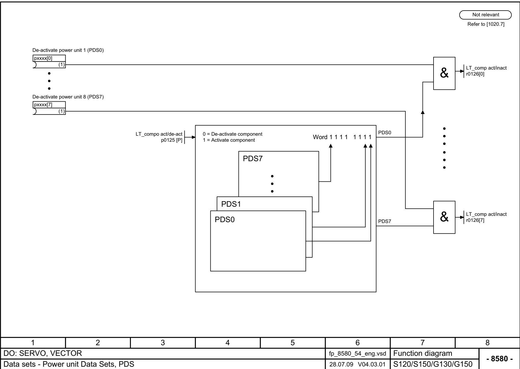
Fig. 2-133 8580 – Power unit data sets (PDS)
