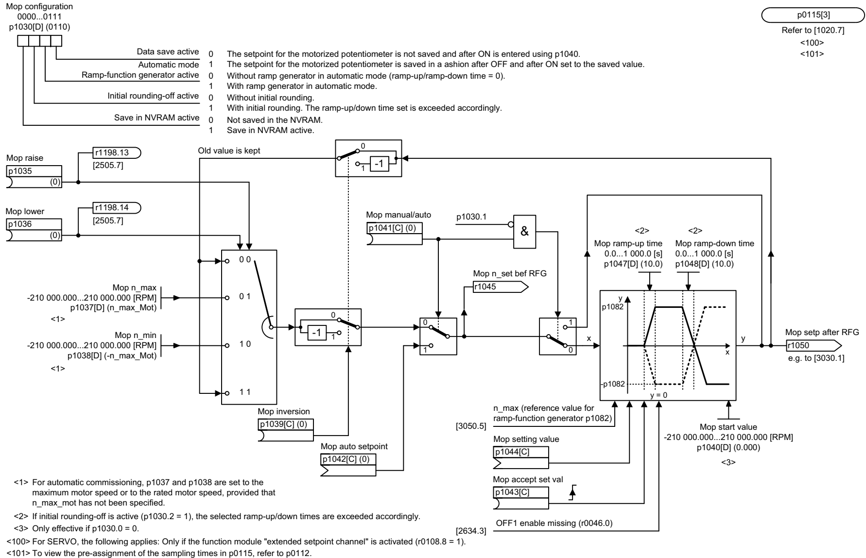
Fig. 2-76 3020 – Motorized potentiometer
