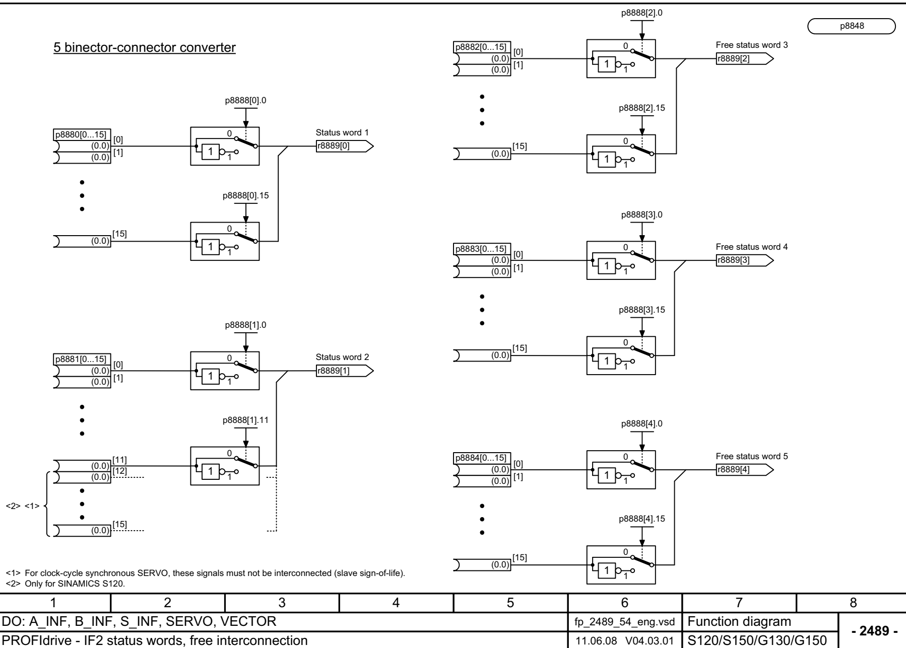
Fig. 2-47 2489 – IF2 status words, free interconnection
