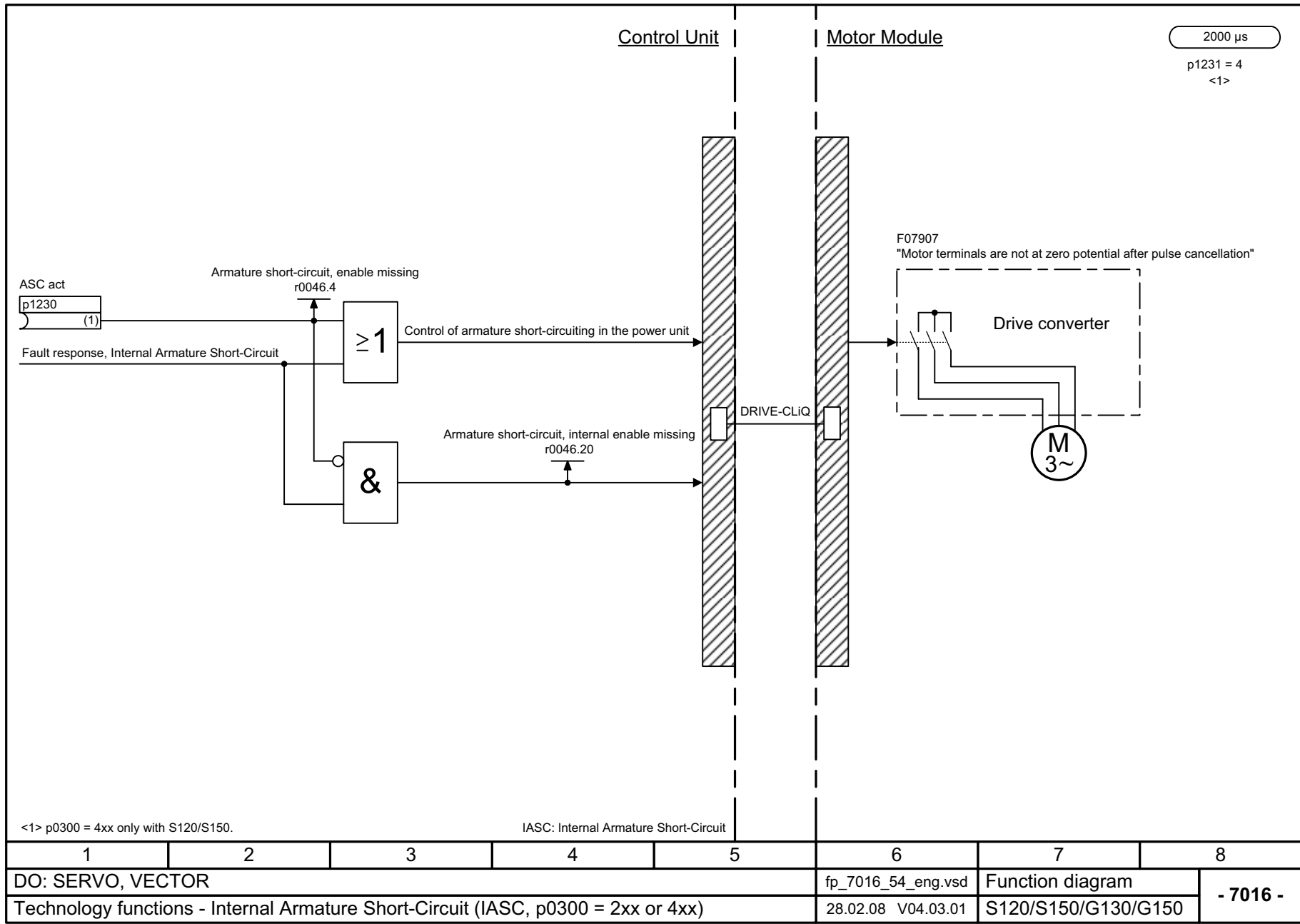
Fig. 2-109 7016 – Internal armature short-circuit (IASC, p0300 = 2xx)
