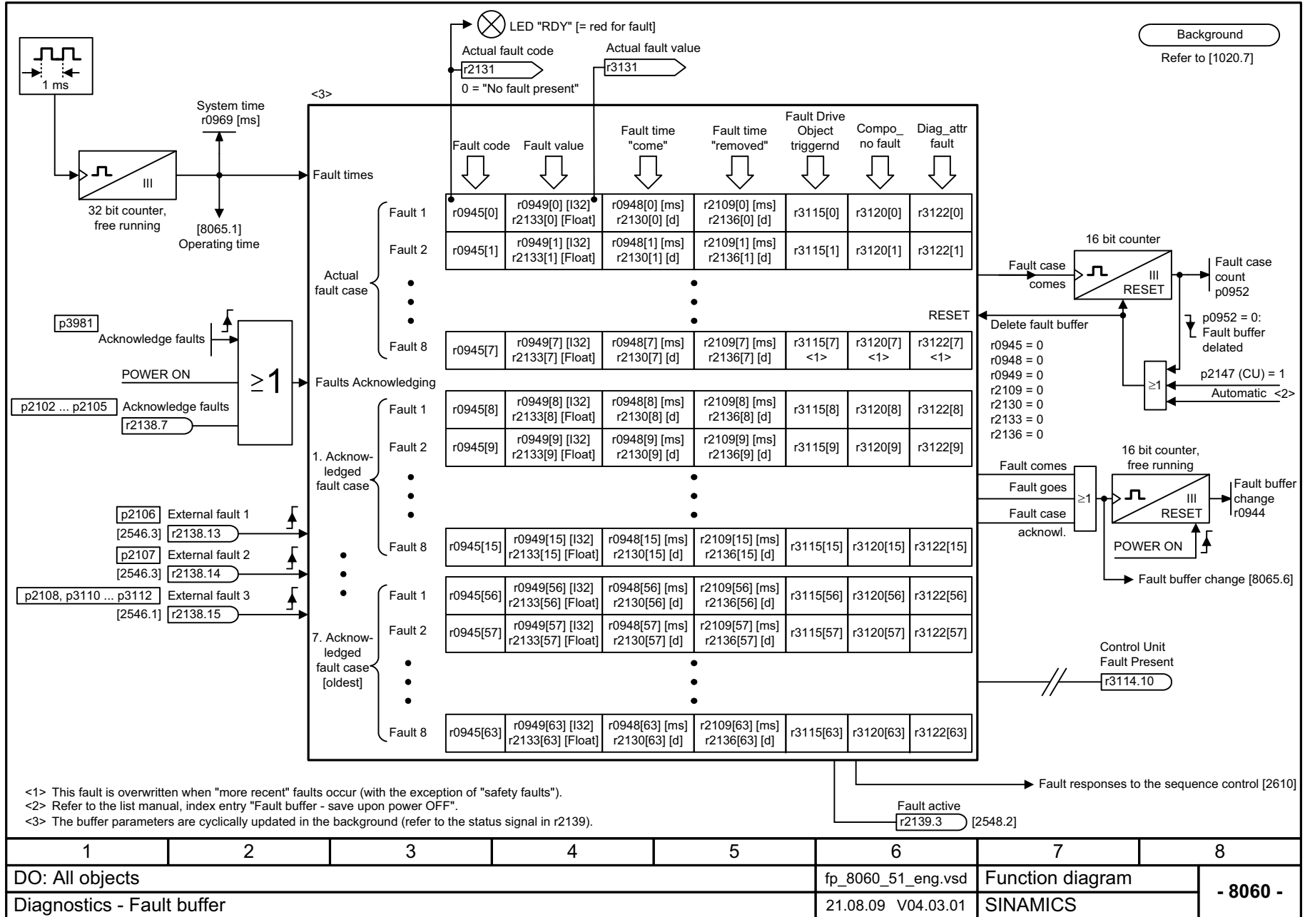
Fig. 2-124 8060 – Fault buffer
