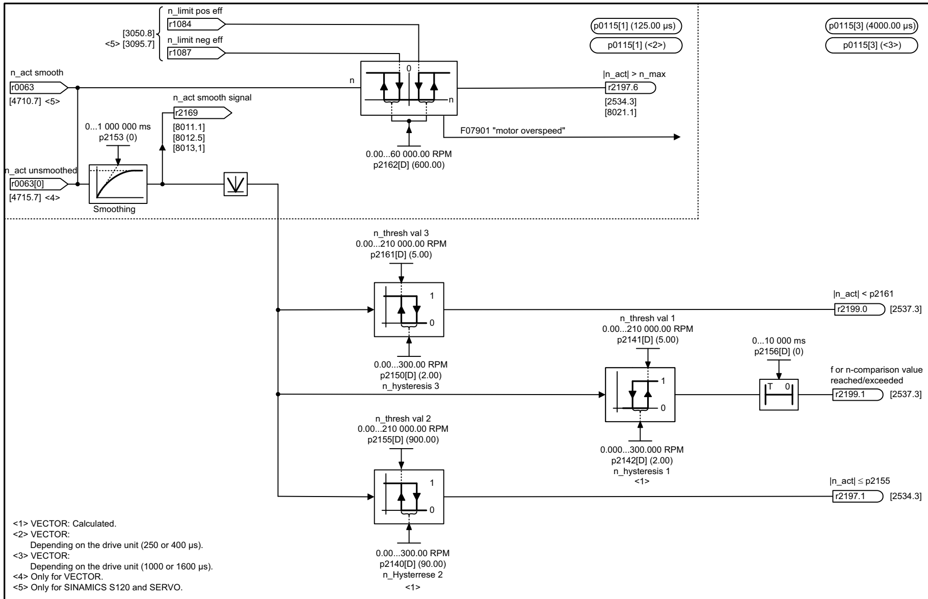
Fig. 2-117 8010 – Speed messages 1
