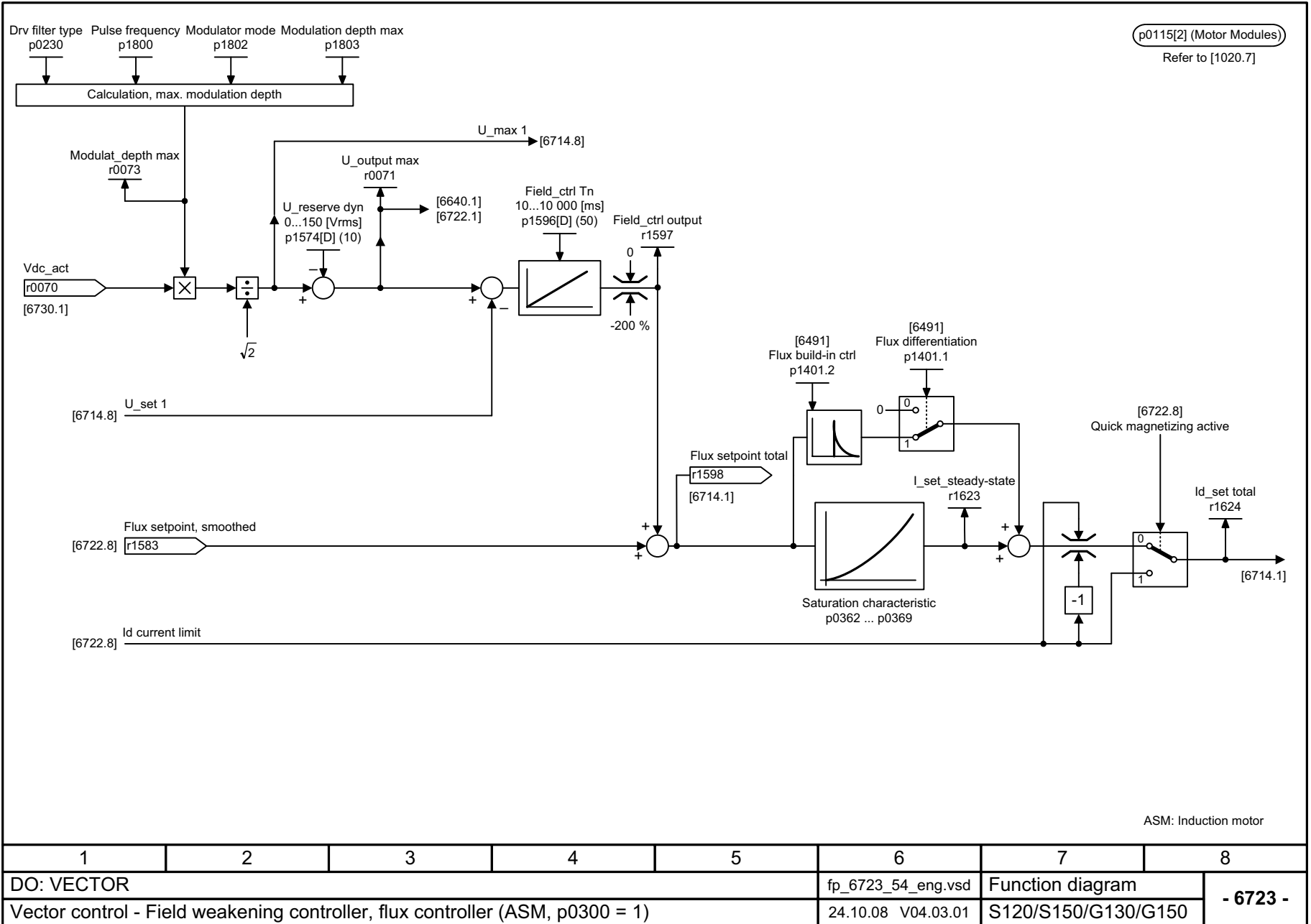
Fig. 2-102 6723 – Field weakening controller, flux controller (ASM, p0300 = 1)
