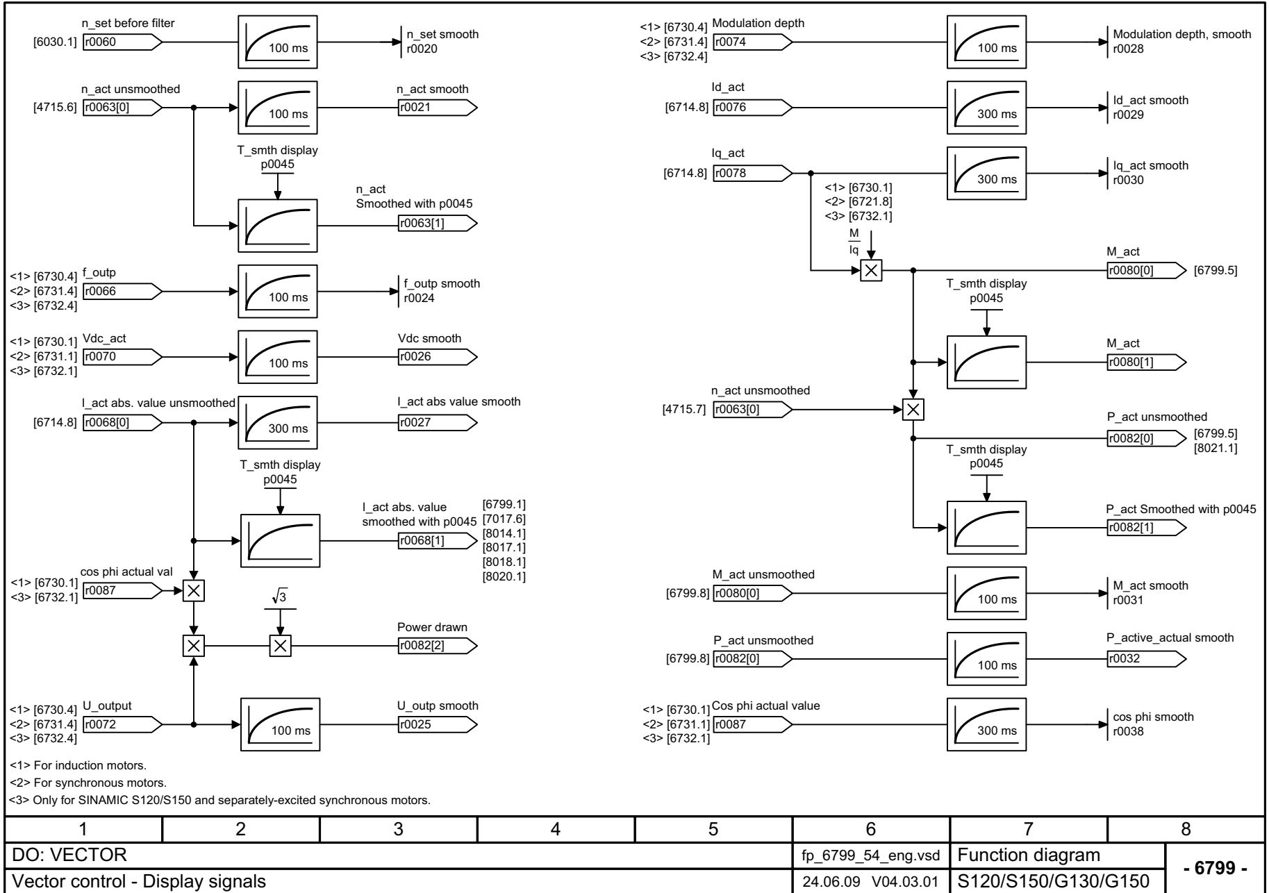
Fig. 2-106 6799 – Display signals
