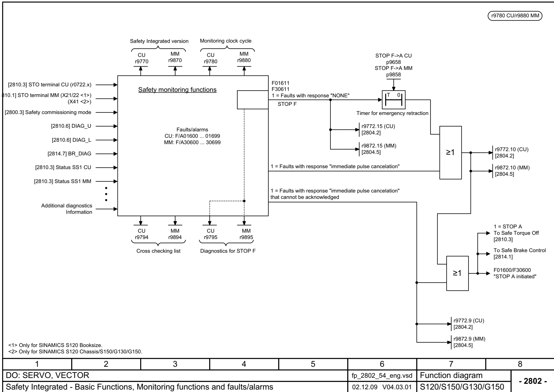
Fig. 2-71 2802 – Basic functions, monitoring and faults/alarms
