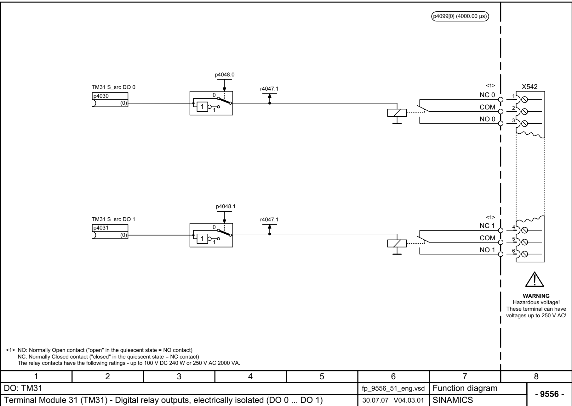
Fig. 2-146 9556 – Digital relay outputs, isolated (DO 0 to DO 1)
