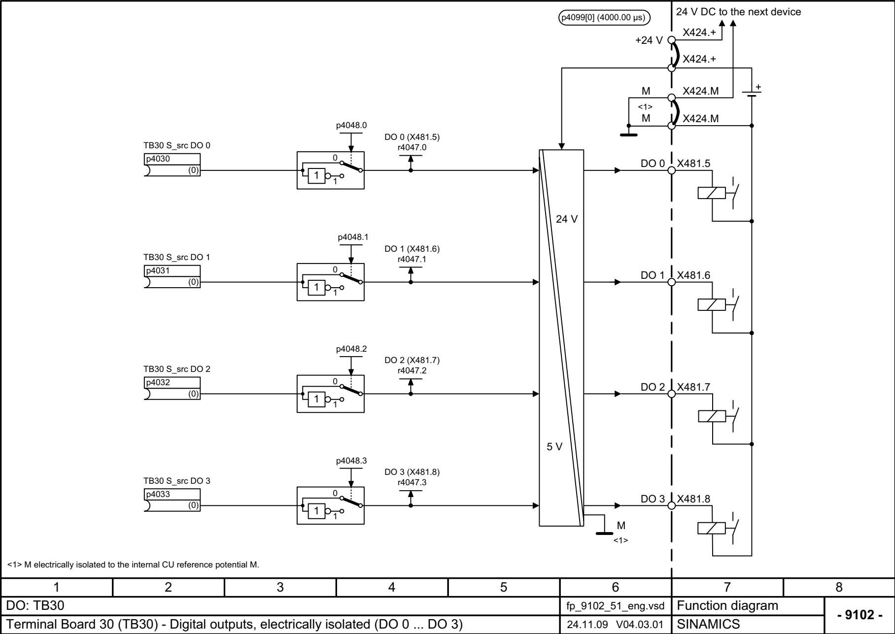
Fig. 2-135 9102 – Digital outputs, isolated (DO 0 to DO 3)
