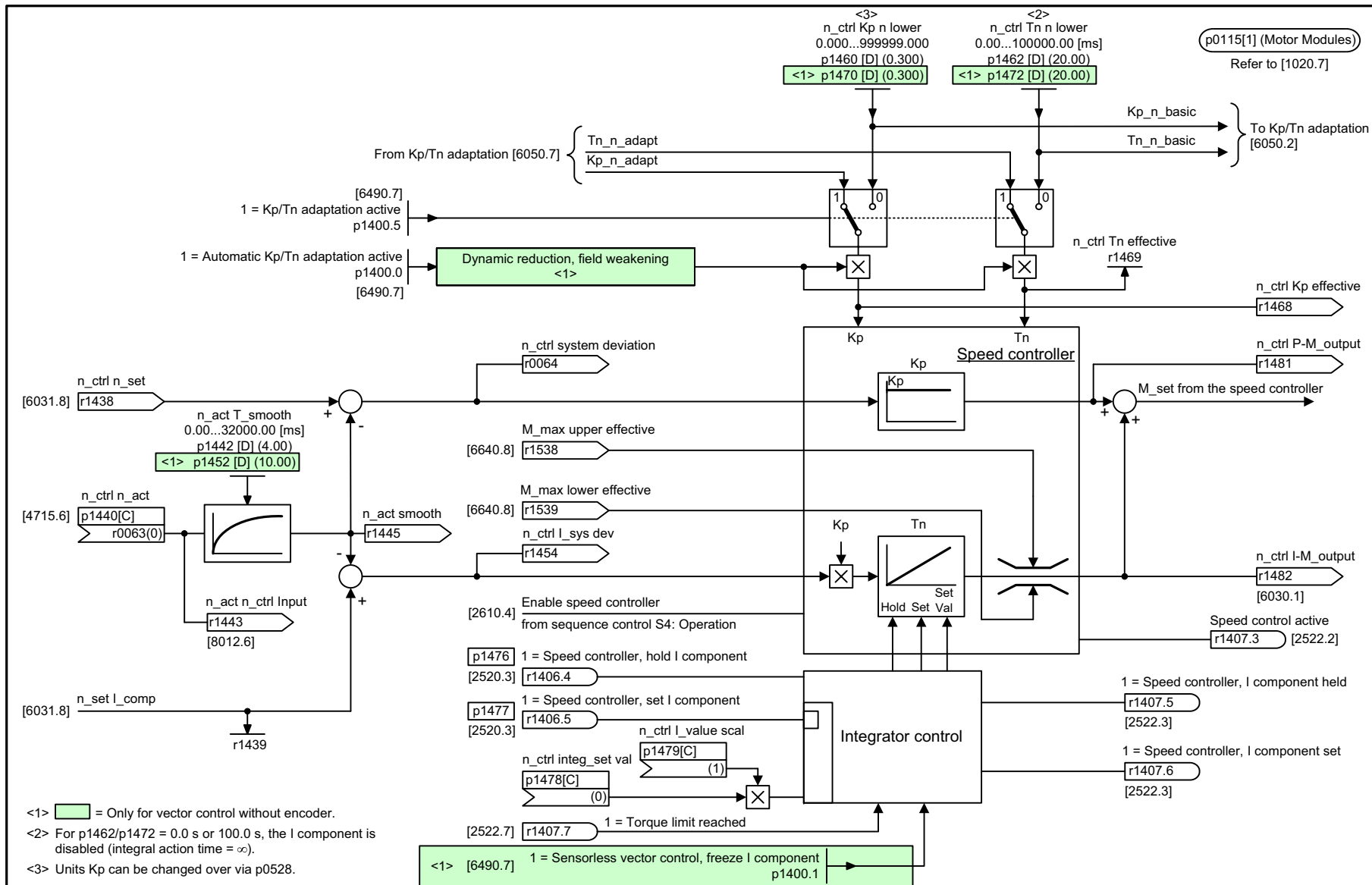
Fig. 2-87 6040 – Speed controller with/without encoder
