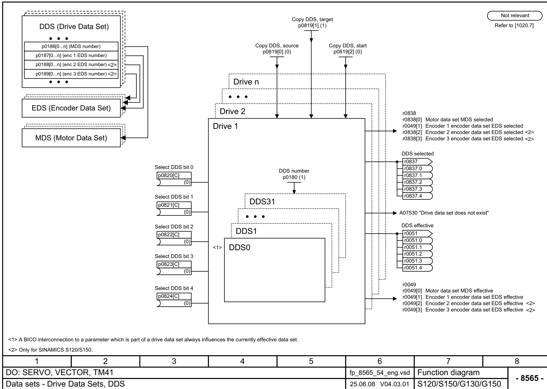
Fig. 2-130 8565 – Drive data sets (DDS)
