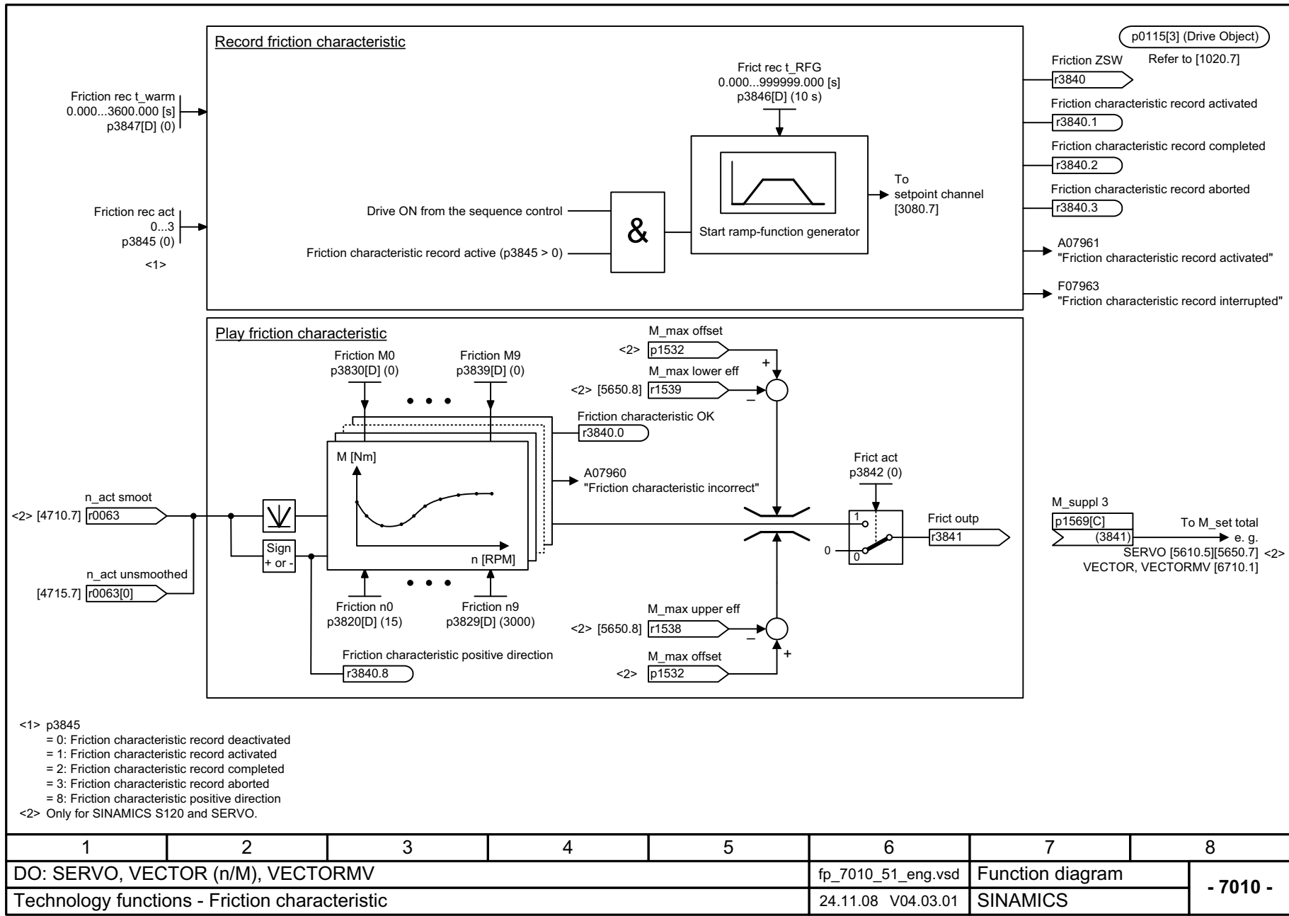
Fig. 2-107 7010 – Friction characteristic
