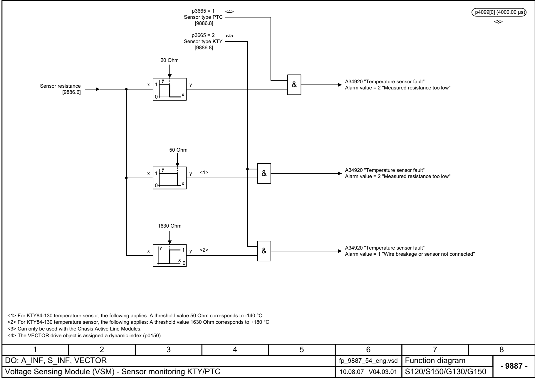
Fig. 2-156 9887 – Sensor monitoring KTY/PTC
