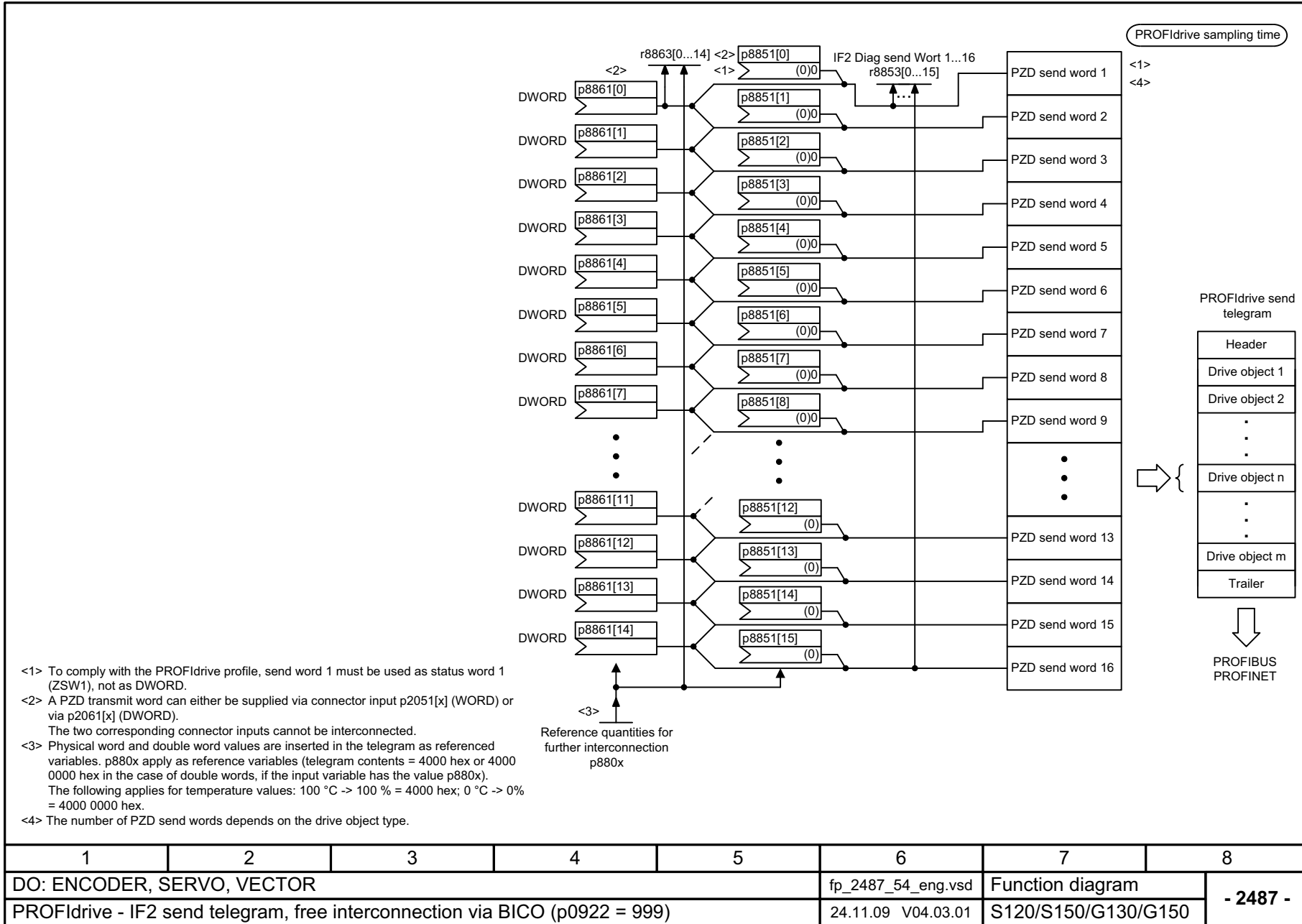
Fig. 2-46 2487 – IF2 send telegram, free interconnection via BICO (p0922 = 999)
