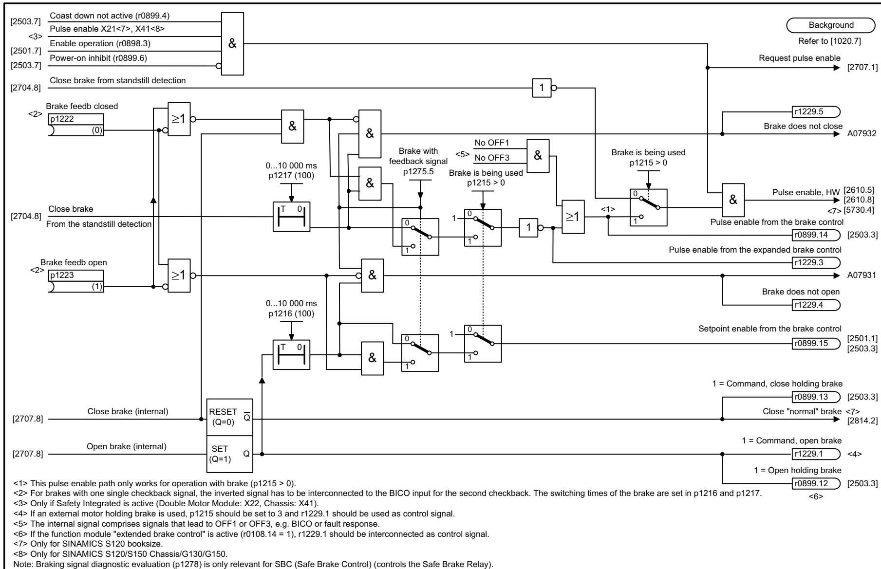
Fig. 2-69 2711 – Extended brake control, signal outputs (r0108.14 = 1)
