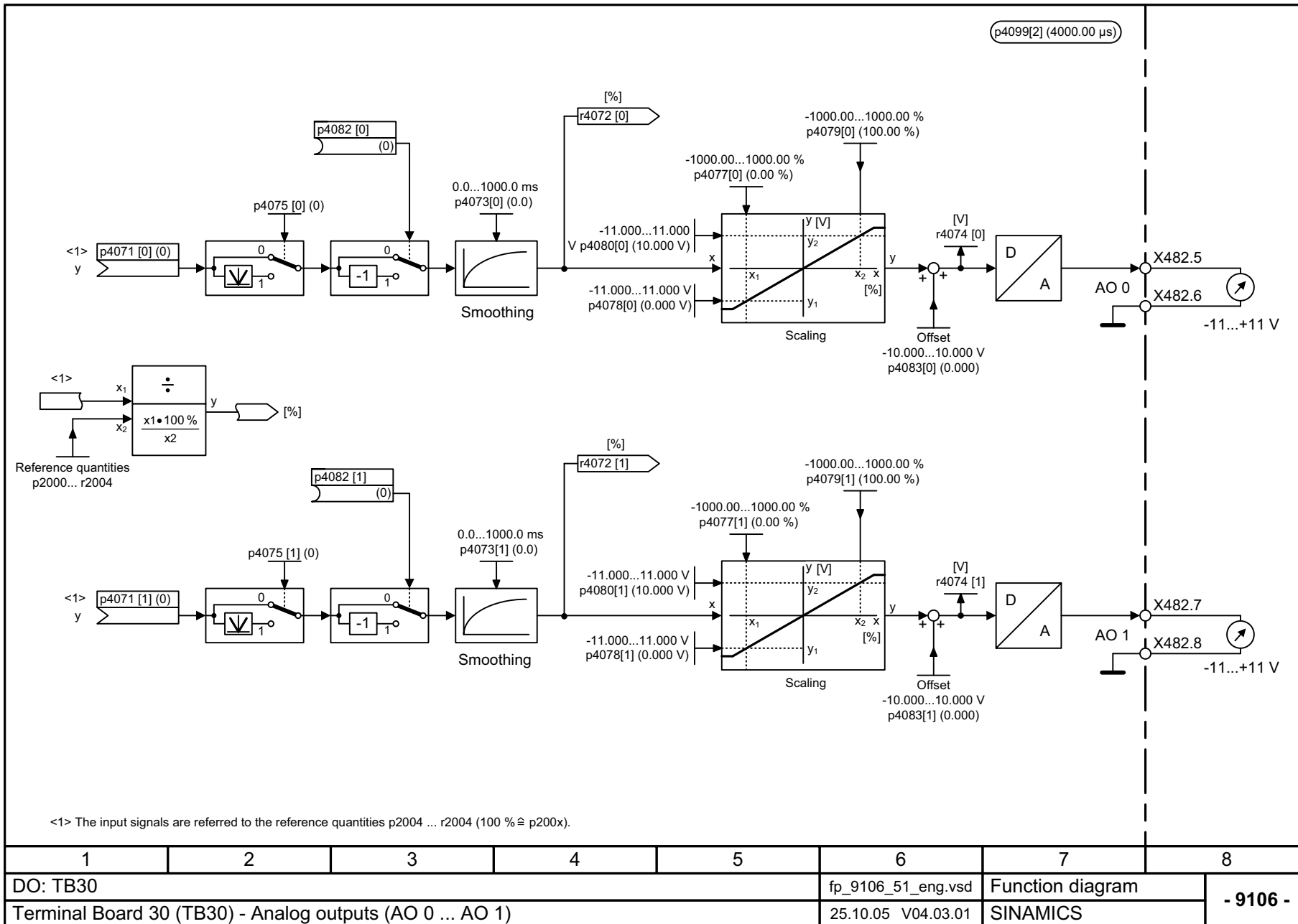
Fig. 2-137 9106 – Analog outputs (AO 0 to AO 1)
