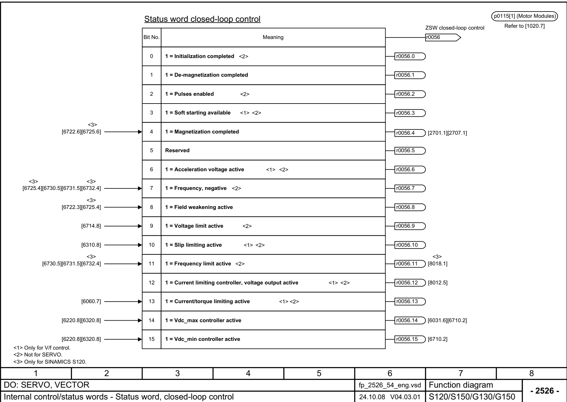
Fig. 2-57 2526 – Status word, closed loop control
