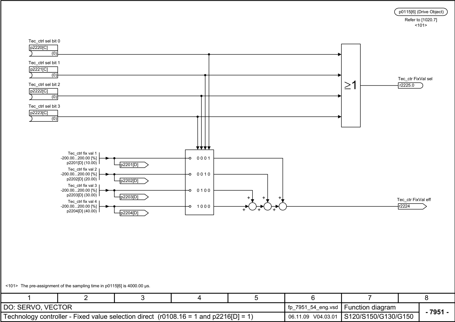
Fig. 2-113 7951 – Fixed values, direct selection (r0108.16 = 1 and p2216[D] = 1)
