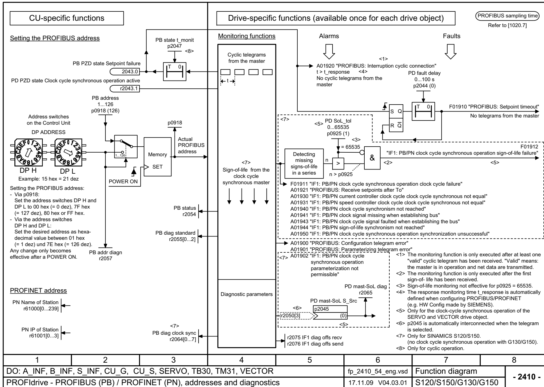
Fig. 2-22 2410 – PROFIBUS (PB)/PROFINET (PN), addresses and diagnostics
