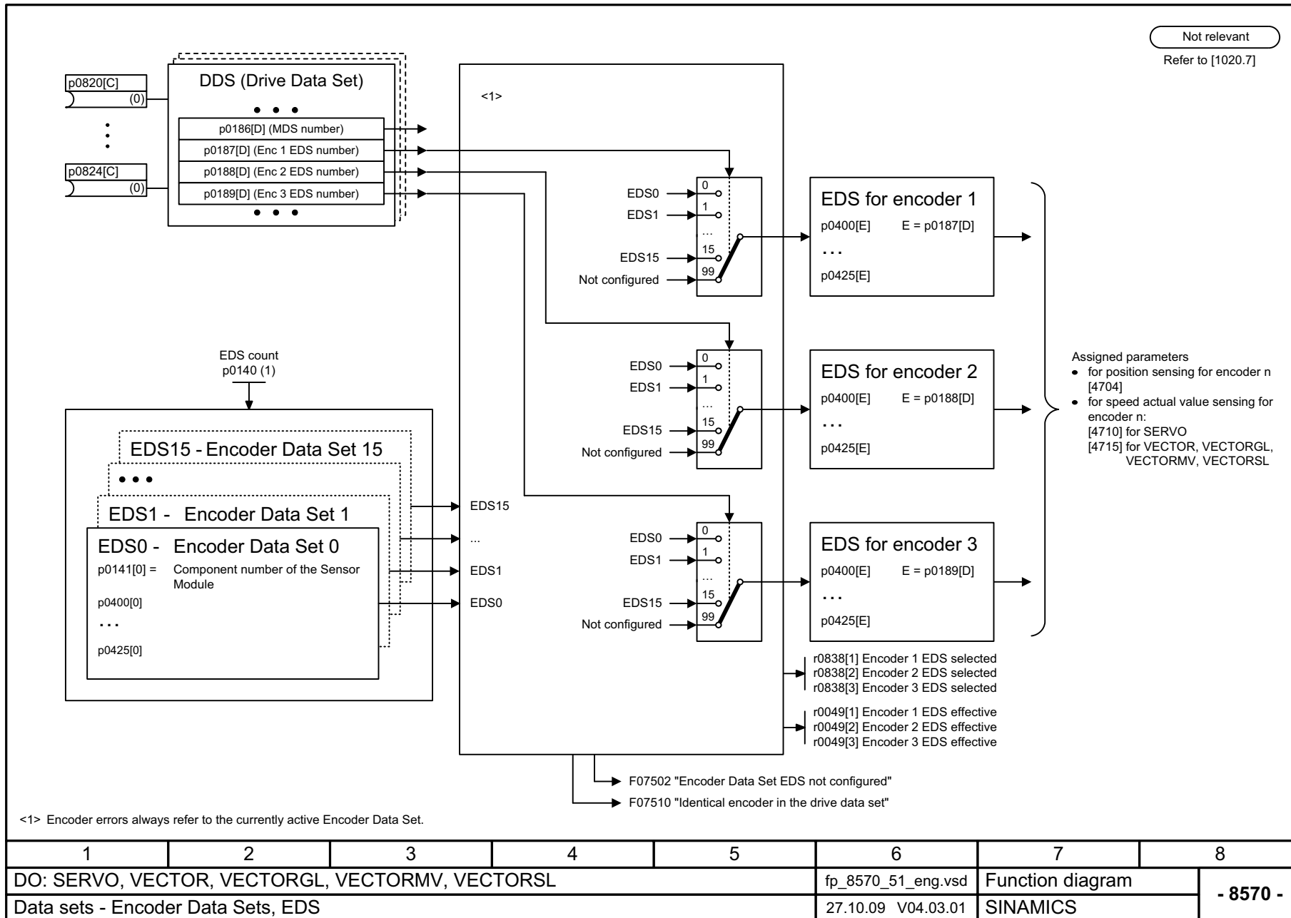
Fig. 2-131 8570 – Encoder data sets (EDS)
