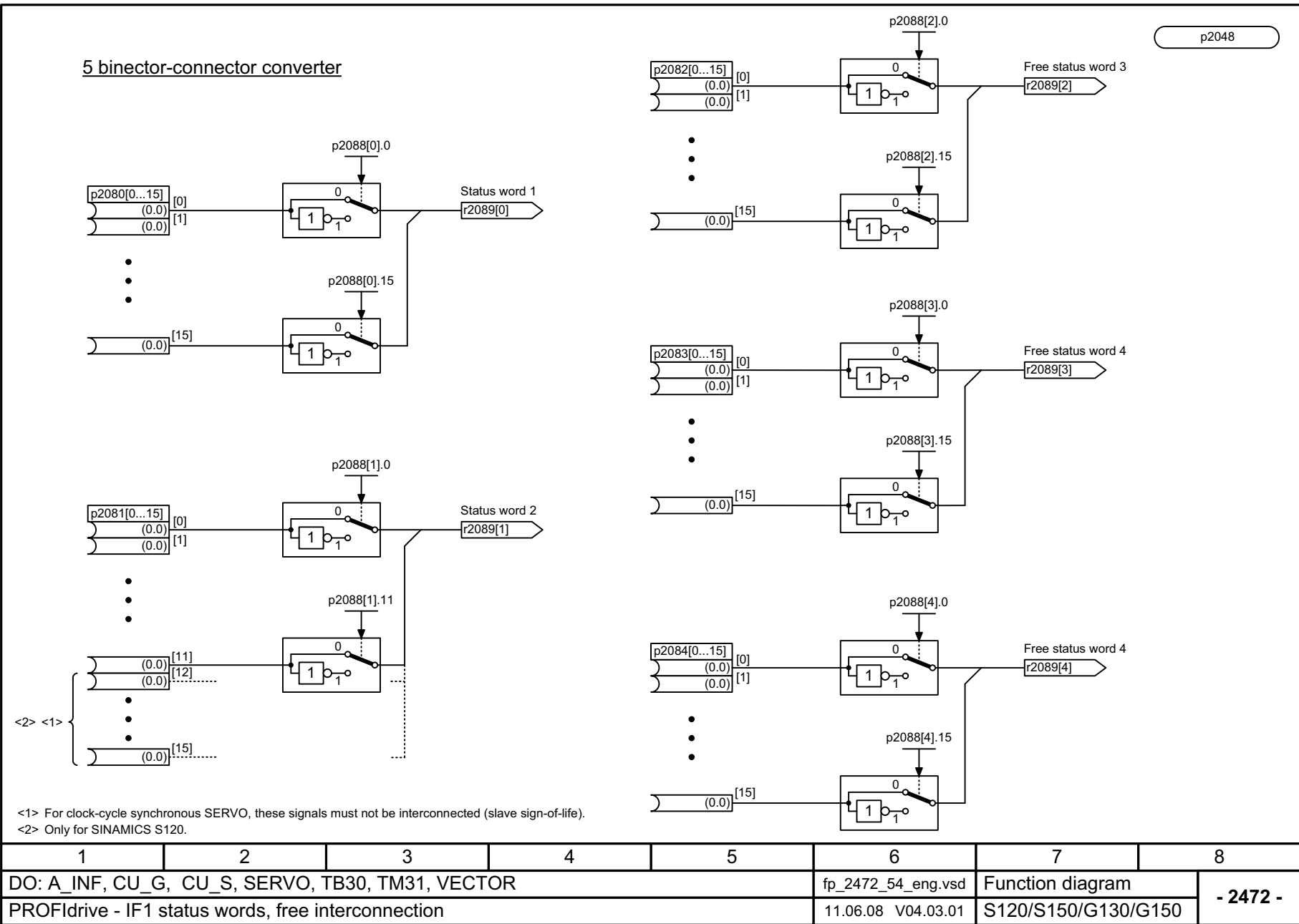
Fig. 2-42 2472 – IF1 status words, free interconnection
