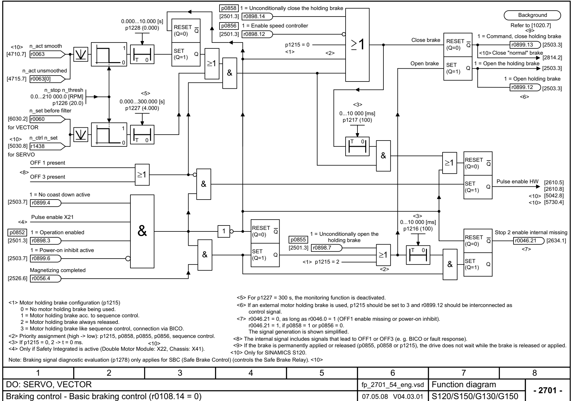
Fig. 2-66 2701 – Simple brake control (r0108.14 = 0)
