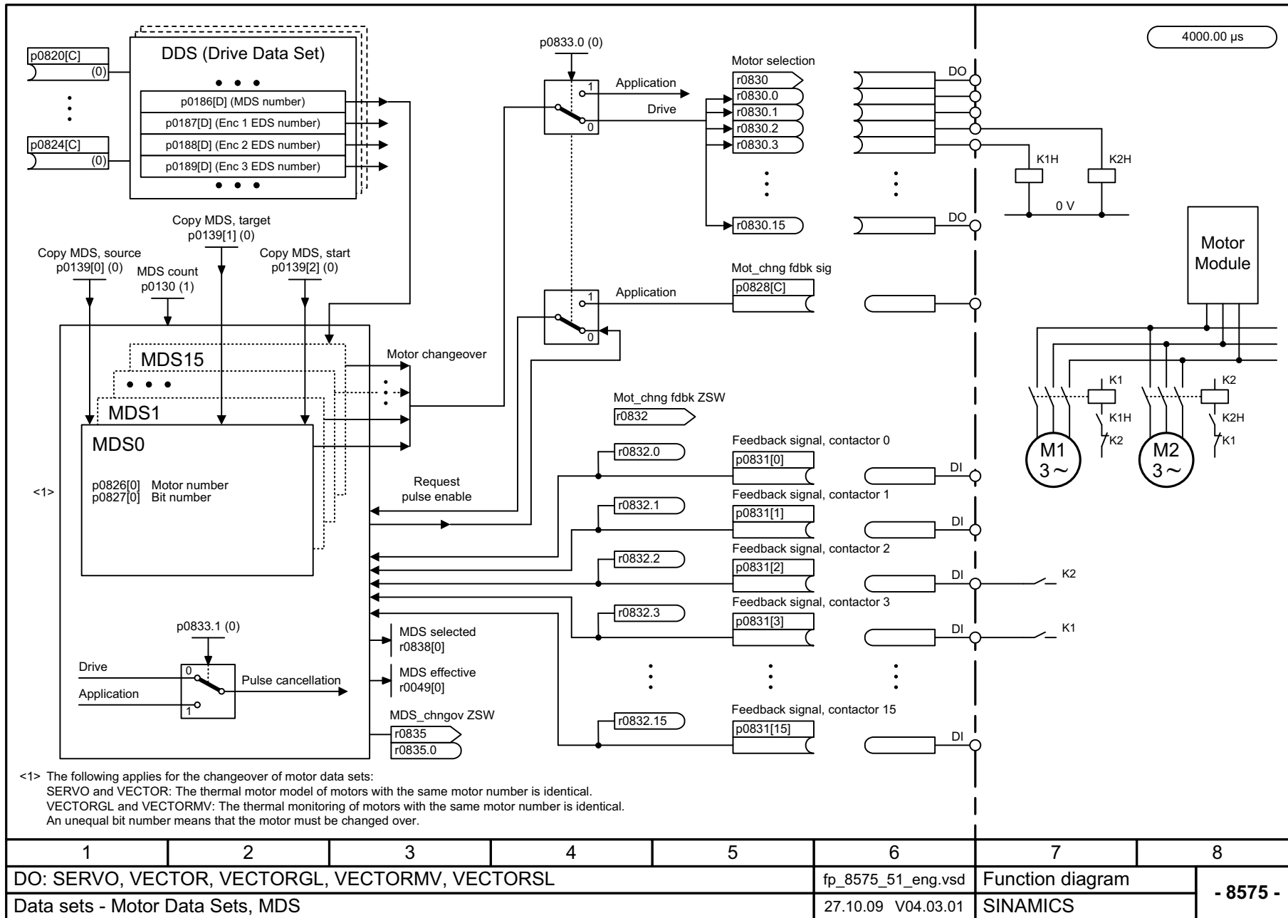
Fig. 2-132 8575 – Motor data sets (MDS)
