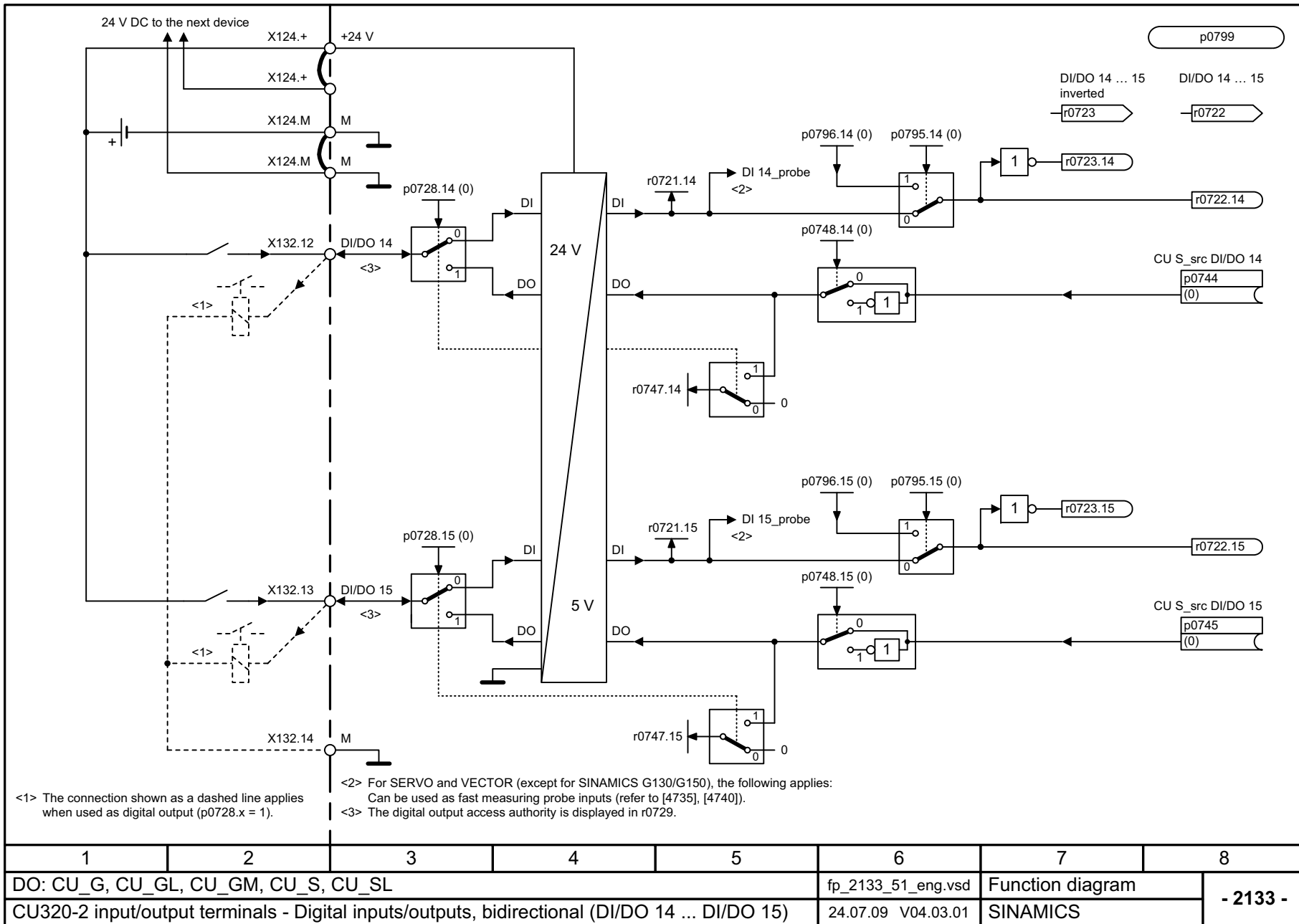
Fig. 2-21 2133 – Digital inputs/outputs, bidirectional (DI/DO 14 to DI/DO 15)
