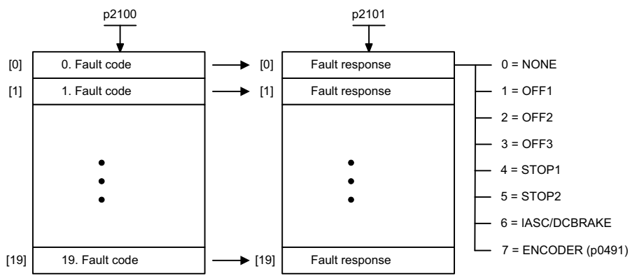
Fig. 2-127 8075 – Fault/alarm configuration
