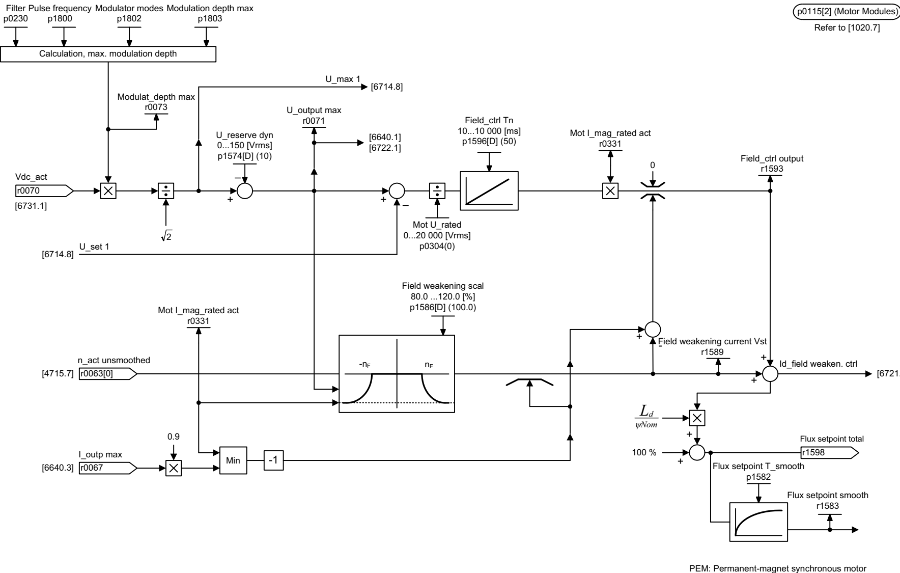
Fig. 2-103 6724 – Field weakening controller (PEM, p0300 = 2)
