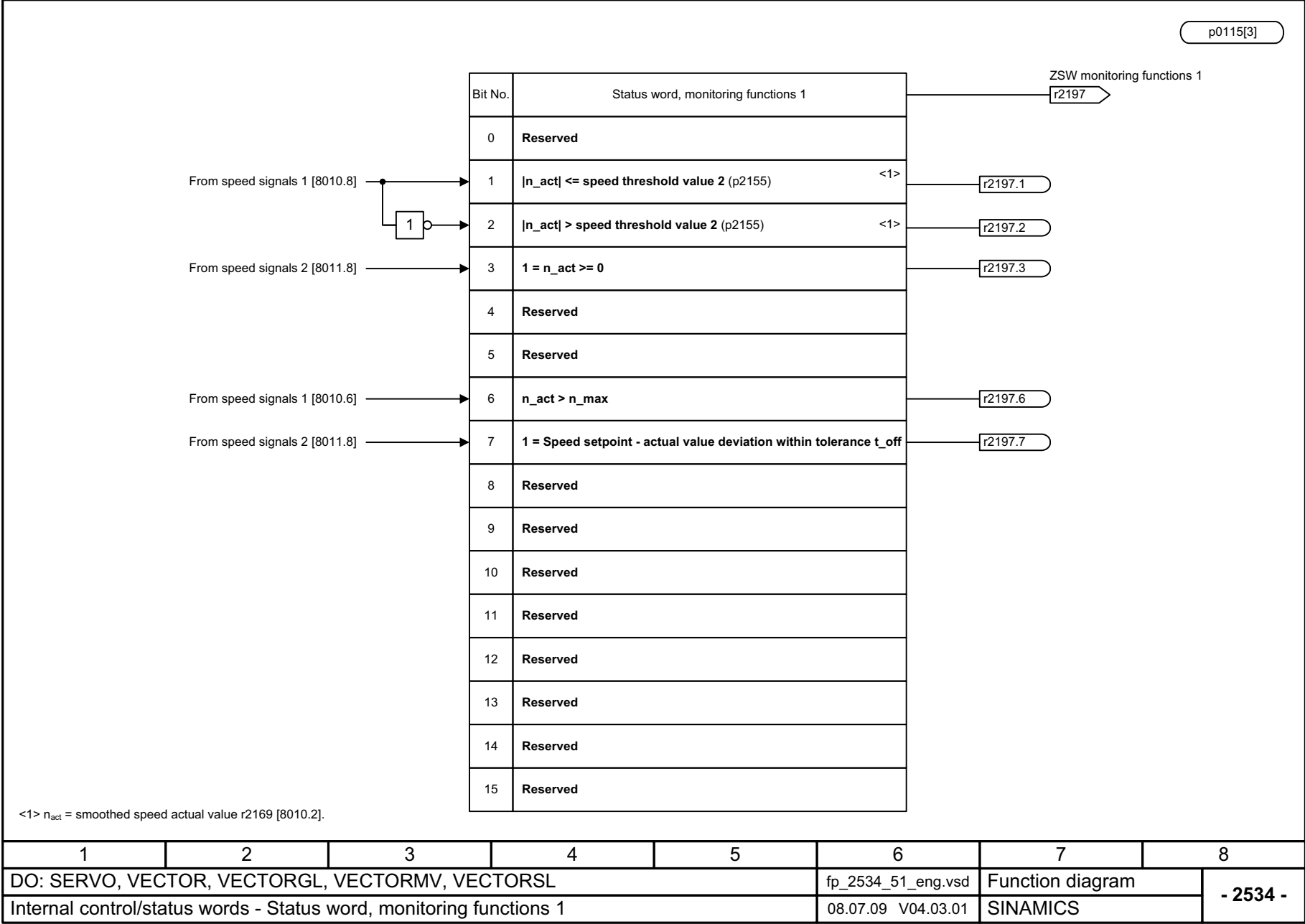
Fig. 2-59 2534 – Status word, monitoring functions 1
