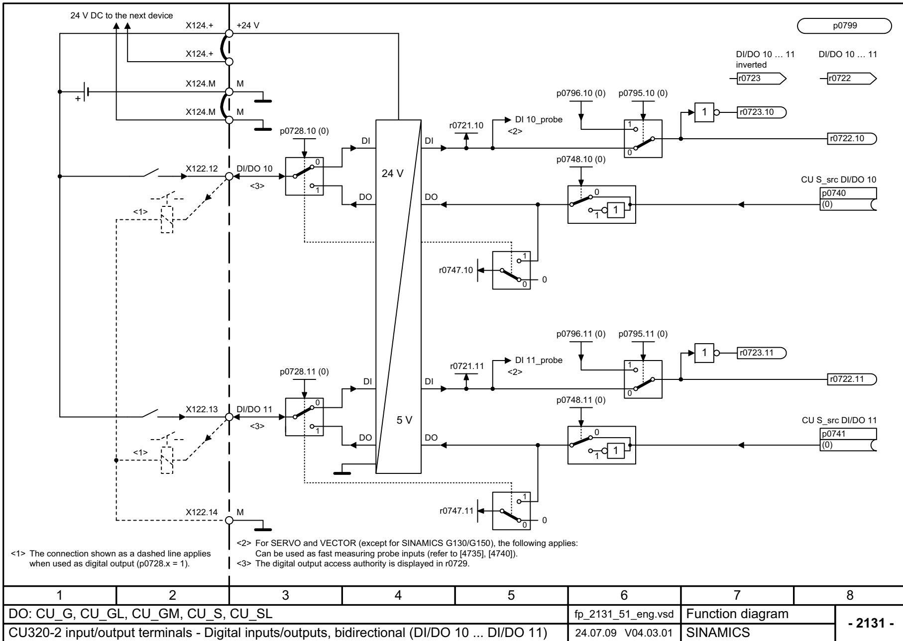
Fig. 2-19 2131 – Digital inputs/outputs, bidirectional (DI/DO 10 to DI/DO 11)
