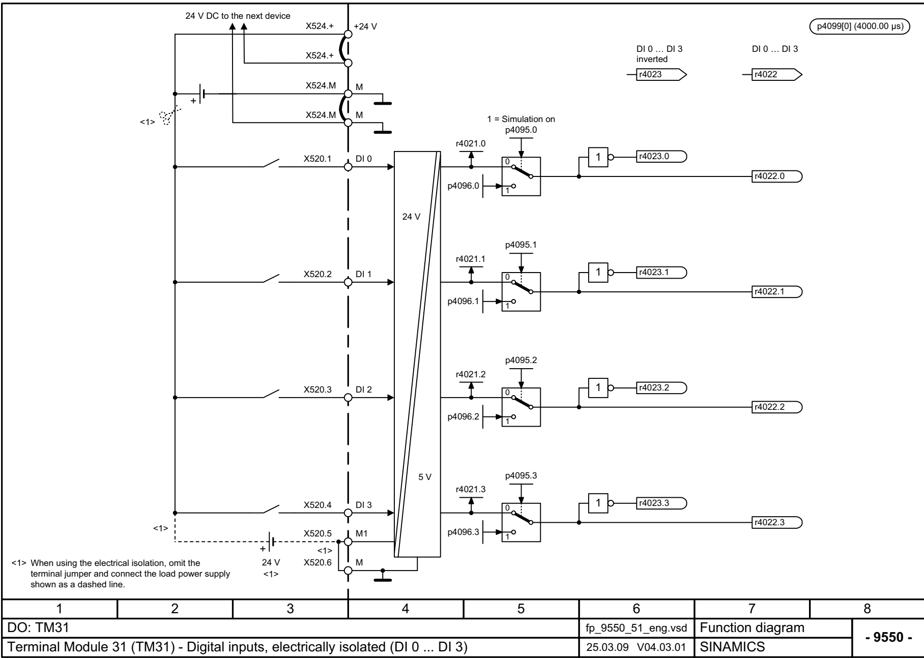
Fig. 2-144 9550 – Digital inputs, isolated (DI 0 to DI 3)
