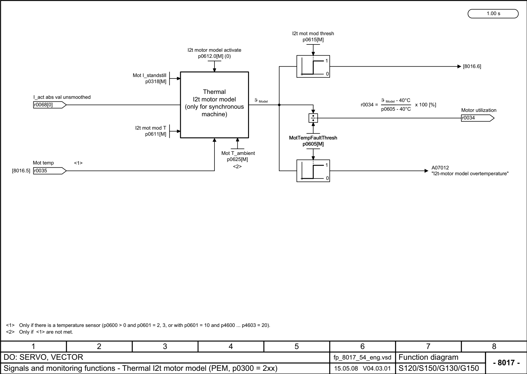
Fig. 2-123 8017 – Thermal I2t motor model (PEM, p0300 = 2xx)
