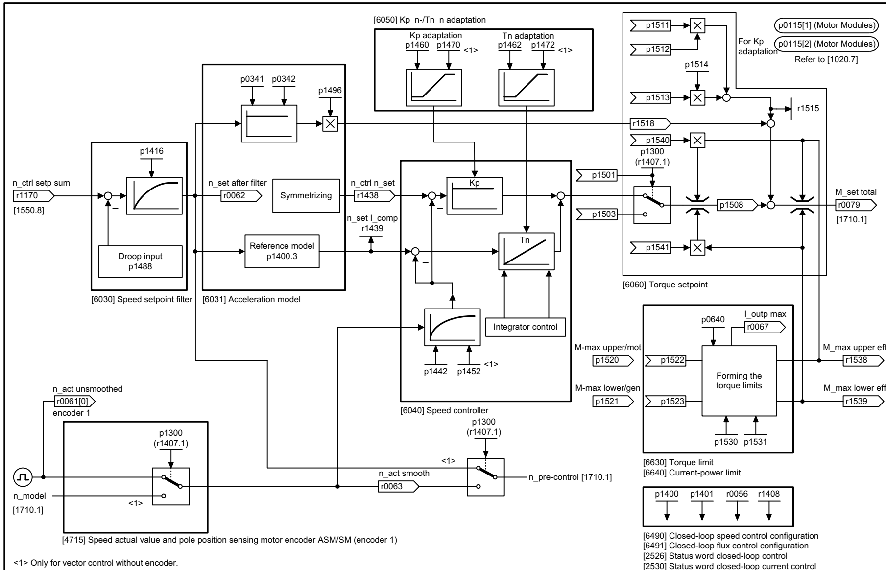
Fig. 2-11 1700 – Vector control, closed-loop speed control, and generation of torque limits
