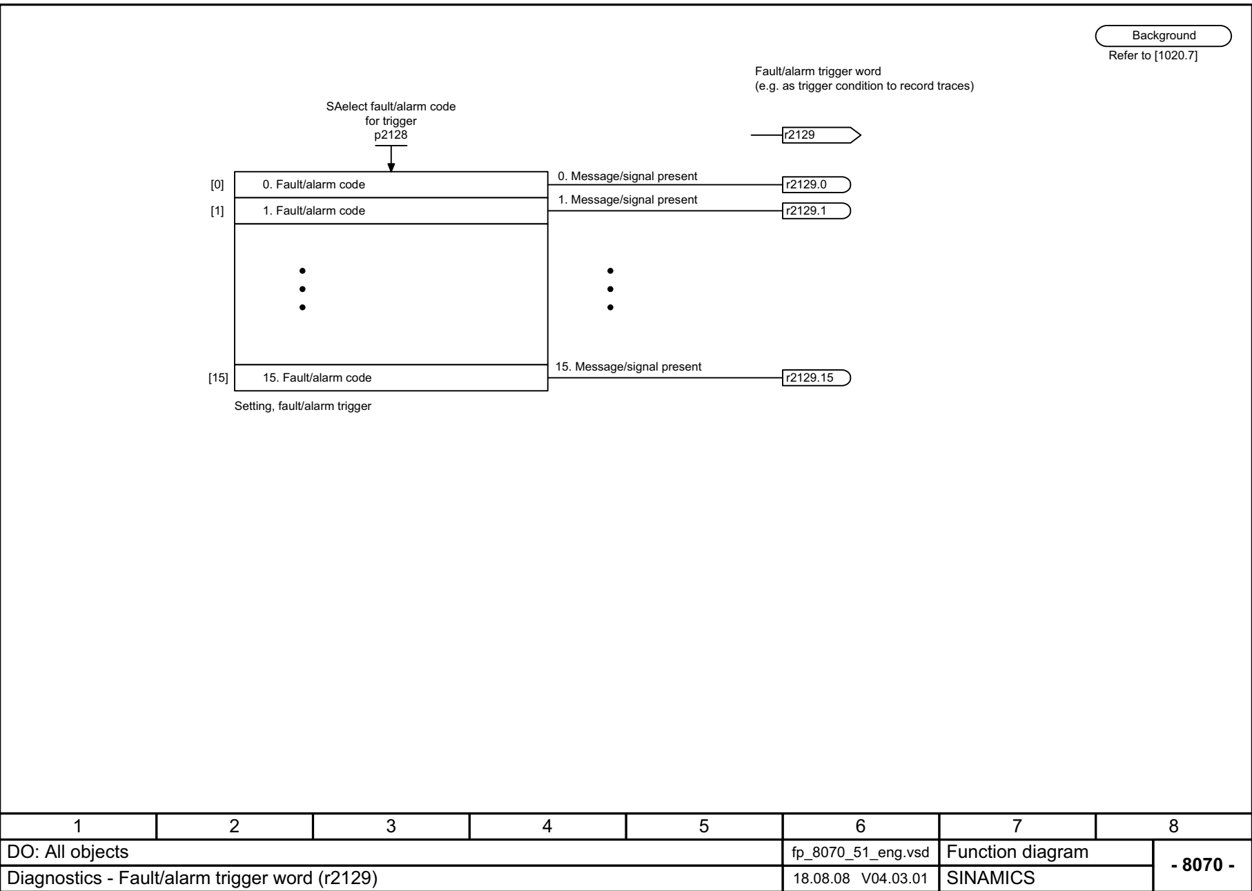
Fig. 2-126 8070 – Fault/alarm trigger word (r2129)
