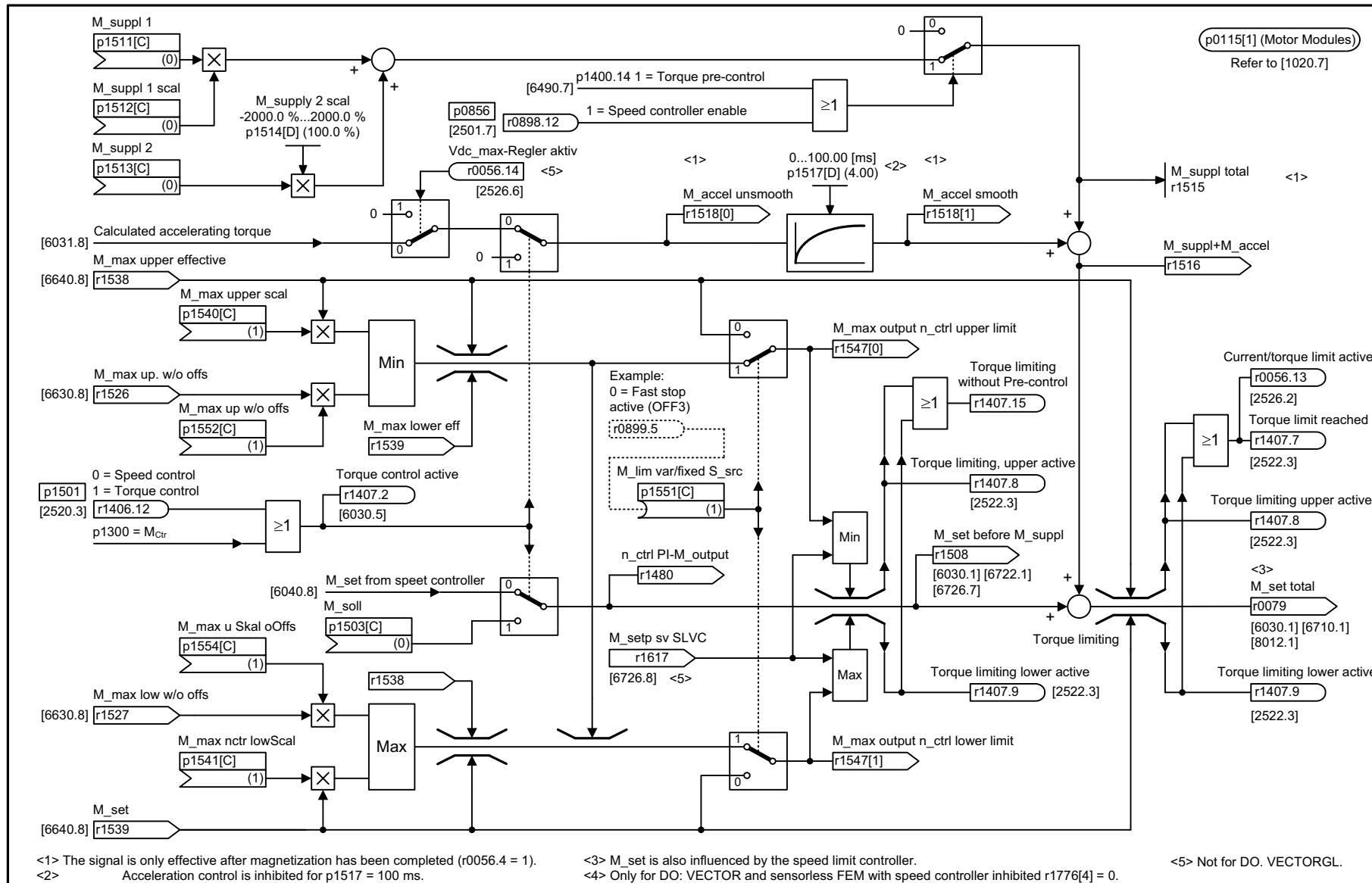
Fig. 2-89 6060 – Torque setpoint
