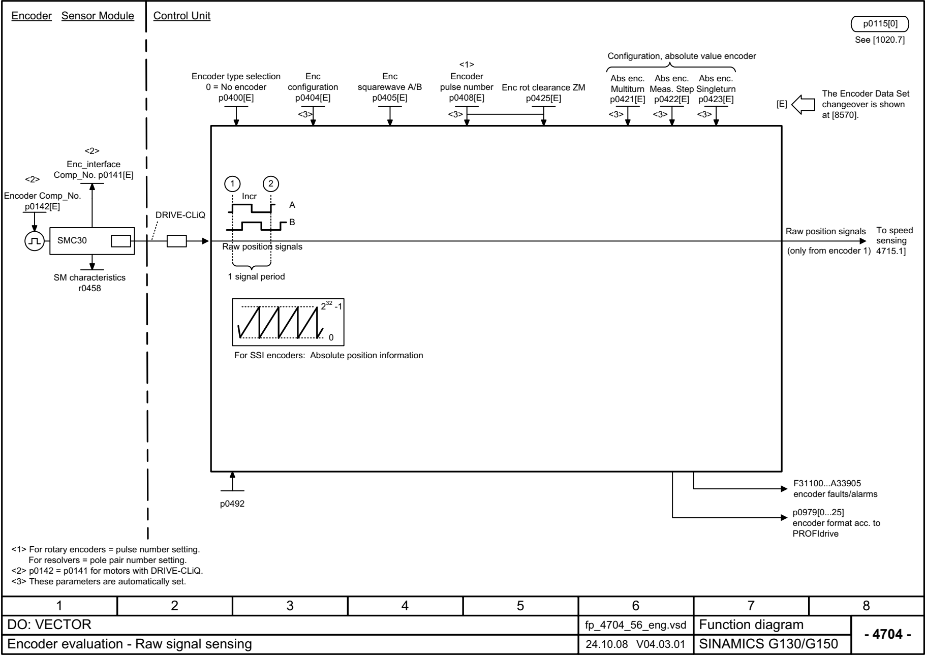
Fig. 2-83 4704 – Raw signal sensing
