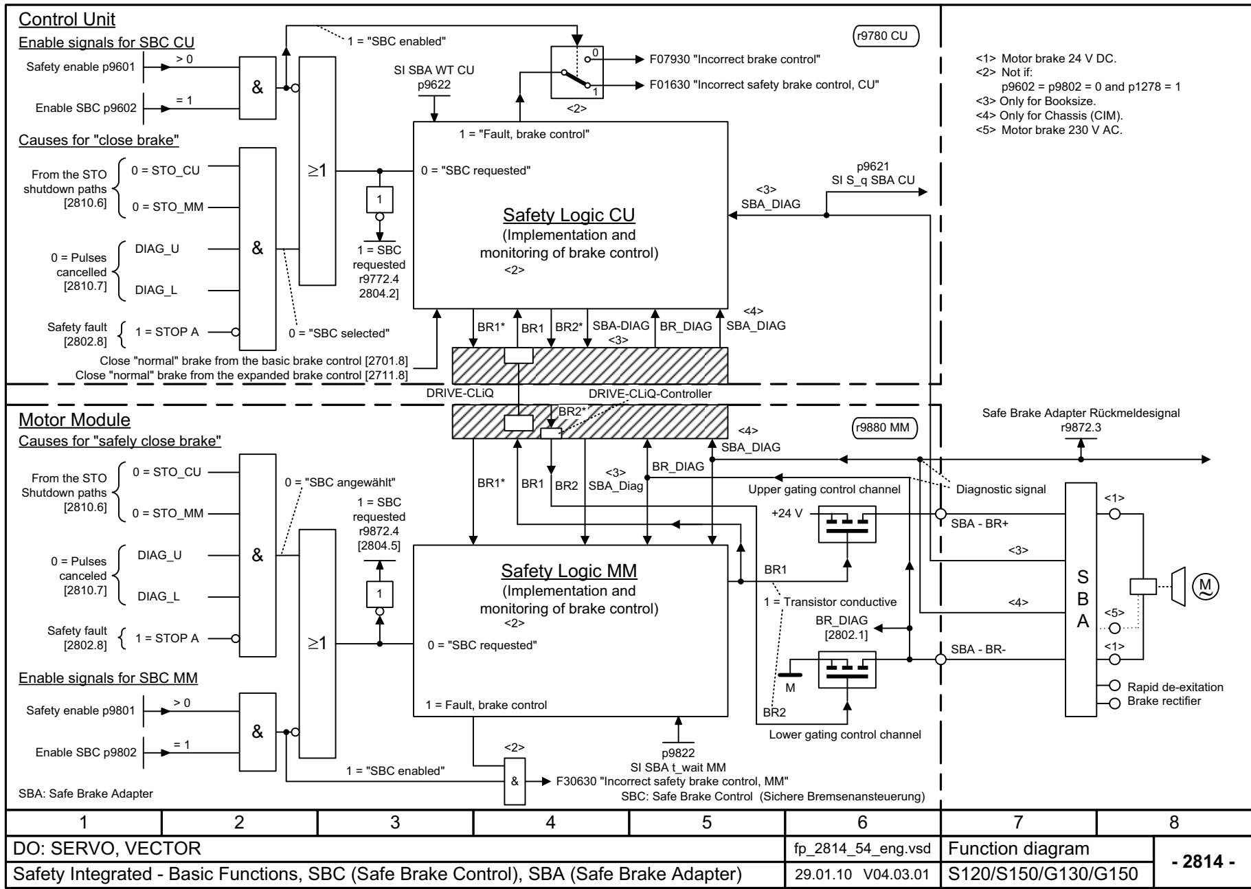
Fig. 2-74 2814 – Basic functions, SBC (Safe Brake Control), SBA (Safe Brake Adapter)
