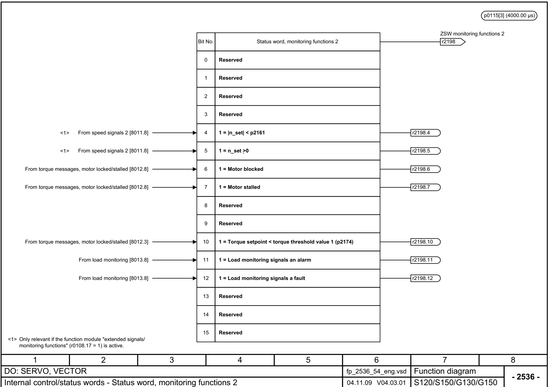
Fig. 2-60 2536 – Status word, monitoring functions 2
