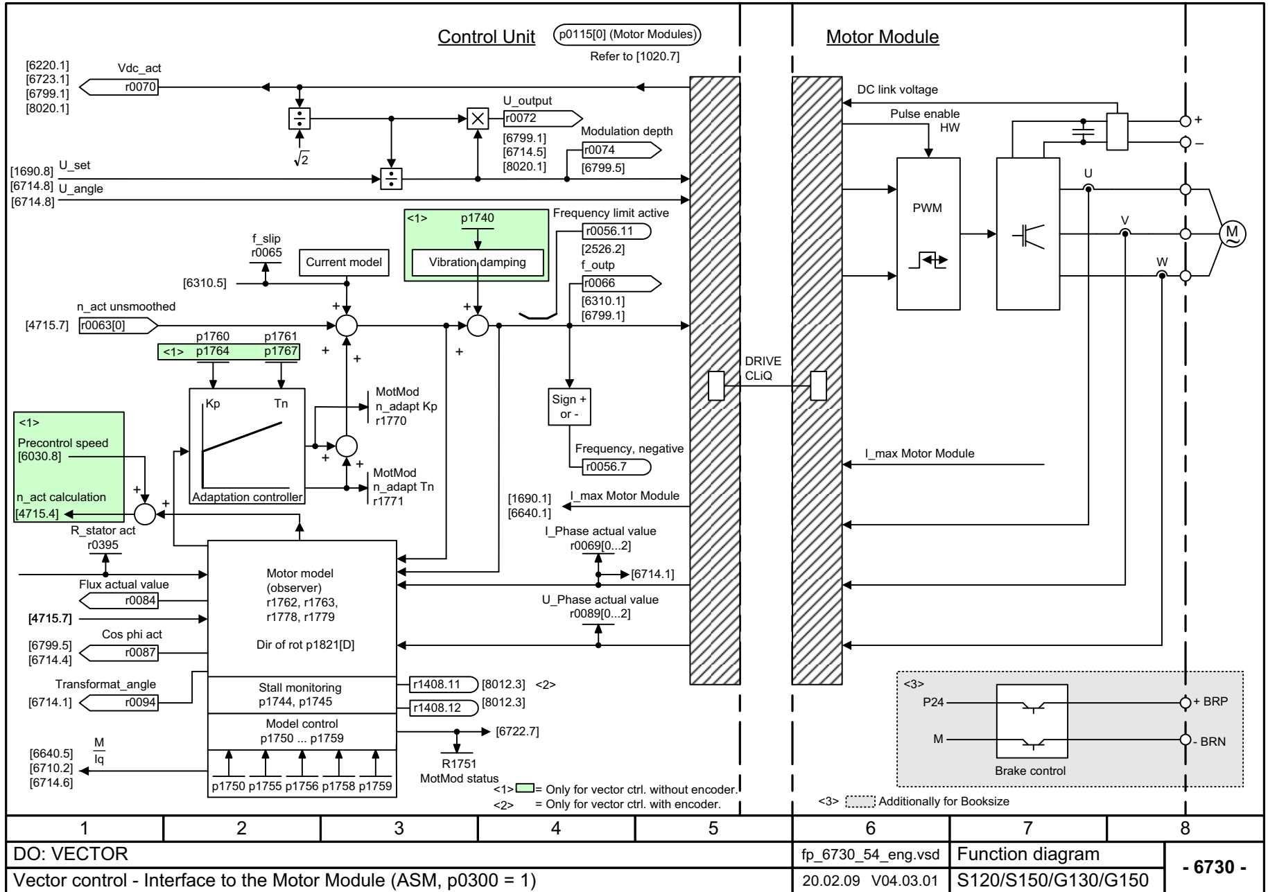
Fig. 2-104 6730 – Interface to Motor Module (ASM, p0300 = 1)
