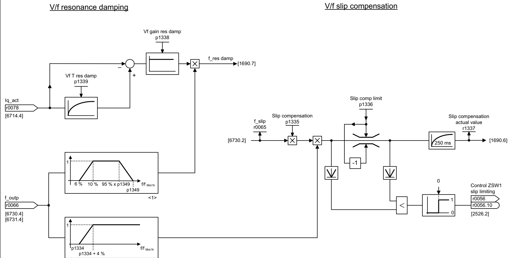
Fig. 2-92 6310 – Resonance damping and slip compensation
