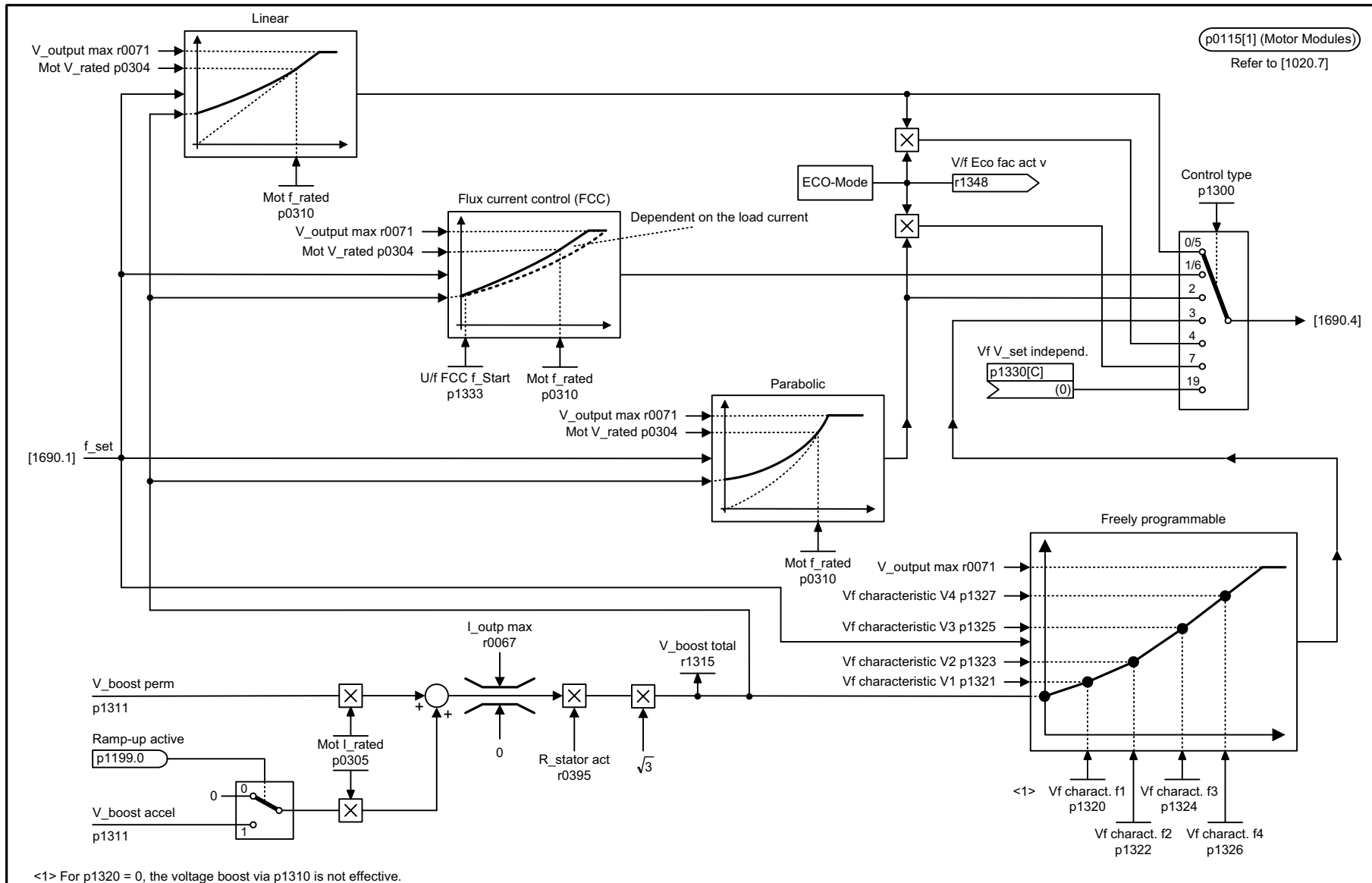
Fig. 2-91 6300 – V/f characteristic and voltage boost
