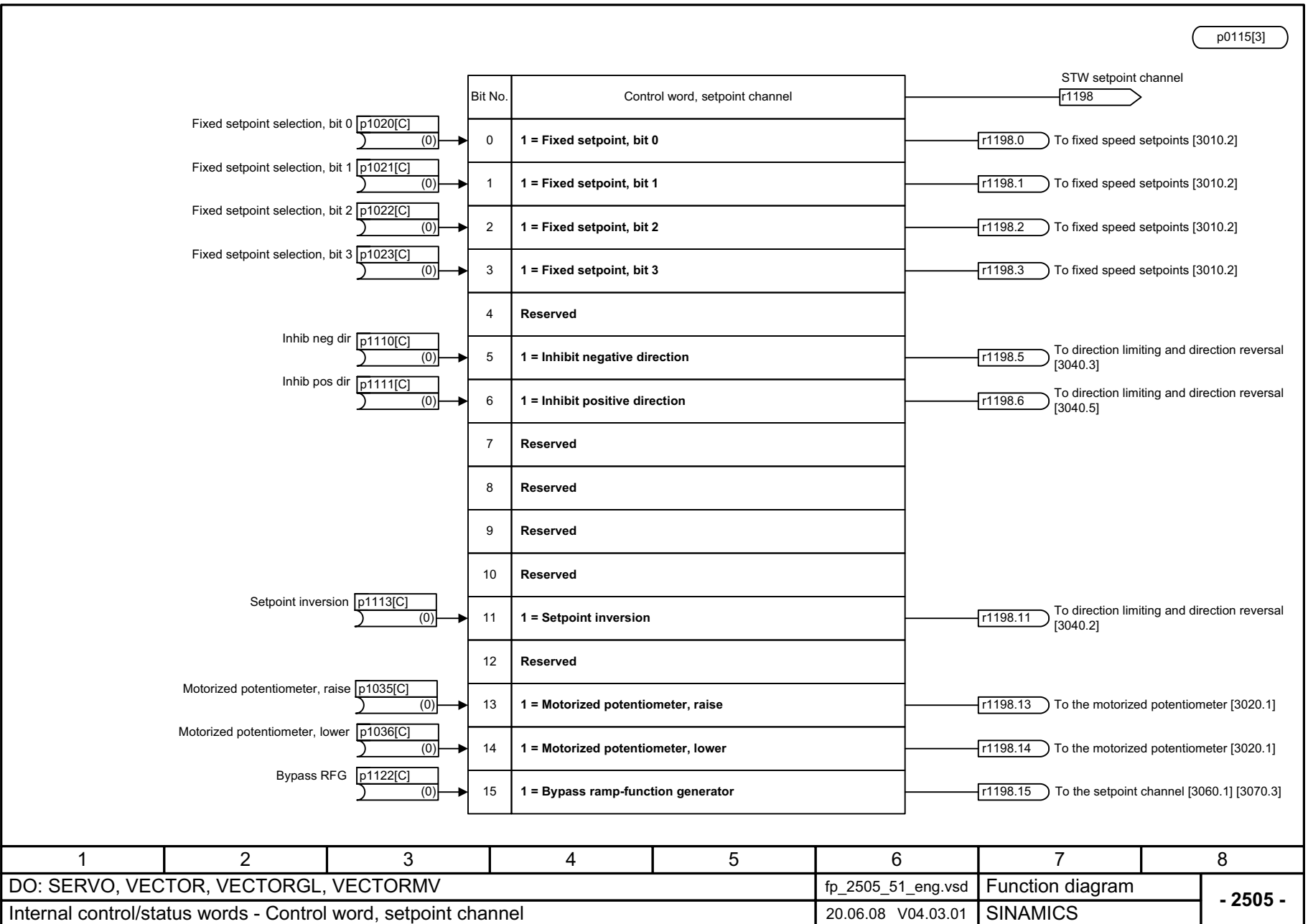
Fig. 2-54 2505 – Control word, setpoint channel
