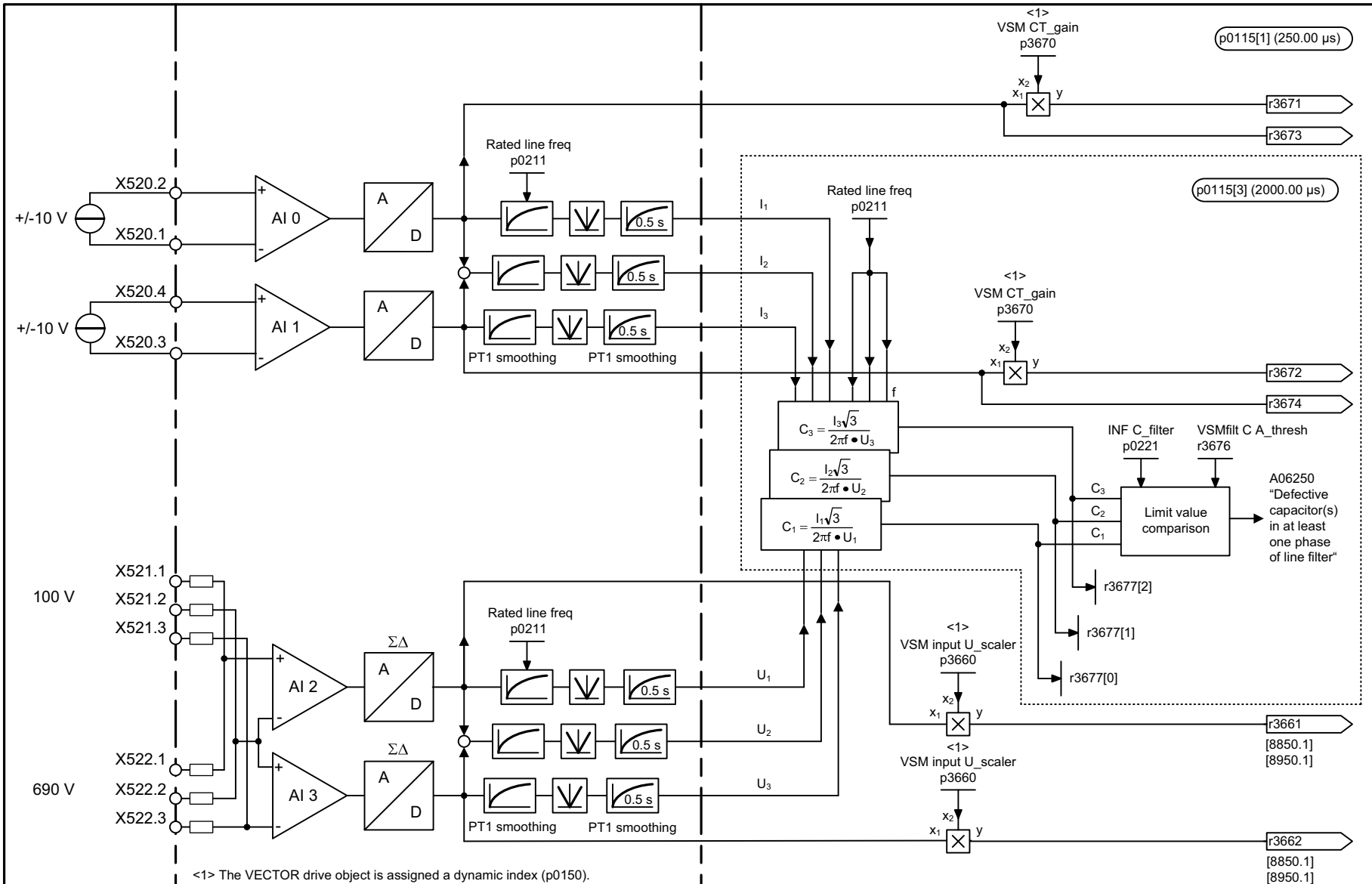
Fig. 2-154 9880 – Analog inputs (AI 0 to AI 3)
