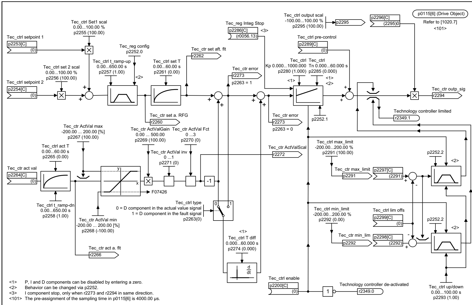
Fig. 2-115 7958 – Closed loop control (r0108.16 = 1)
