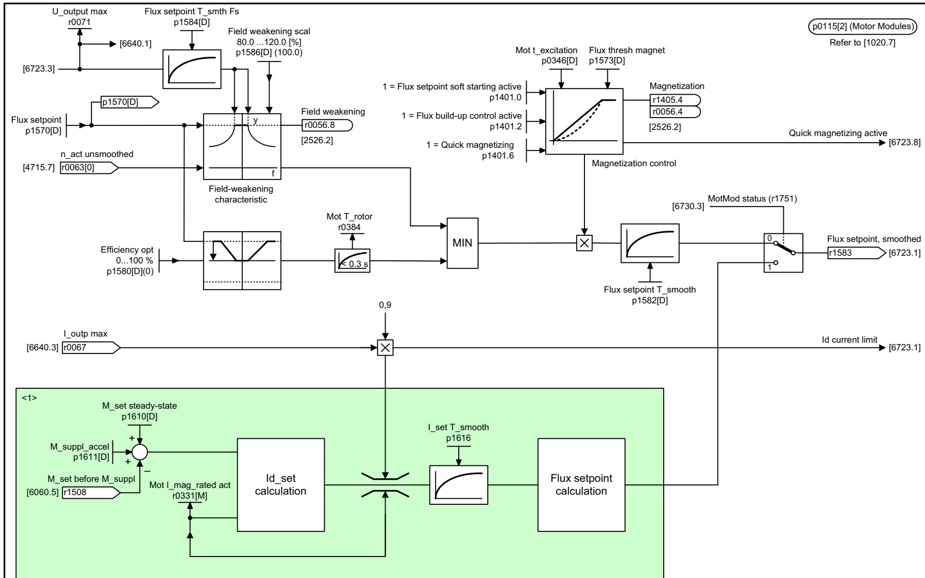
Fig. 2-101 6722 – Field weakening characteristic, Id setpoint (ASM, p0300 = 1)
