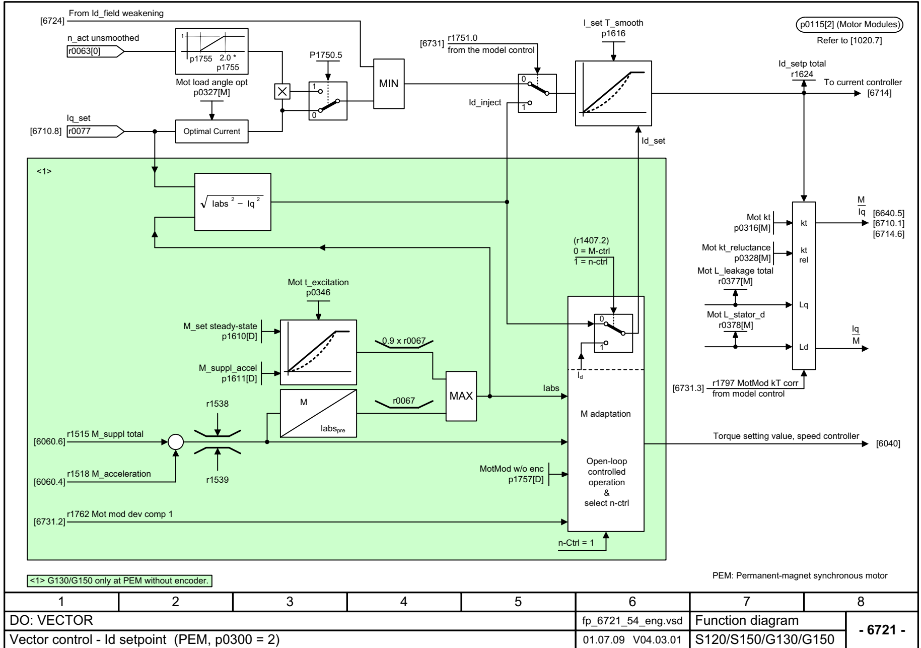
Fig. 2-100 6721 – Id setpoint (PEM, p0300 = 2)
