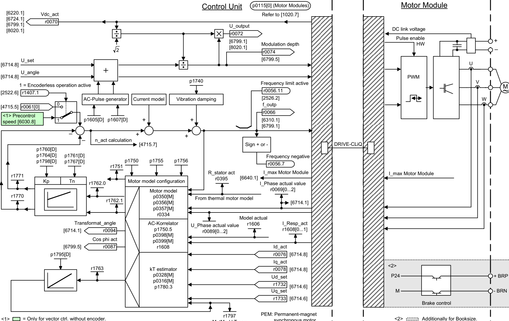
6731 – Interface to the Motor Module (PEM, p0300 = 2)
