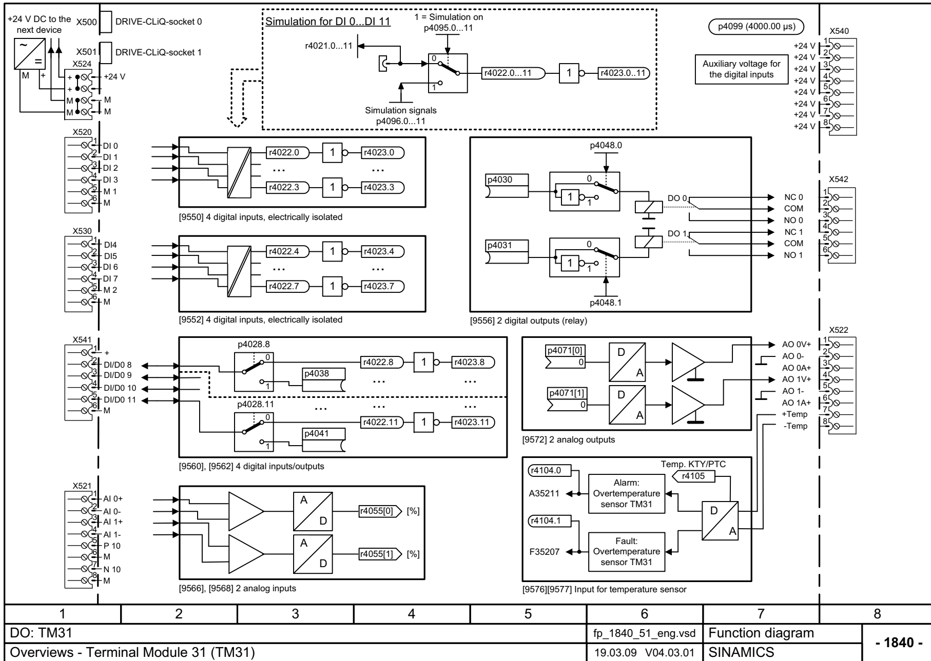
Fig. 2-15 1840 – Terminal Module 31 (TM31)
