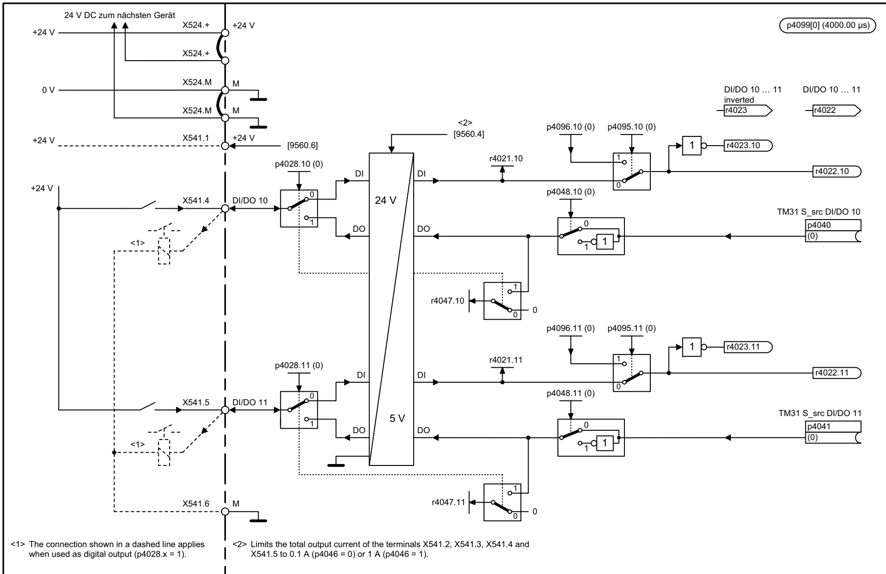
Fig. 2-148 9562 – Digital inputs/outputs, bidirectional (DI/DO 10 to DI/DO 11)
