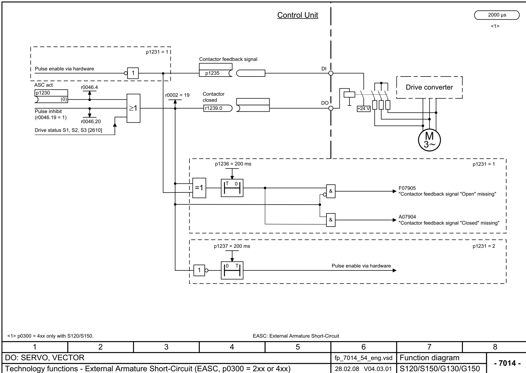
Fig. 2-108 7014 – External armature short-circuit (EASC, p0300 = 2xx)
