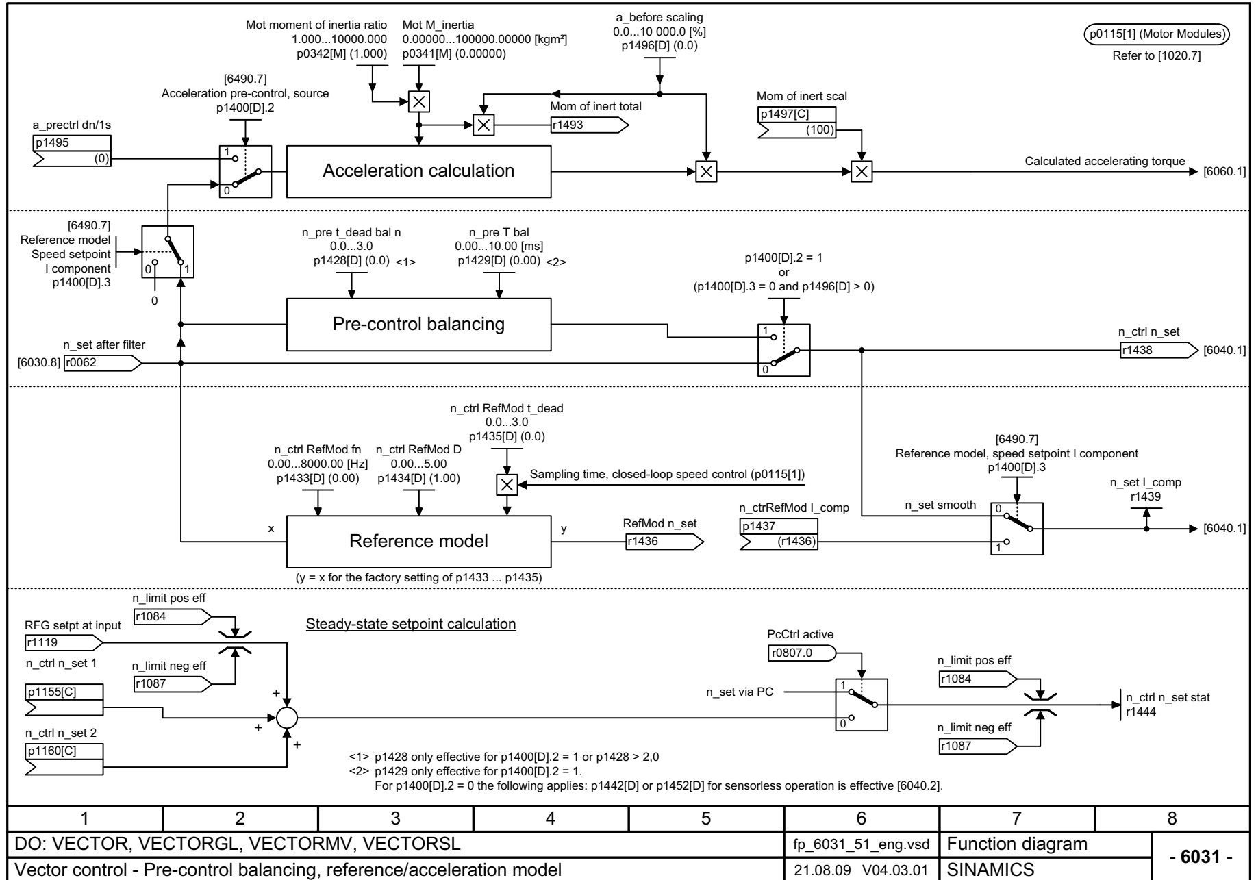
Fig. 2-86 6031 – Pre-control balancing for reference/acceleration model
