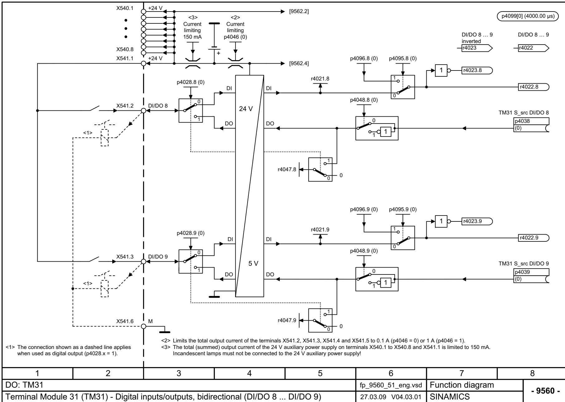
Fig. 2-147 9560 – Digital inputs/outputs, bidirectional (DI/DO 8 to DI/DO 9)
