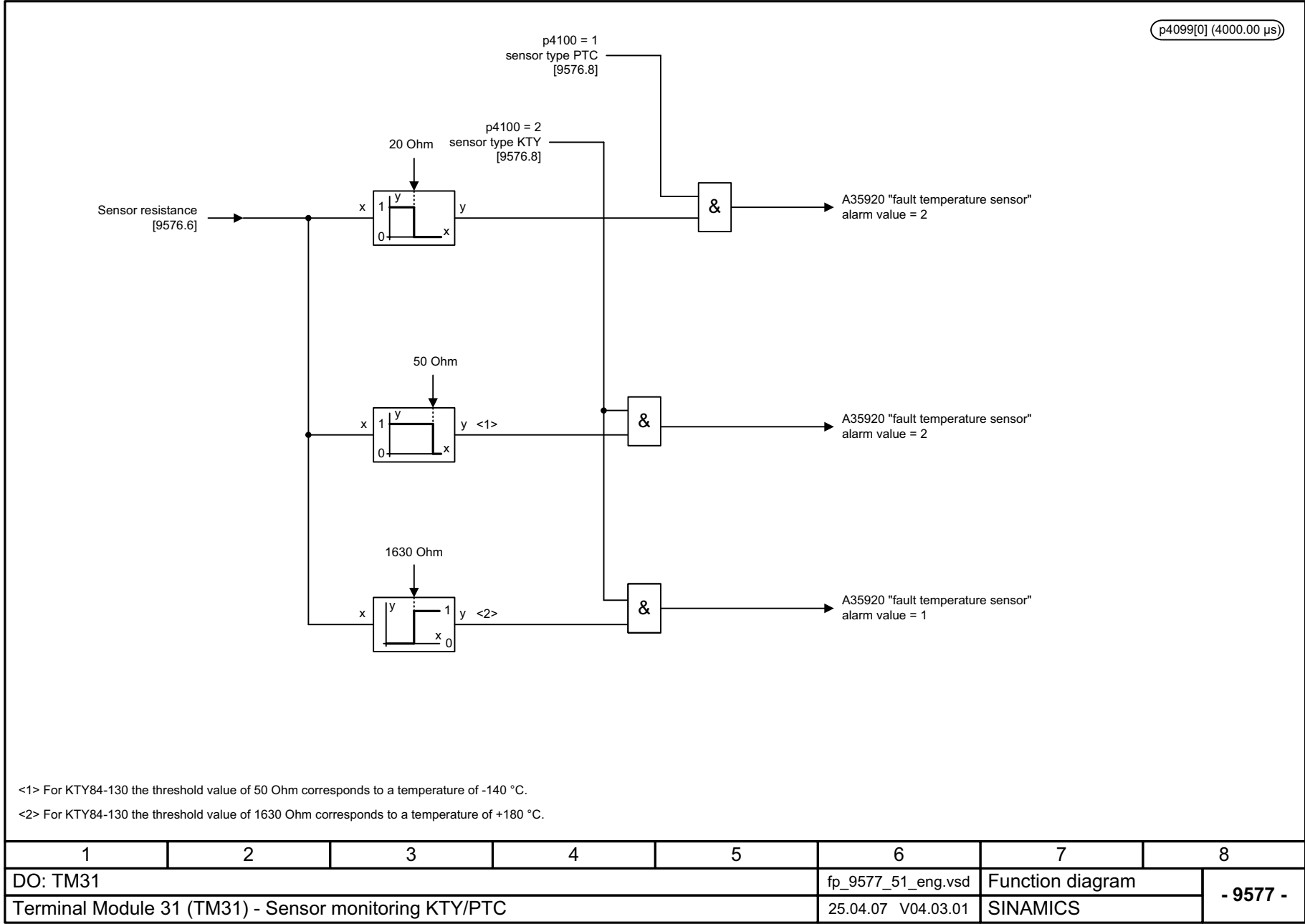
Fig. 2-153 9577 – Sensor monitoring KTY/PTC
