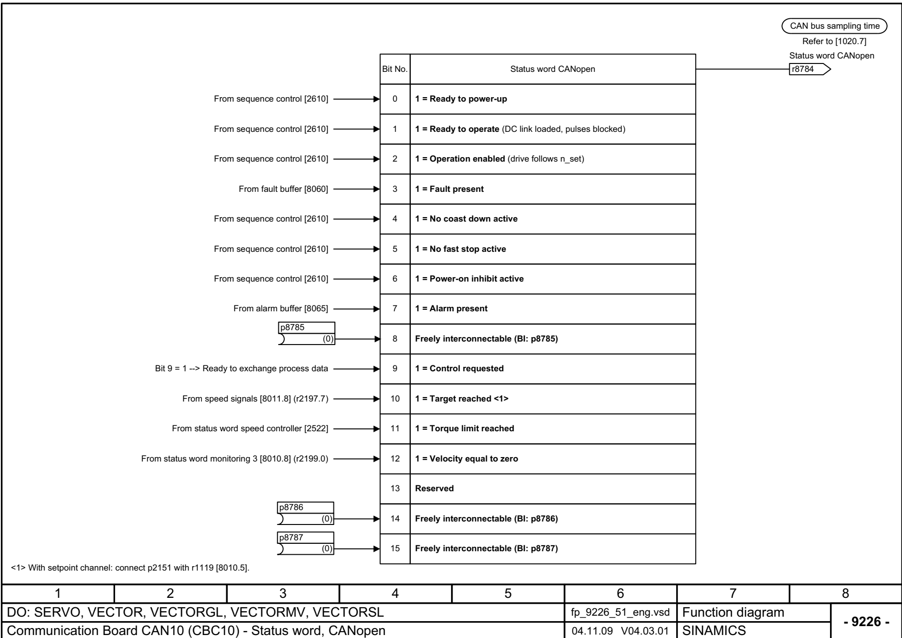
Fig. 2-143 9226 – Status word CANopen
