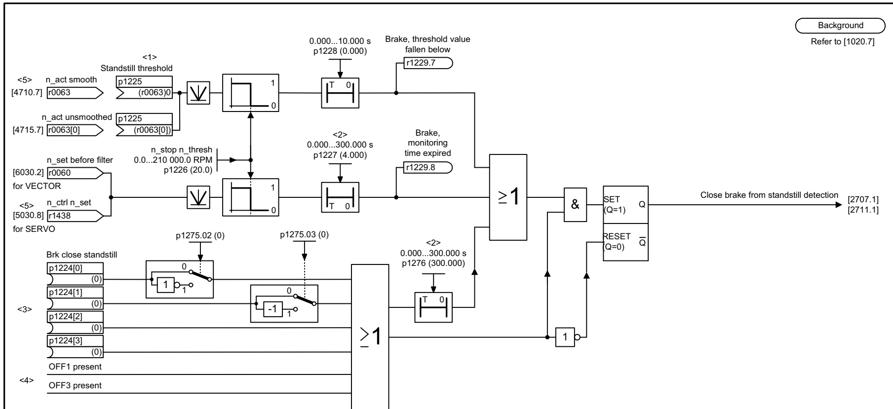
Fig. 2-67 2704 – Extended brake control, zero speed detection (r0108.14 = 1)
