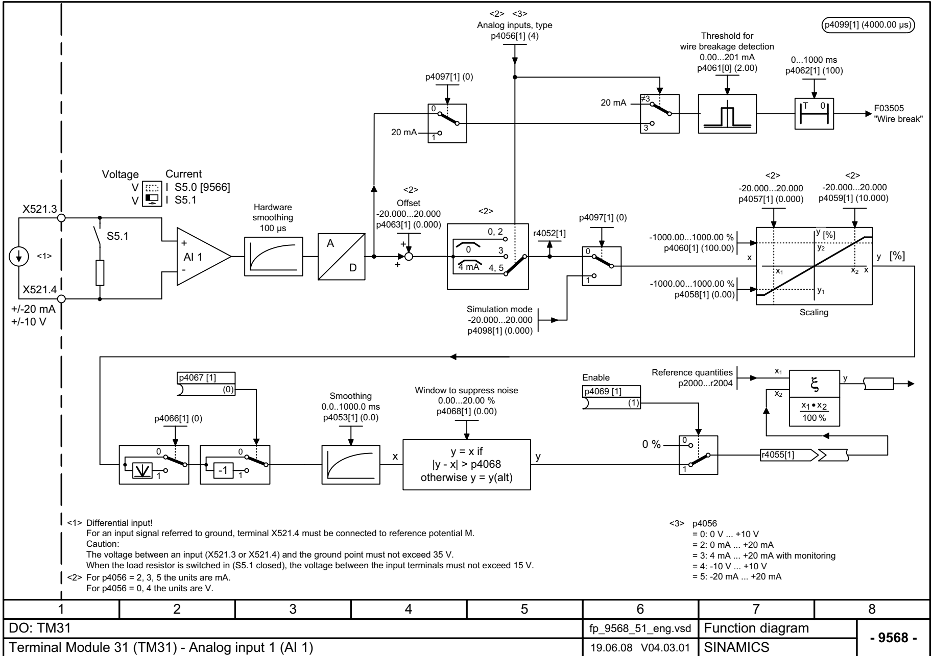
Fig. 2-150 9568 – Analog input 1 (AI 1)
