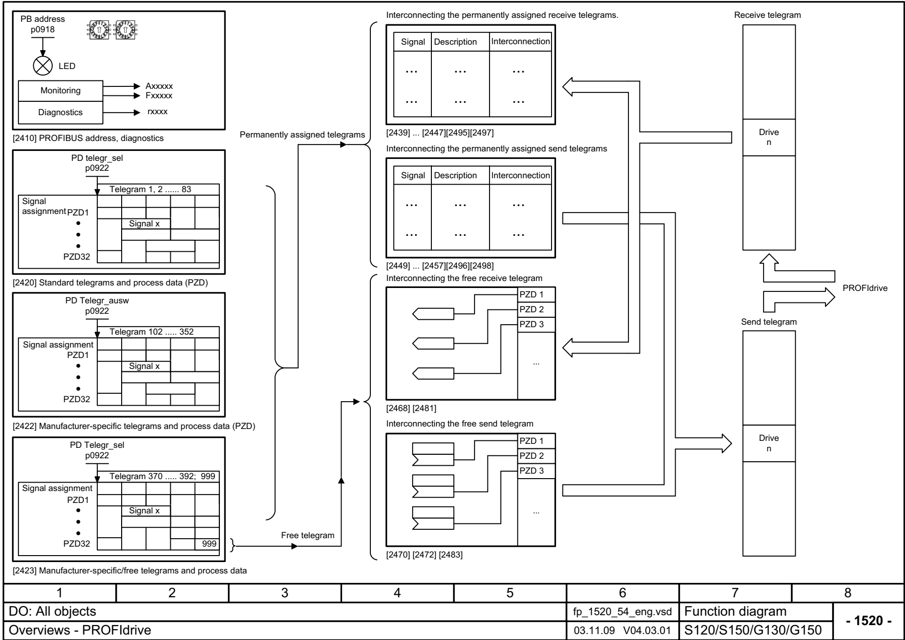
Fig. 2-6 1520 – PROFIdrive
