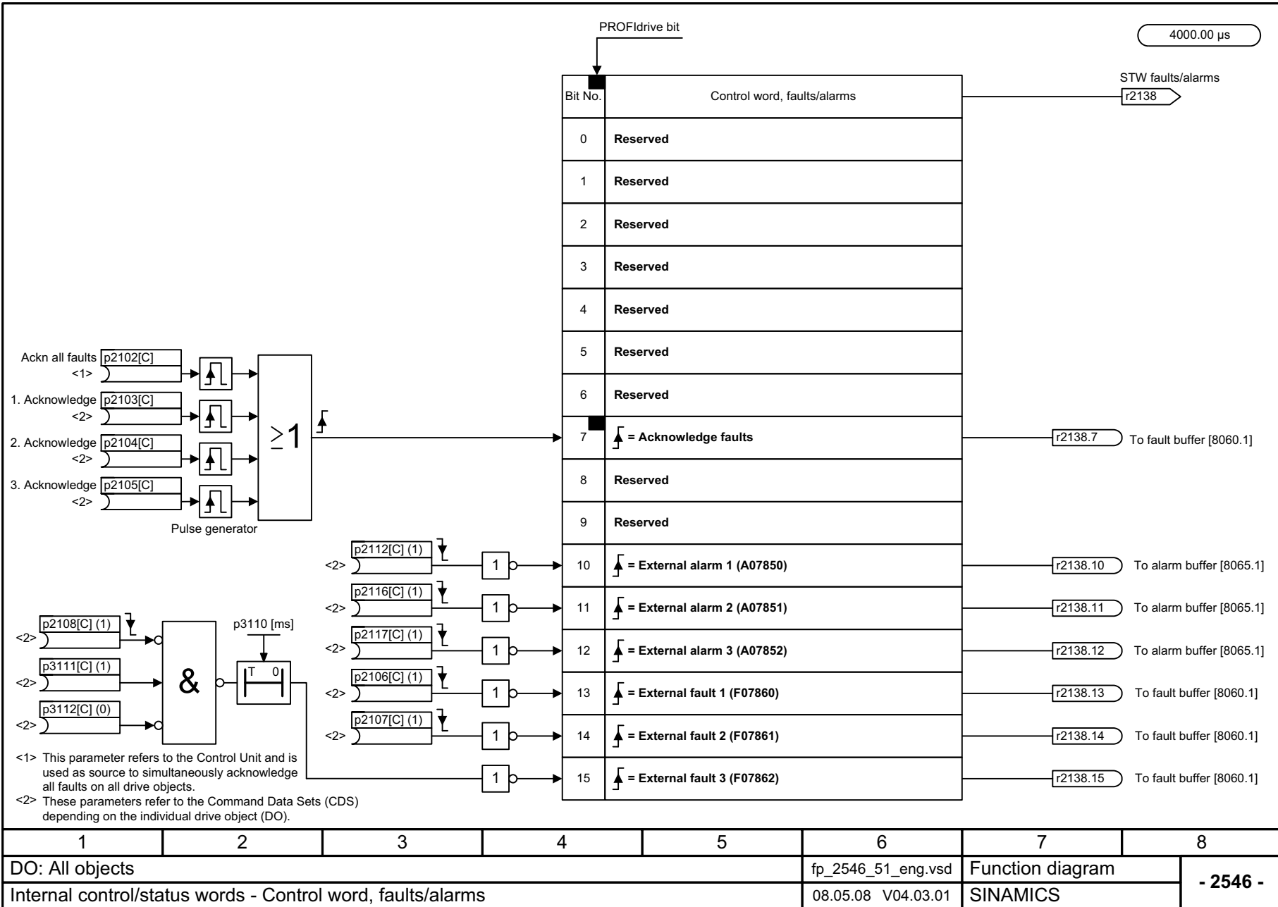
2546 – Control word, faults/alarms
