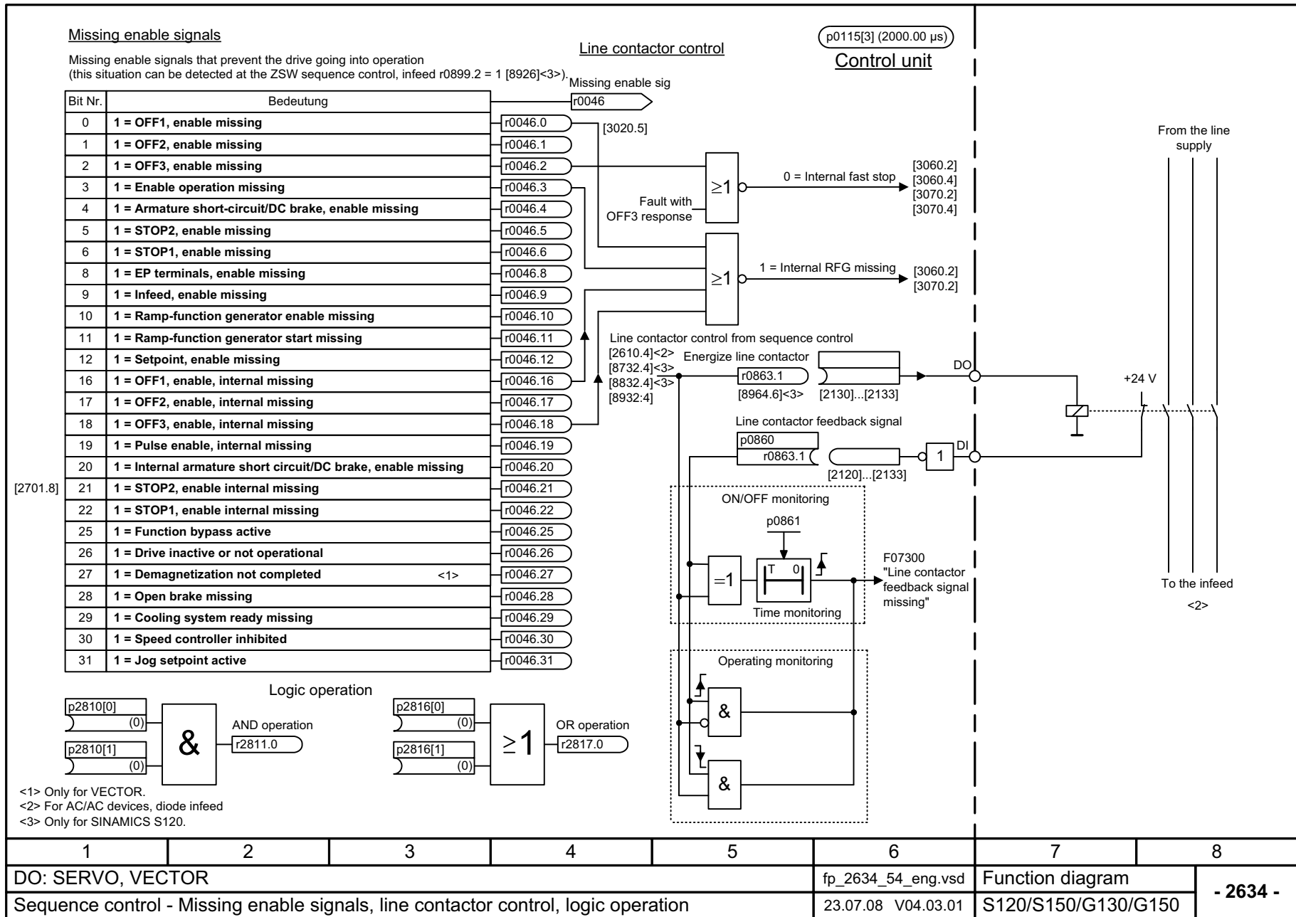
Fig. 2-65 2634 – Missing enable signals, line contactor control, logic operation
