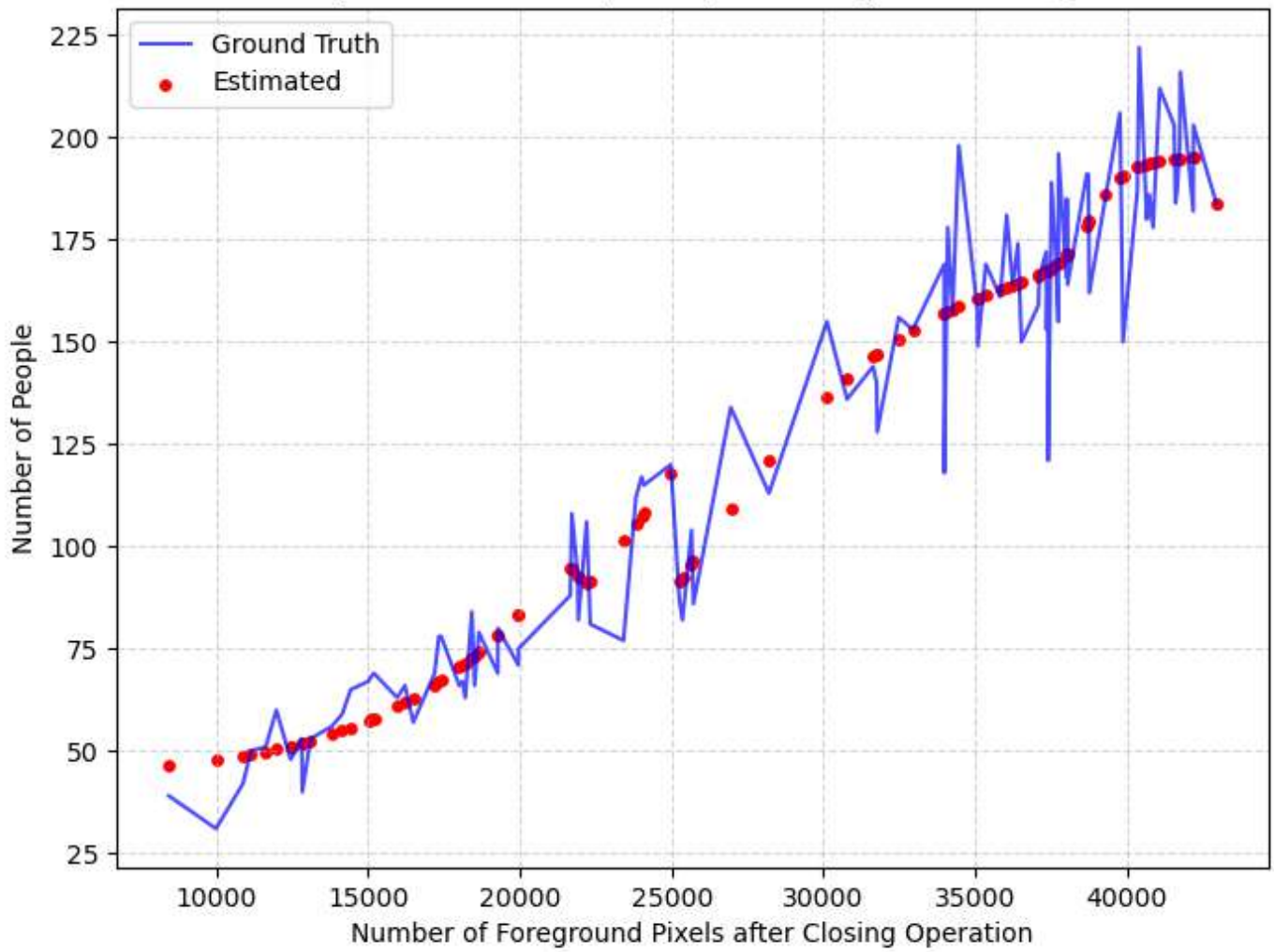
Figure 9: Method 2 (disk-5) - Training Relationship
