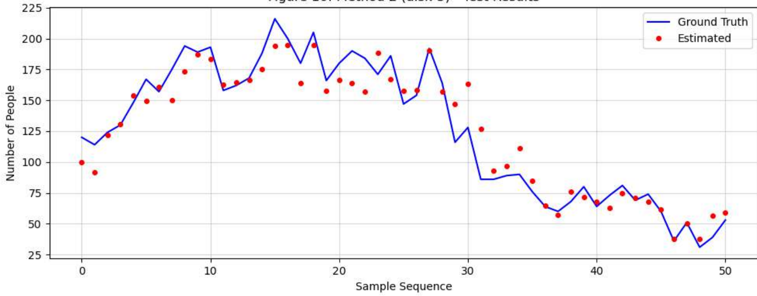
Figure 10: Method 2 (disk-5) - Test Results
