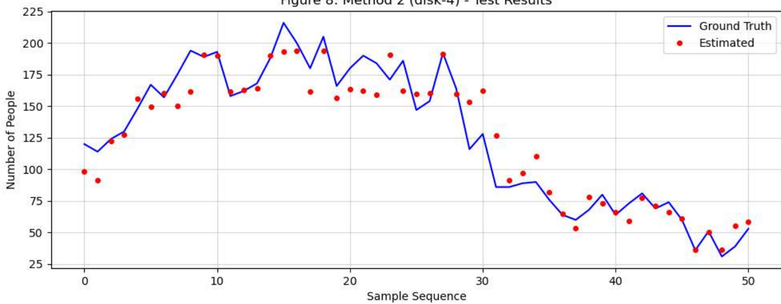
Figure 8: Method 2 (disk-4) - Test Results
