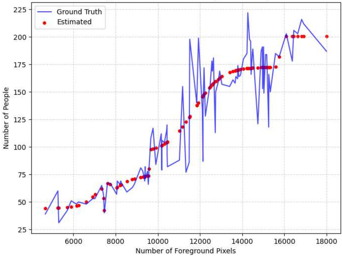
Figure 5: Method 1 - Training Relationship
