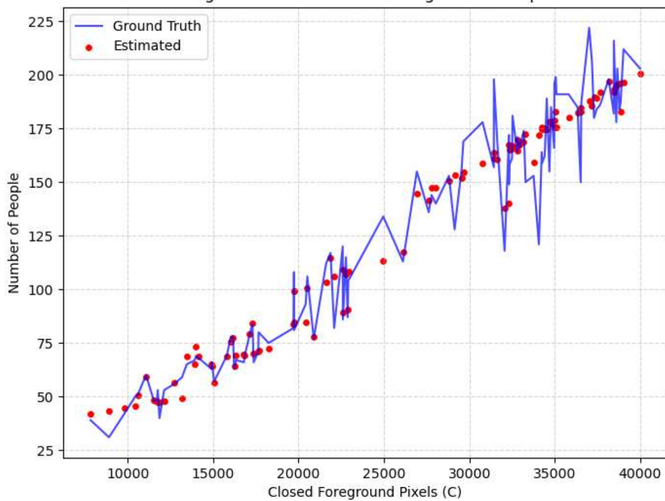
Figure 11: Method 3 - Training Relationship
