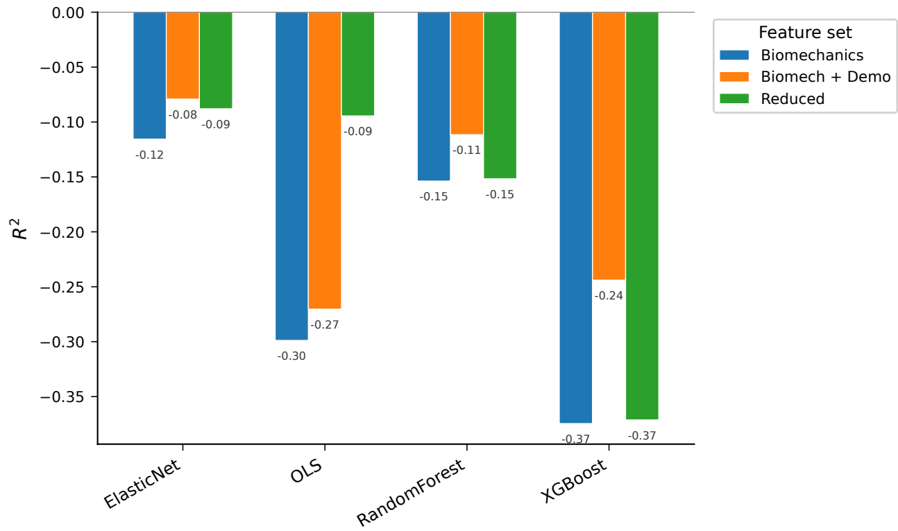
Cross-validated R^2 : CSIA J_{45} Component
