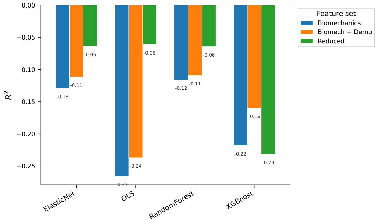
Cross-validated R^2 : CSIA Magnitude
