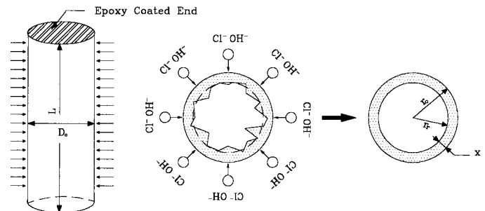
FIG. 4. Diffusion of \text{Cl}^- and \text{OH}^- Free Ions from Alkaline, Acidic, and Salt Solutions
