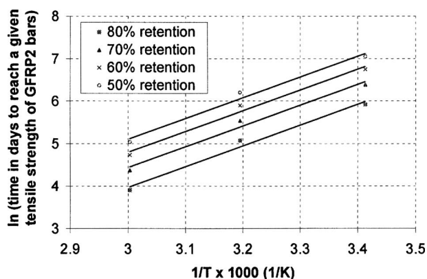
Fig. 8. Arrhenius plots of tensile strength degradation for GFRP2 bars exposed to Solution 2
