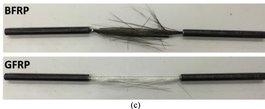
Fig. 2. Tensile specimens: (a) reference/intact specimen; (b) typical FRP bars under test and (c) specimens after test.
