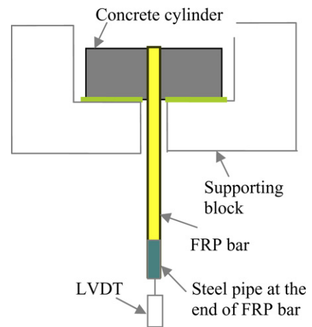
Fig. 7. Experimental setup for pullout test.
