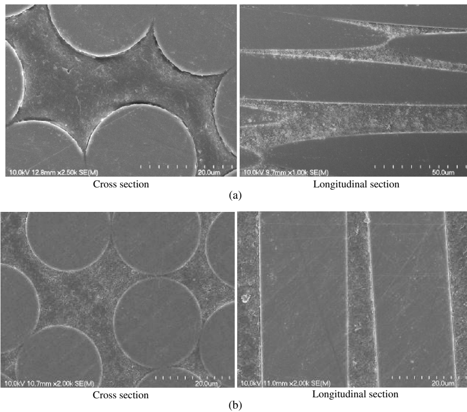
Fig. 10. Micrographs of the fiber/matrix interface of a G/V bar before and after conditioning: (a) before conditioning; (b) after conditioning
