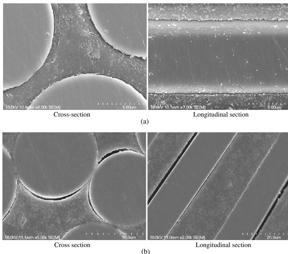
Fig. 9. Micrographs of the fiber/matrix interface of a B/V bar before and after conditioning: (a) before conditioning; (b) after conditioning
