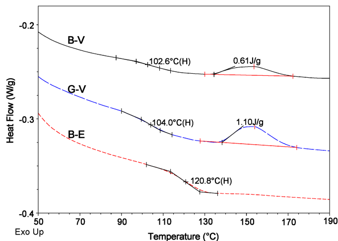
Fig. 3. DSC scans for glass transition temperature ( T_g )
