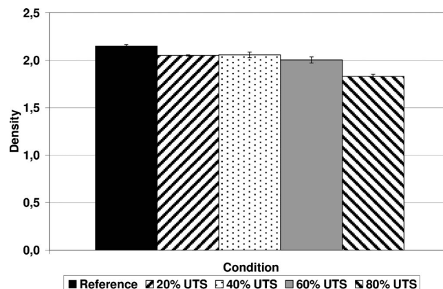
Fig. 4. Measured density of reference and preloaded GFRP bar specimen
