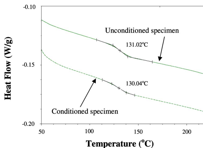
Fig. 8. Thermogram of the second heating run by DSC
