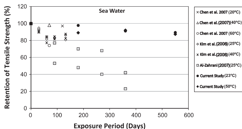
Fig. 7. Retention of tensile strength of GFRP bars exposed to sea water.
