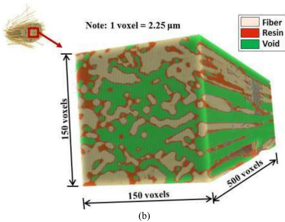
Figure 13. X-ray CT images for FRP specimens exposed to N-SWSSC solution for 63 days: (a) BR; (b) NBT55D63; (c) GR and (d) NGT55D63.
