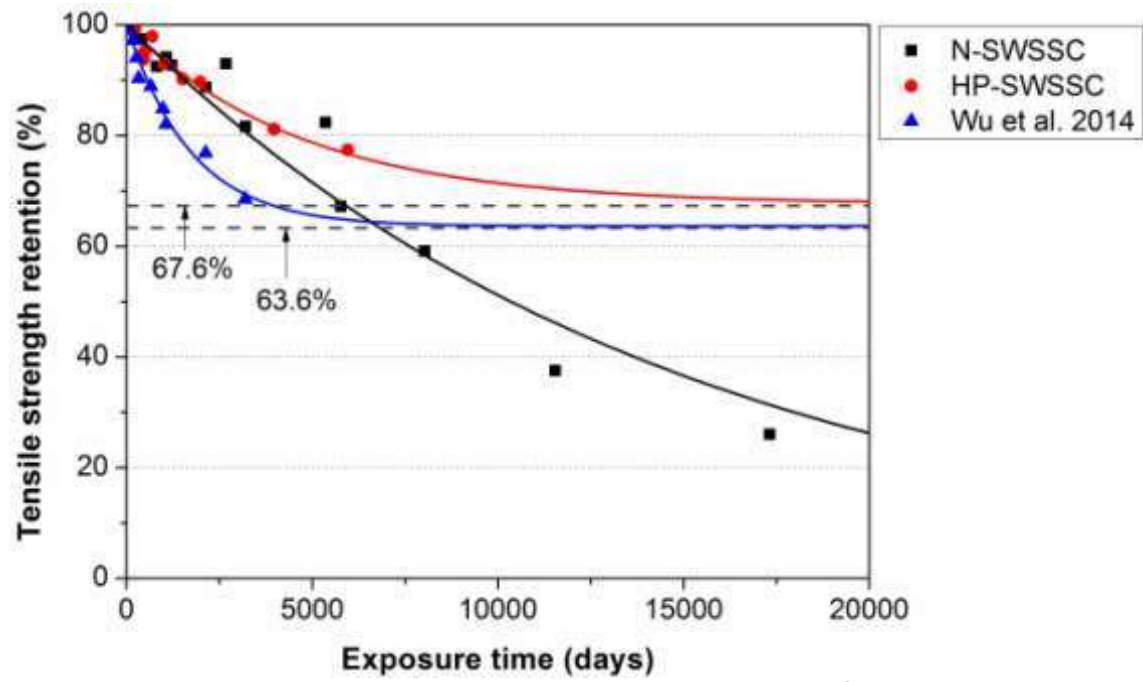
Figure 16. Comparison of predictions for BFRP bars at 9.9°C using Model 3
