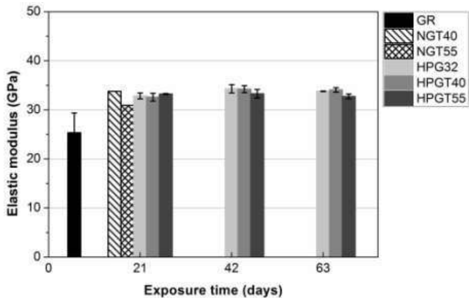
Figure 7. Elastic modulus of conditioned FRP bars in SWSSC solutions: (a) BFRP and (b) GFRP.
