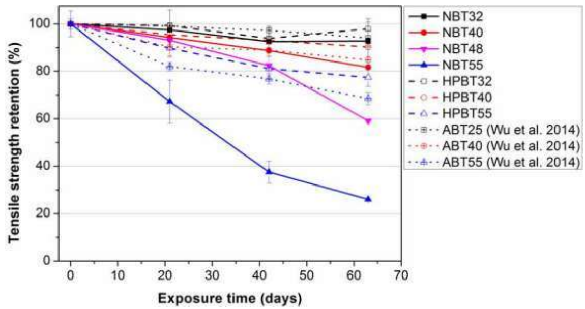
Figure 5. Comparison of tensile strength retention of BFRP bars in SWSSC and alkaline environments at different temperatures.
