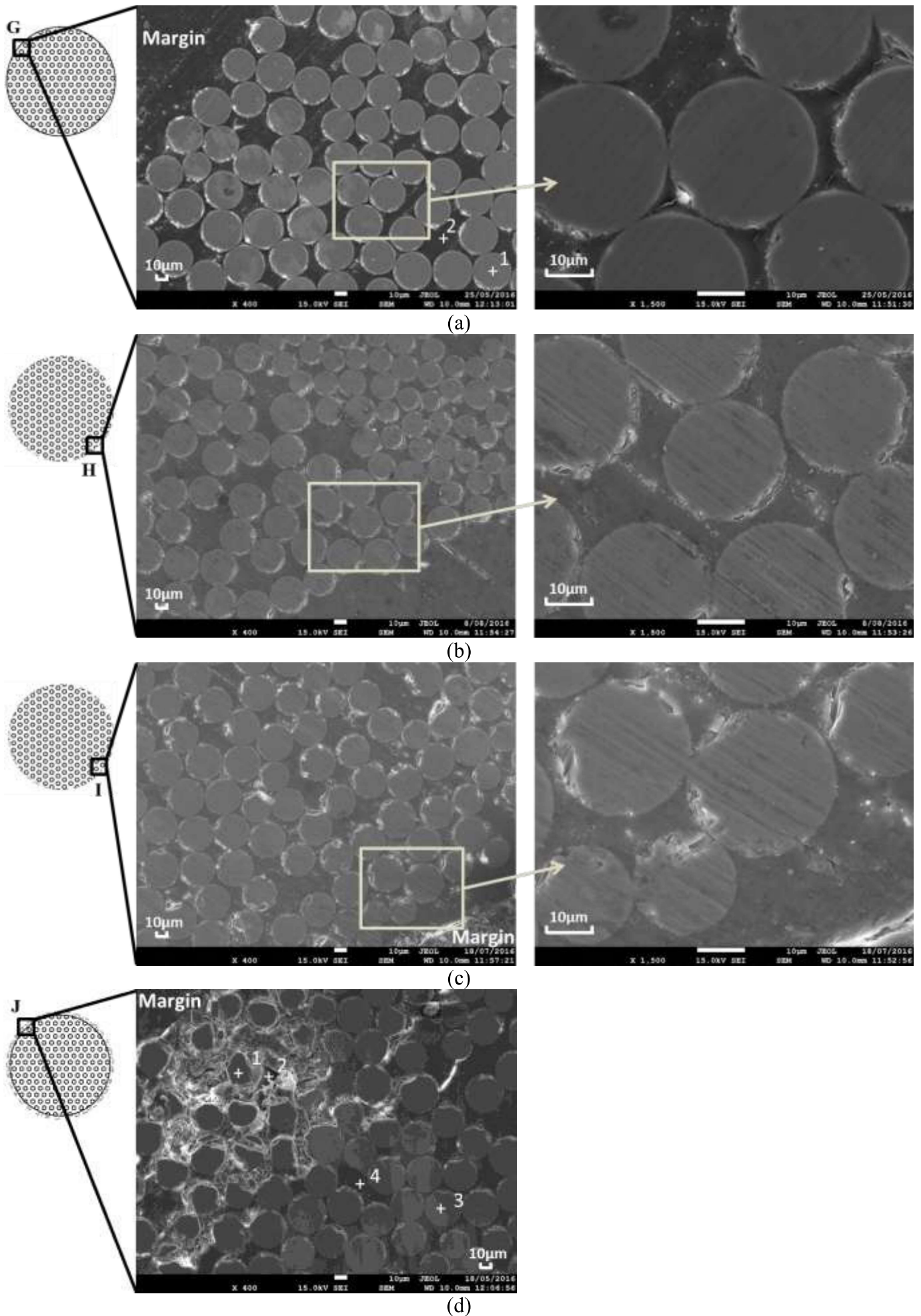
Figure 11. SEM images for GFRP specimens exposed to N-SWSSC solution for 63 days: (a) GR; (b) NGT32D63; (c) NGT40D63 and (d) NGT55D63.
