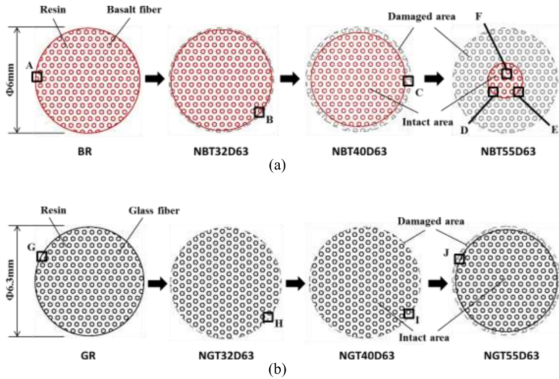
Figure 9. Schematics of evolution of the damage along cross section of the FRP bars after conditioned exposure: (a) BFRP and (b) GFRP.
