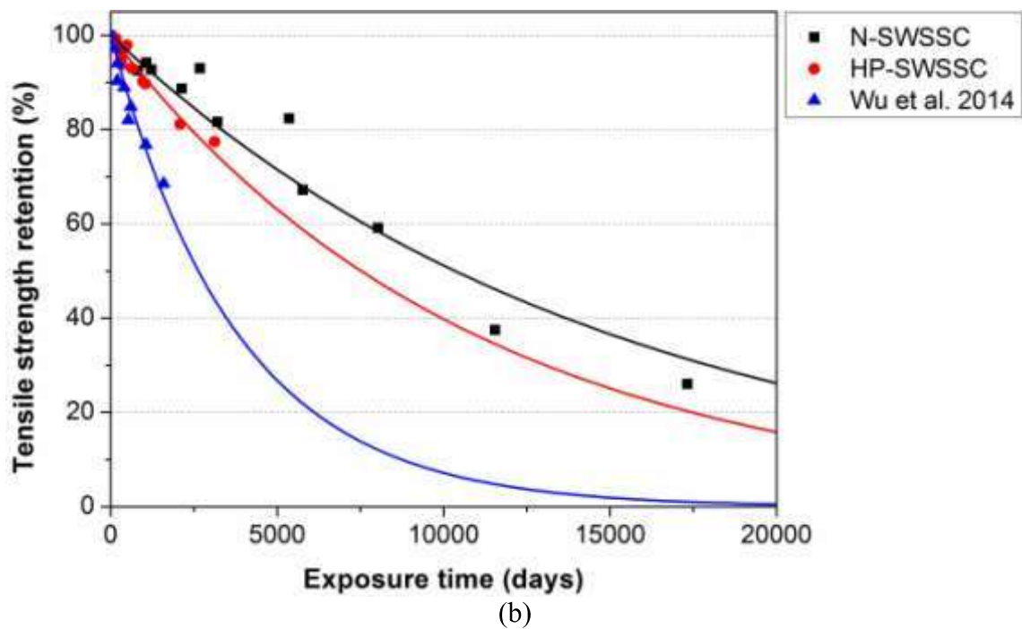
Figure 15. Comparison of predictions for BFRP bars at 9.9°C using Model 2: (a) Arrhenius plots of tensile strength retention and (b) master curves
