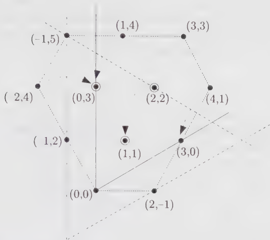
Figure 16.1. The \widehat{\mathfrak{su}}(3)_3 fusion rule [0, 2, 1] \times [0, 1, 2] . Weights are reflected with respect to the lines [-1, \cdot, \cdot], [\cdot, -1, \cdot], [\cdot, \cdot, -1] ; weights sitting on those lines are ignored (circled dots correspond to weights with multiplicity 2).
