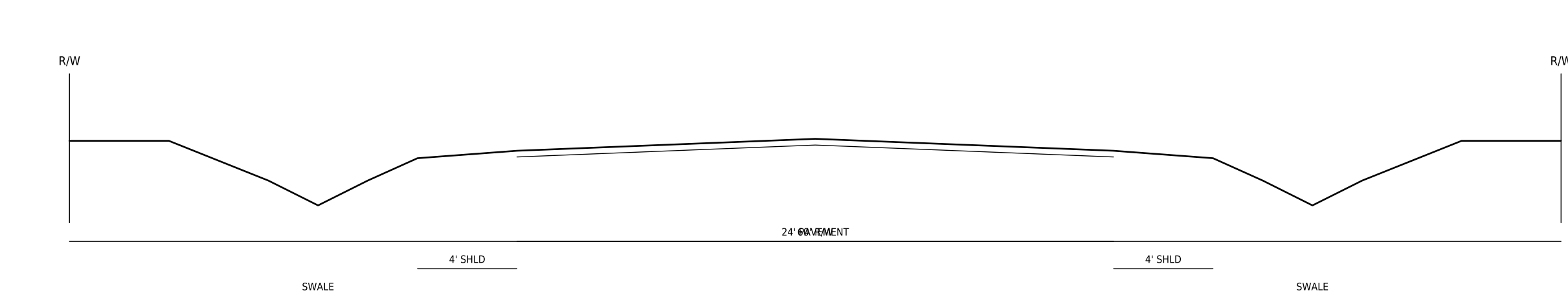
ESTATES COURT — TYPICAL SECTION (RURAL OPEN SECTION, 60' R/W)
