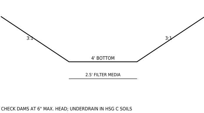
DRY SWALE (M-8) WITH CHECK DAM
