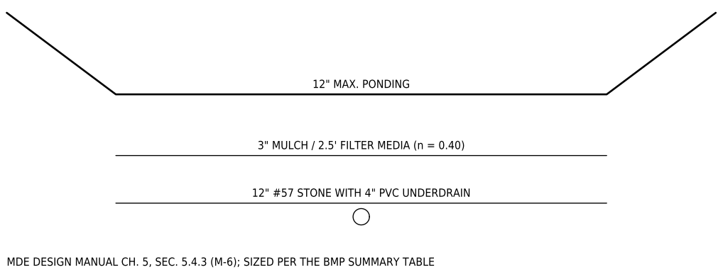
MICRO-BIORETENTION (M-6) — TYPICAL SECTION
