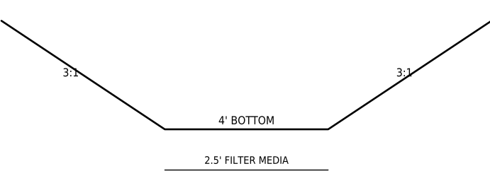
DRY SWALE (M-8) WITH CHECK DAM
