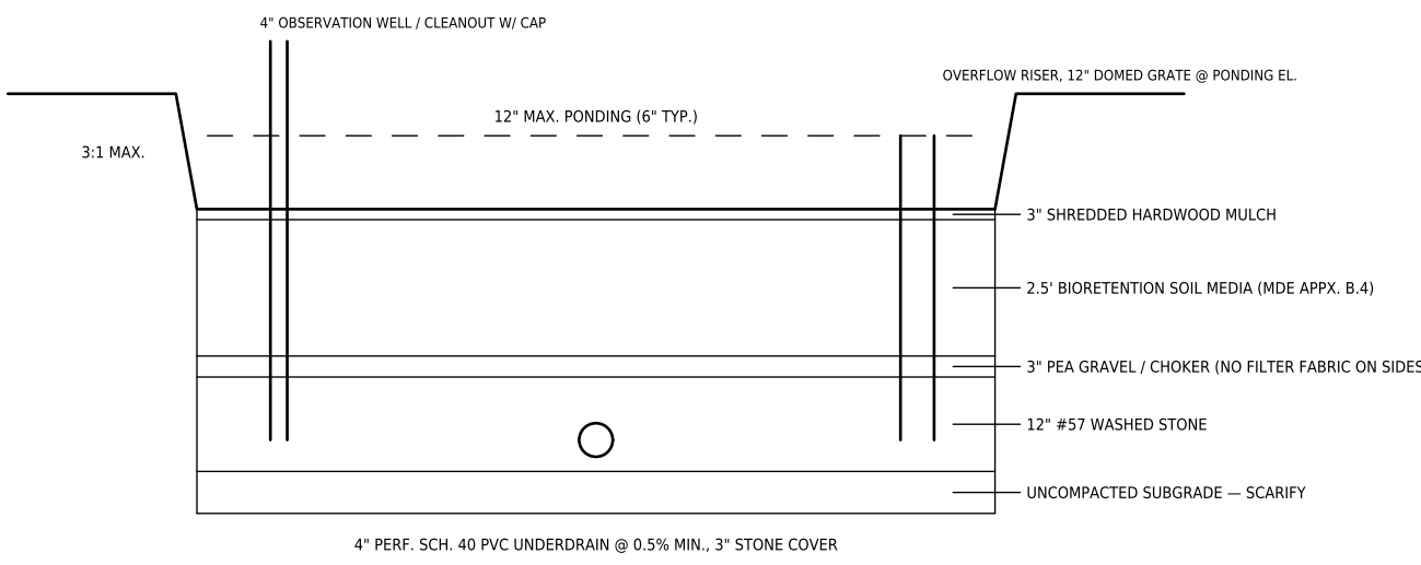
MICRO-BIORETENTION (M-6) — TYPICAL SECTION NTS
