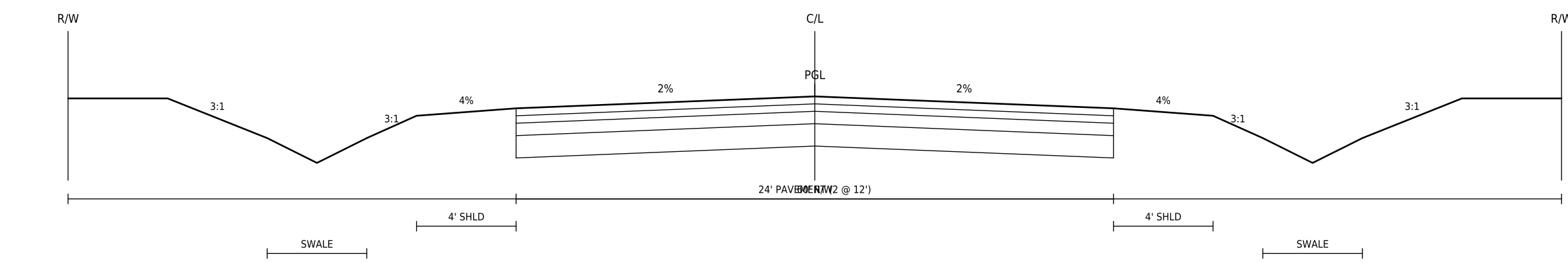
PAVEMENT SECTION — PG DPW&T SPECIFICATIONS AND STANDARDS FOR ROADWAYS AND BRIDGES, SECTION III (RESIDENTIAL)
