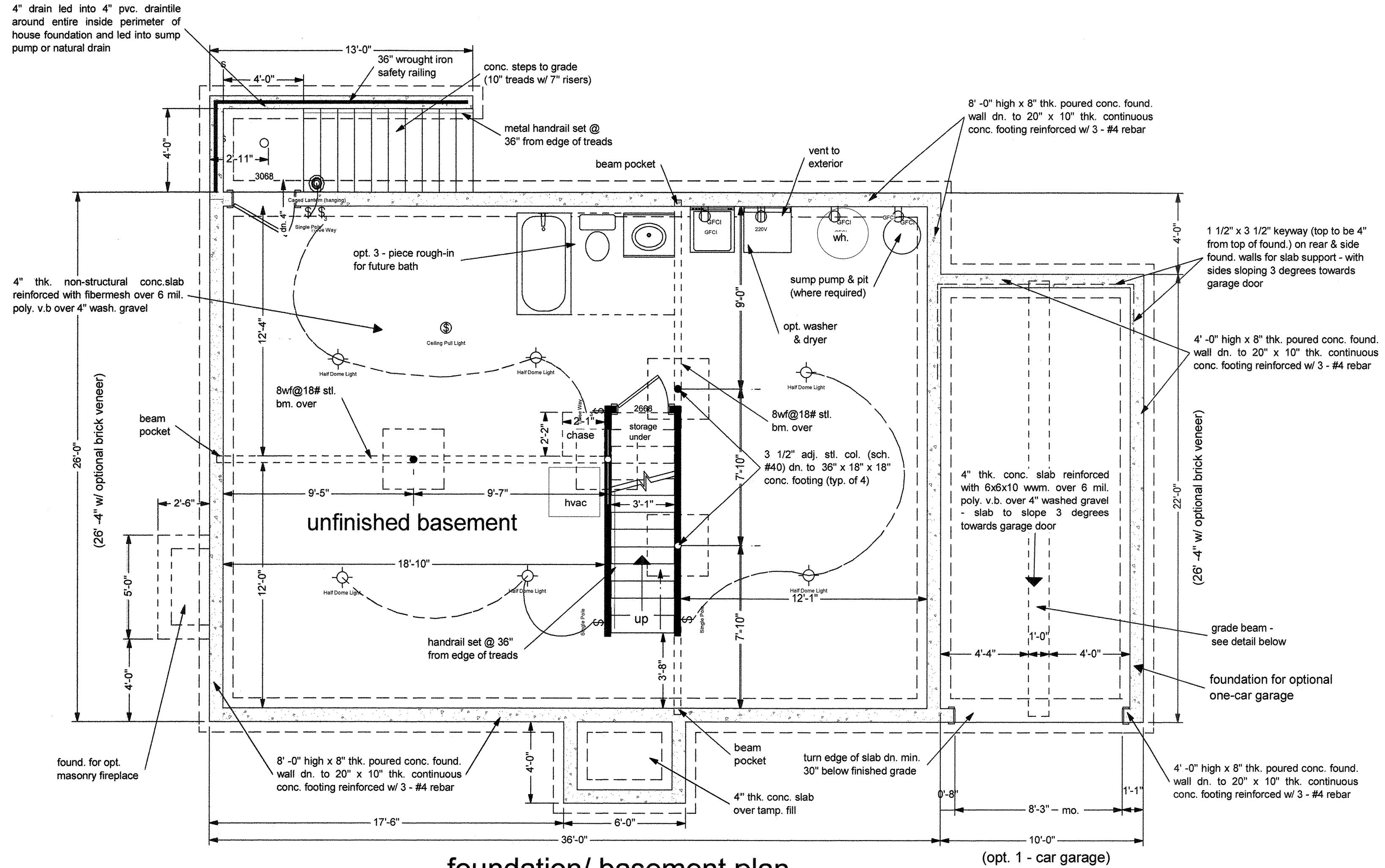
foundation/ basement plan
