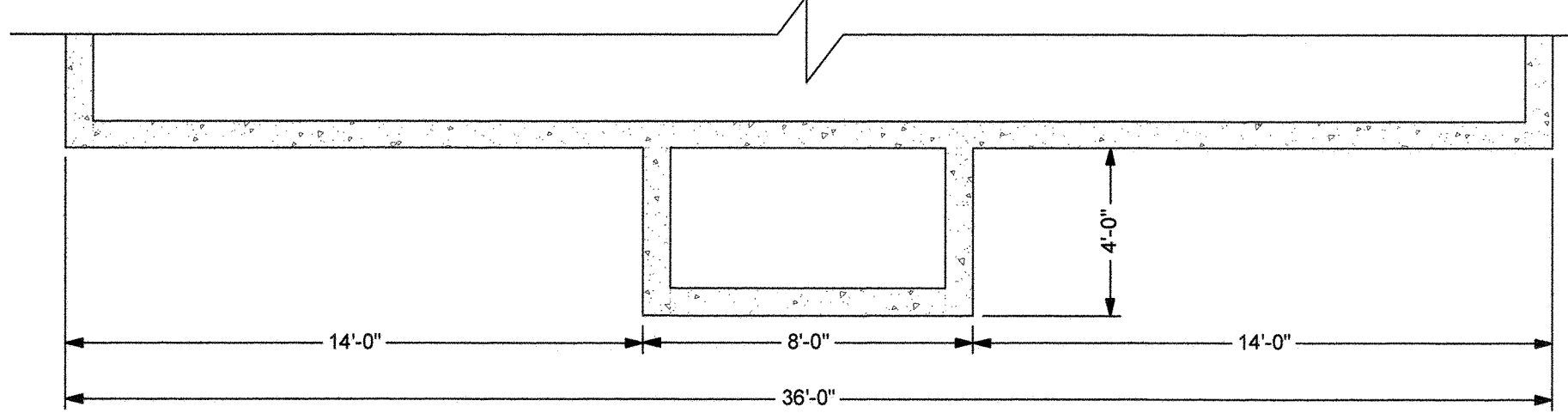
foundation/ basement plan
