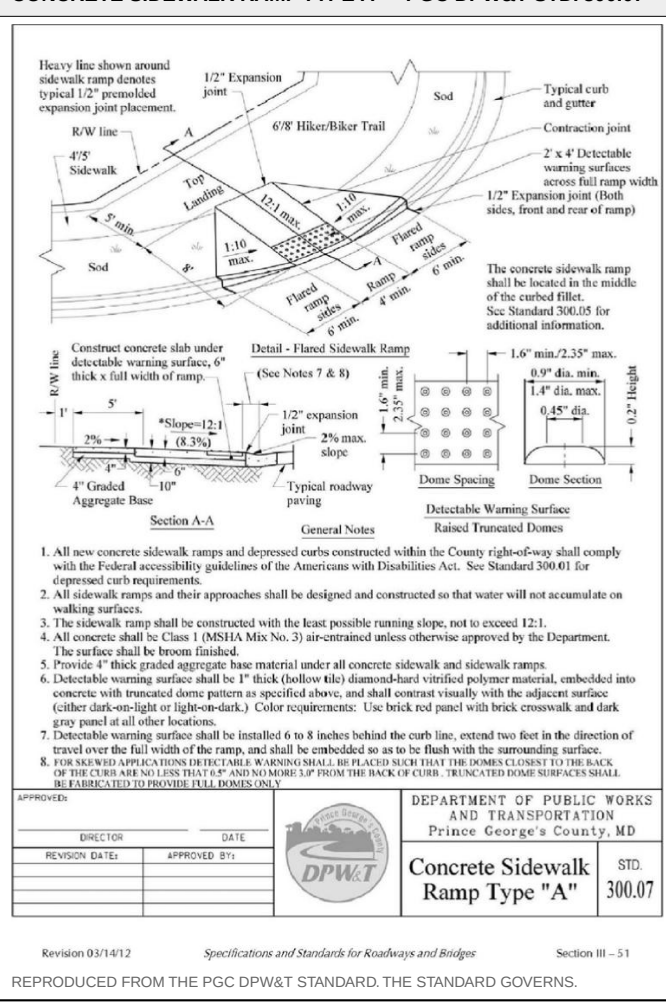
CONCRETE CURB AND GUTTER — PGC DPW&T STD. 300.01 CONCRETE SIDEWALK RAMP TYPE A — PGC DPW&T STD. 300.07
