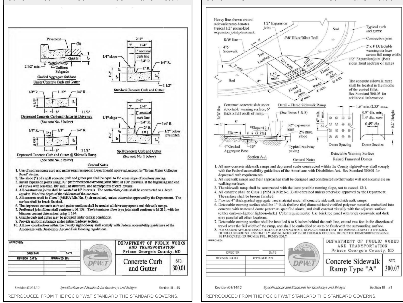
CONCRETE CURB AND GUTTER — PGC DPW&T STD. 300.01 CONCRETE SIDEWALK RAMP TYPE A — PGC DPW&T STD. 300.07
