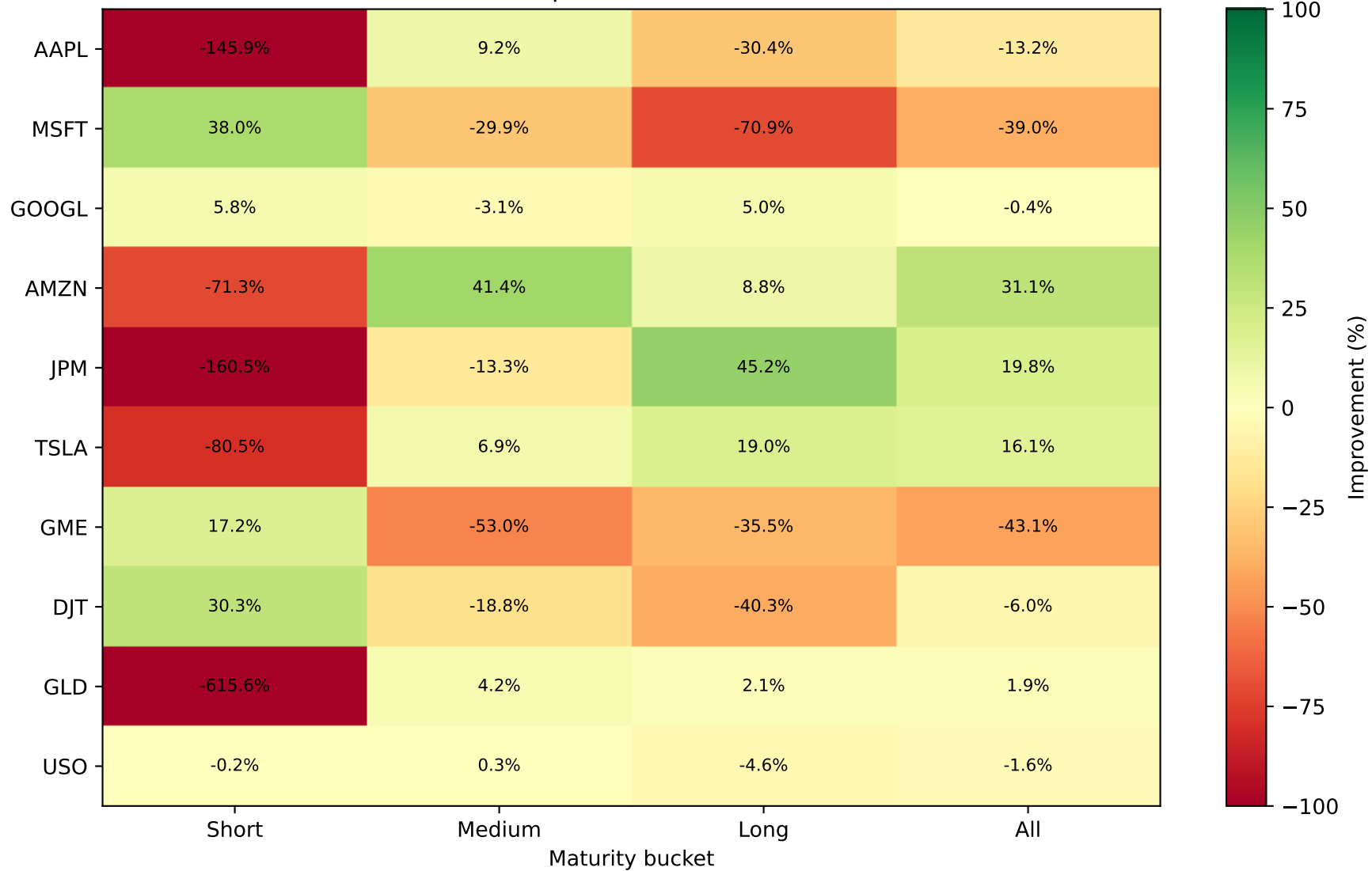
TFBS validation improvement over Black--Scholes
