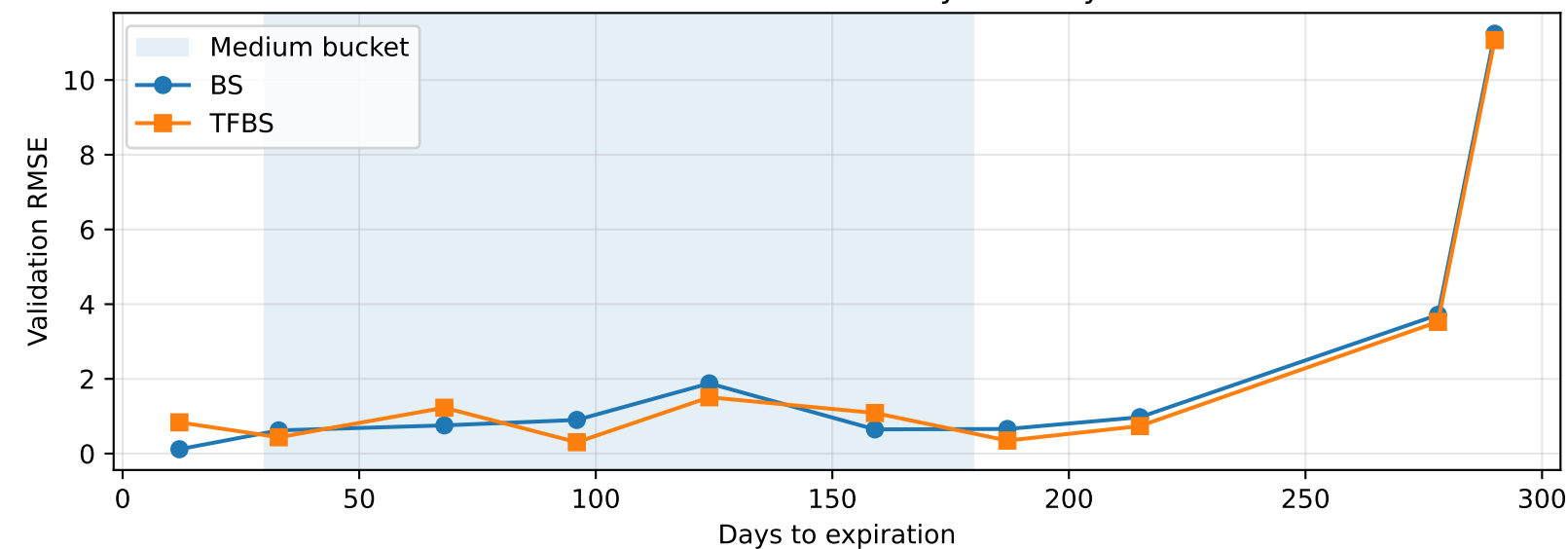
GLD: validation RMSE by maturity
