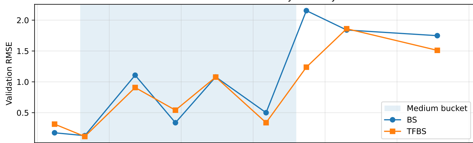
GLD: validation RMSE by maturity
