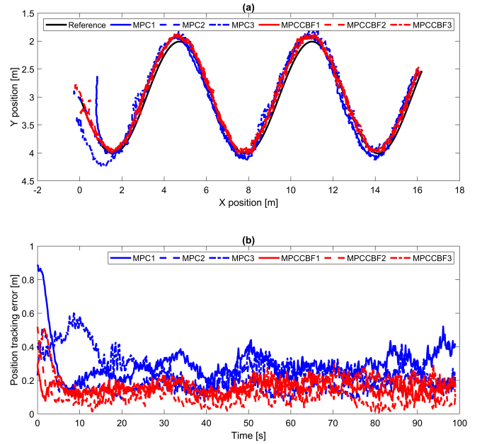
Fig. 6. Tracking performance comparison between MPC and MPC-CBF in Charles River. (a) Position tracking; (b) Position tracking errors.
