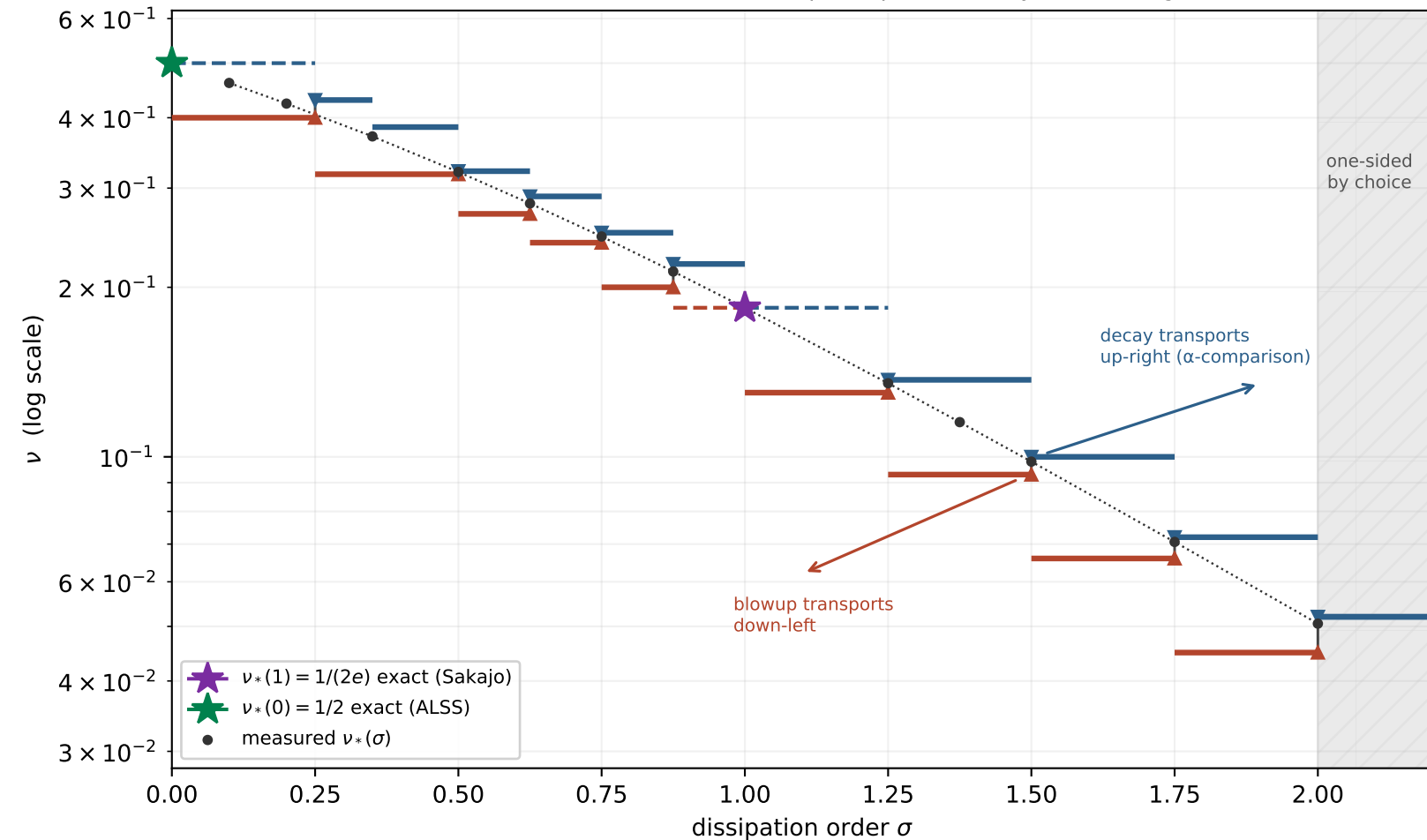
The certified two-sided staircase for \nu_*(\sigma) (ten pinch points; every interior segment \leq 1.603 )
