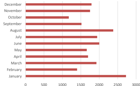
Monthly Rainfall Analysis
