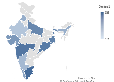
Temperature by State
