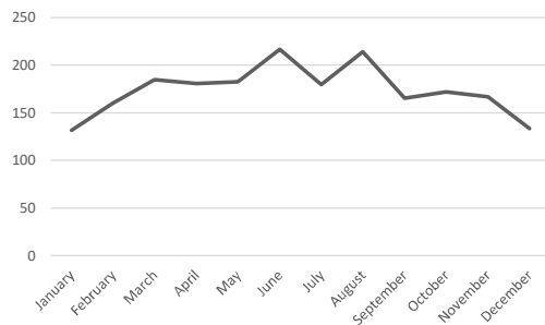
Monthly Rainfall Analysis
