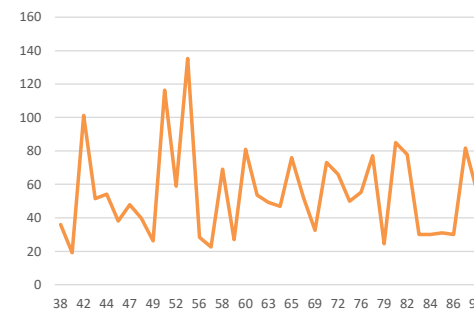
Temperature vs Humidity Analysis
