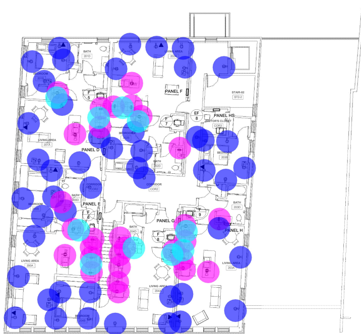
2 SECOND FLOOR POWER PLAN E2.01 1/8" = 1'-0"
