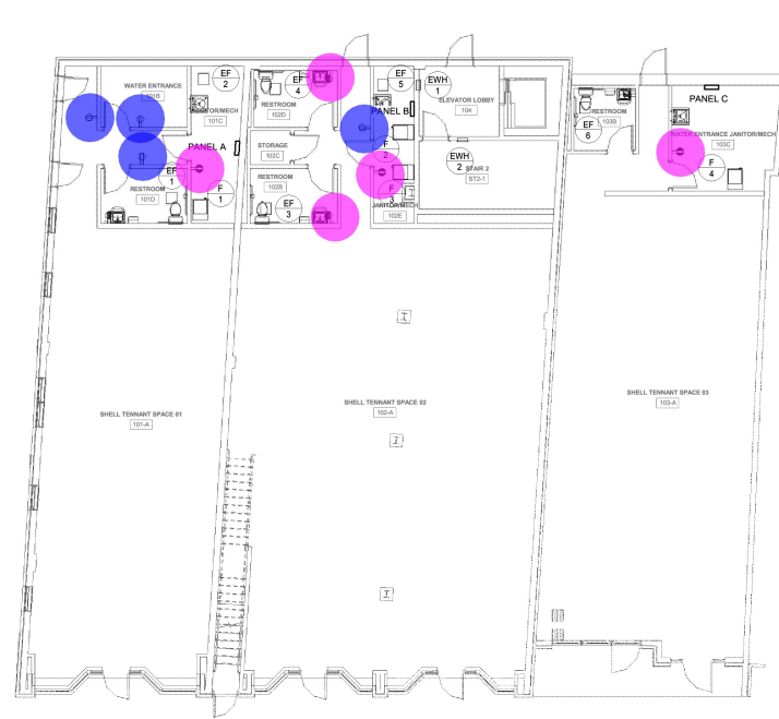
1 FIRST FLOOR POWER PLAN E2.01 1/8" = 1'-0"
