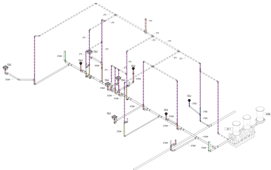
2 SANITARY WASTE AND VENT RISER
