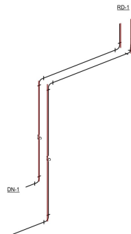
2 PLUMBING RISER DIAGRAM - STORM DRAINAGE SCALE: -
