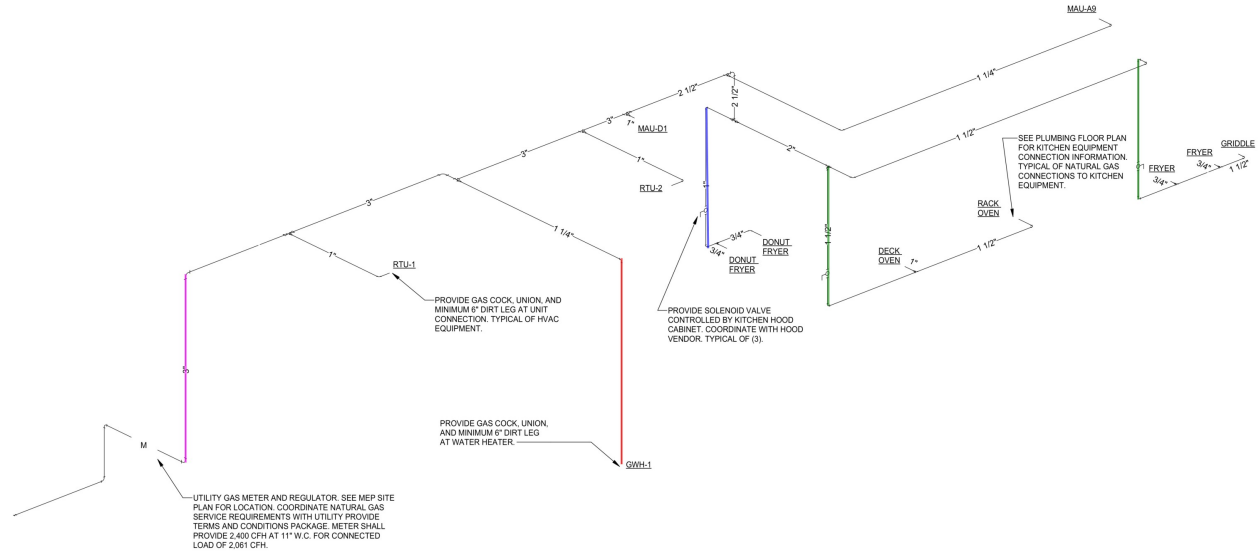
1 PLUMBING RISER DIAGRAM - NATURAL GAS SCALE: -
