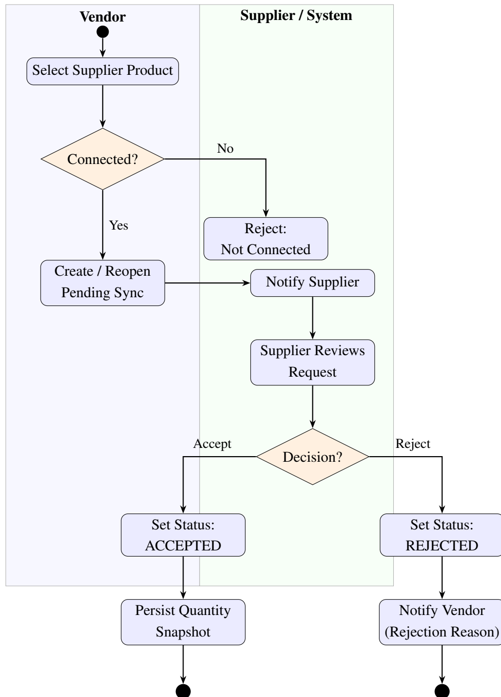
Figure 3.5: Vendor Product Sync Lifecycle Activity Diagram
