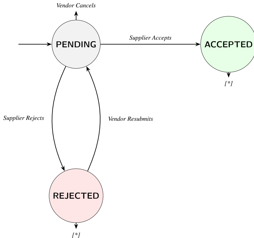
Figure 2.3: Product Sync State Transitions
