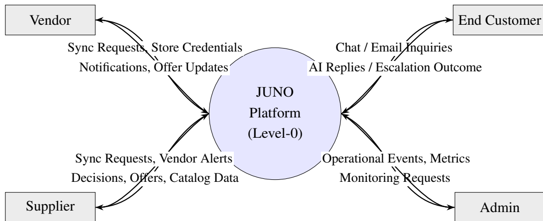
Figure 1.3: Level-0 Data Flow Diagram (DFD)
