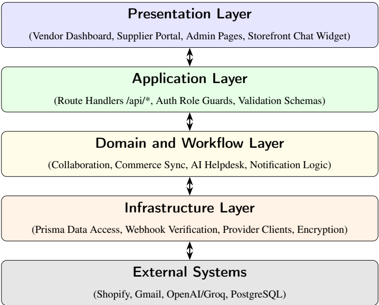
Figure 3.2: Layered Architecture Mapping
