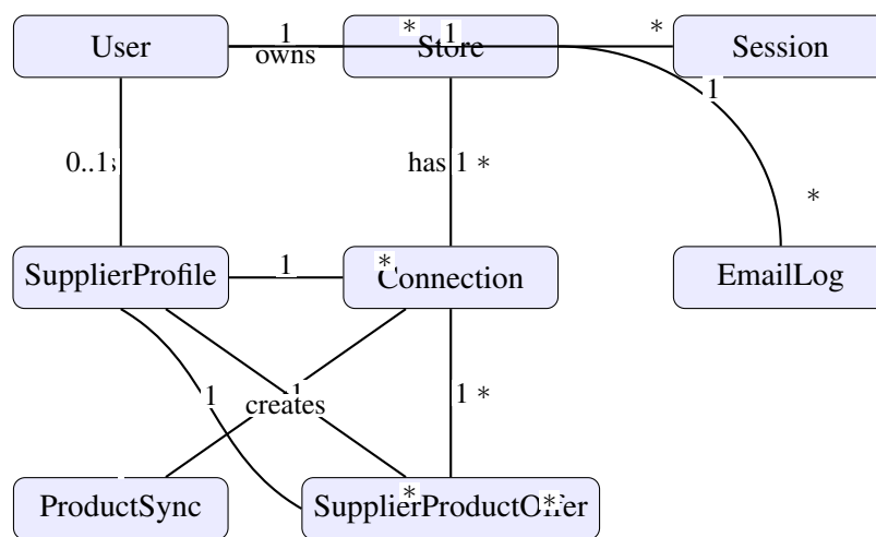
Figure 3.6: Conceptual Domain ER Diagram
