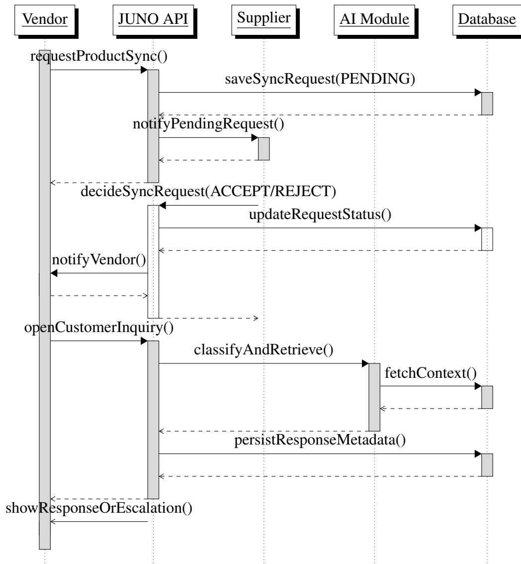
Figure 1.2: Core Sequence Flow Diagram
