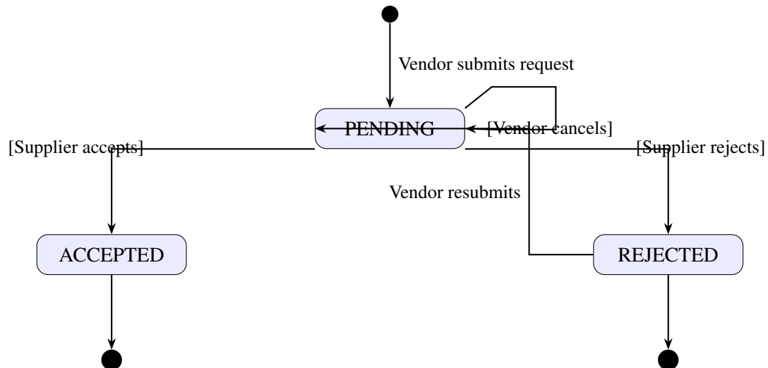
Figure 2.4: Product Sync State Transitions
