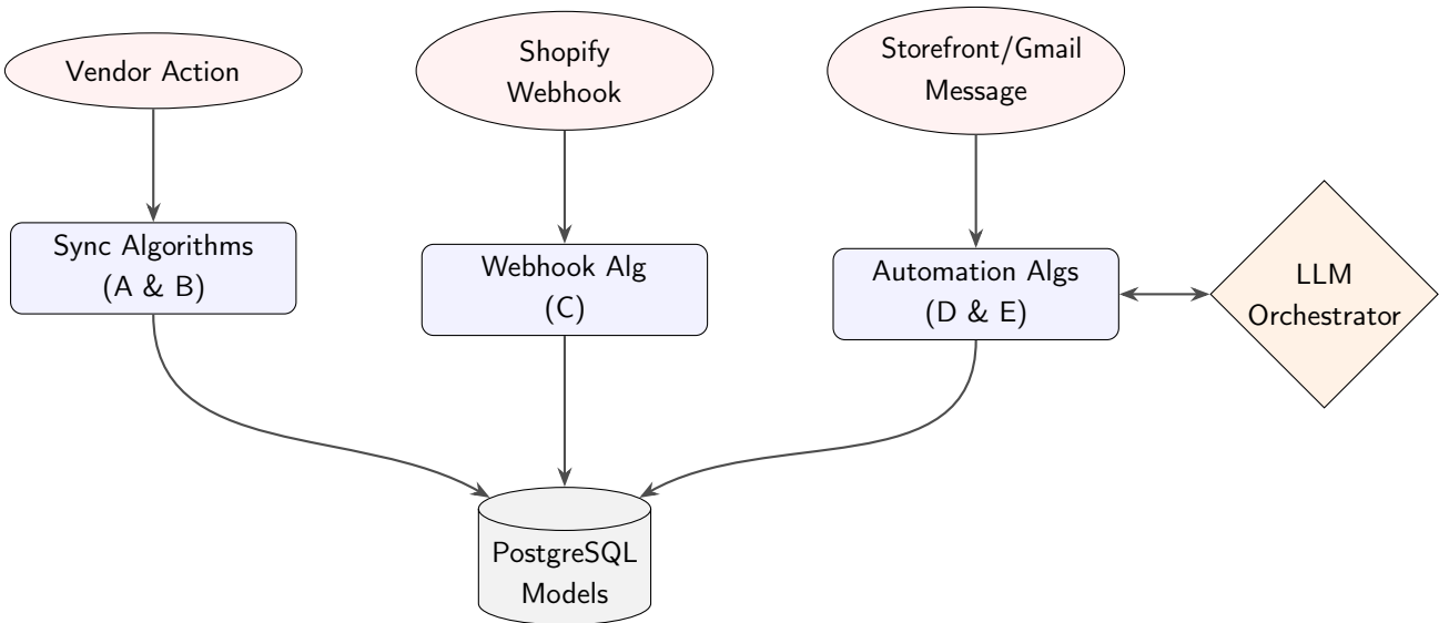
Figure 4.1: Interaction between System Events and Implementation Algorithms
