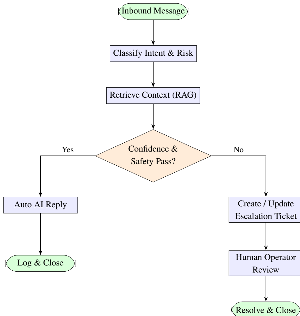
Figure 2.2: Support Escalation Process Flow
